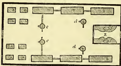
Plan of an oil of vitriol manufactory.
