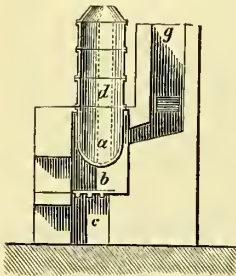
Refining Furnace.
