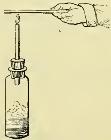
Simple mode of applying Marsh's Test.
