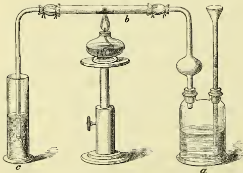
Apparatus for reducing tersulphuret of antimony.
