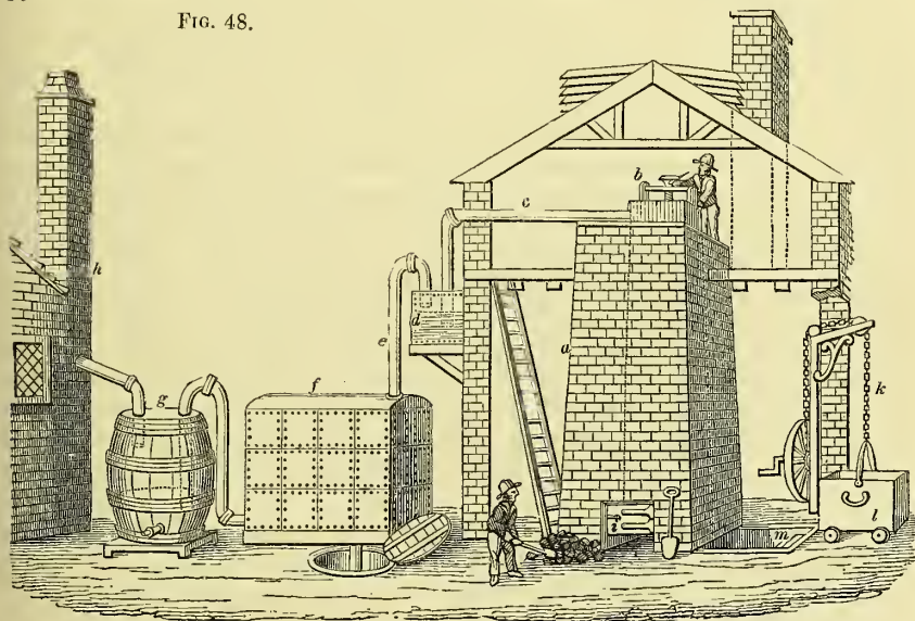
Manufactory of Animal Charcoal.
