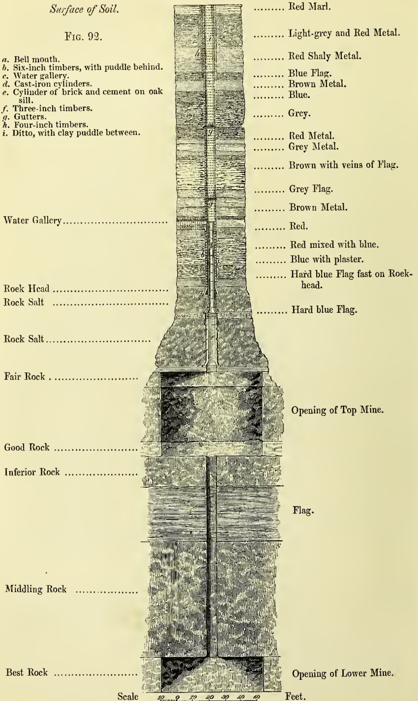
Section of the Wharton Salt Mine, on the River Weaver, Cheshire.
