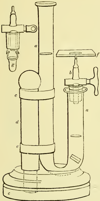
Marsh's Apparatus.
