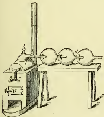
Iodine leaden still and glass receiver.
