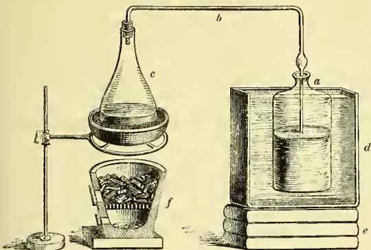
Hydrochloric Acid Apparatus.
