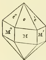
Common bipyramidal crystal with short intervening prism.
