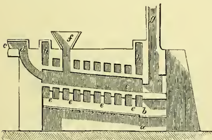
Section of the Roasting Furnace.
