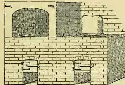
Furnaces for the preparation of Corrosive Sublimate.
