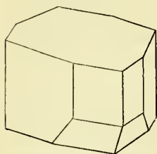
Acute Oblique Rhombic Prism of Realgar.
