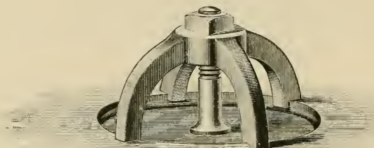
FIG. 2. — ILLUSTRATING THE FOUR-LEGGED FORM.
