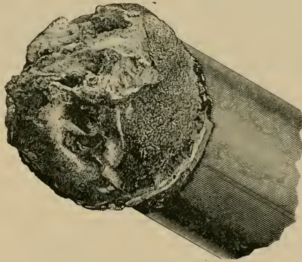
FIG. 1.—A FEED-PIPE NEARLY SEALED UP BY SCALE.
