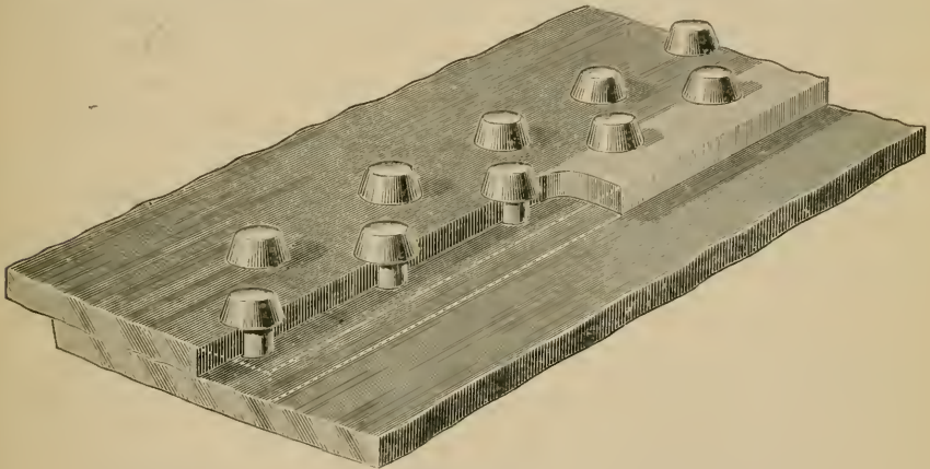
A FAULTY JOINT, AS "PREPARED" TO PASS INSPECTION.
