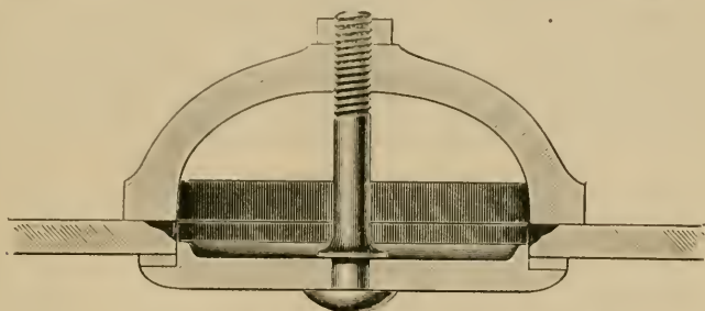
FIG. 4. — ILLUSTRATING THE EFFECTS OF THE RING-GUARD.
