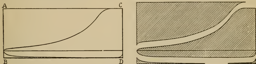
FIGS. 6 AND 7.—INDICATOR CARDS: FINDING AREA AND AVERAGE PRESSURE.
