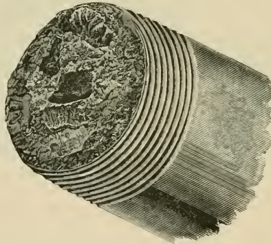
FIG. 3.—A FEED-PIPE CHOKED WITH A STONE-LIKE SCALE.
