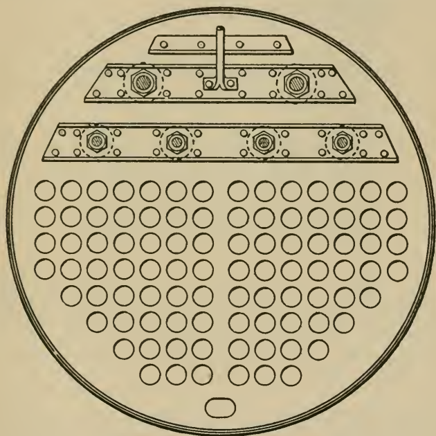
FIG. 1. — A BOILER HEAD WITH THROUGH BRACES.
