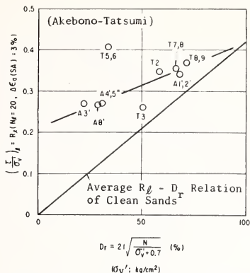
Fig. 26 D_r - R_{\ell} Relationship of Sands of Akebono-Tatsumi Site
