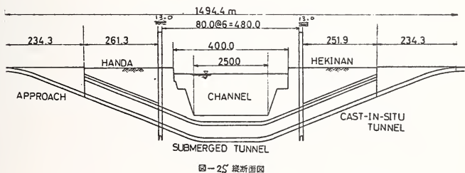
Fig. 2S Longitudinal Section of Tunnel
