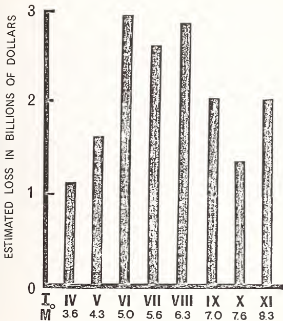
Figure 2.--Estimated dollar losses to wood frame dwellings in California as a function of maximum Modified Mercalli intensity ( I_M ) and equivalent mean magnitude (M). Historical earthquakes in California for the period 1801-1967 were used as the seismicity input. The spatial distribution of dwellings and their characteristics were assumed constant at the 1967 level for the loss simulation study. (Adapted from Reference 6).
