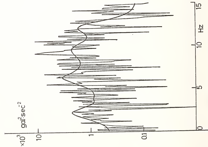
Fig. 10 Power Spectrum (synthesized U-D)
