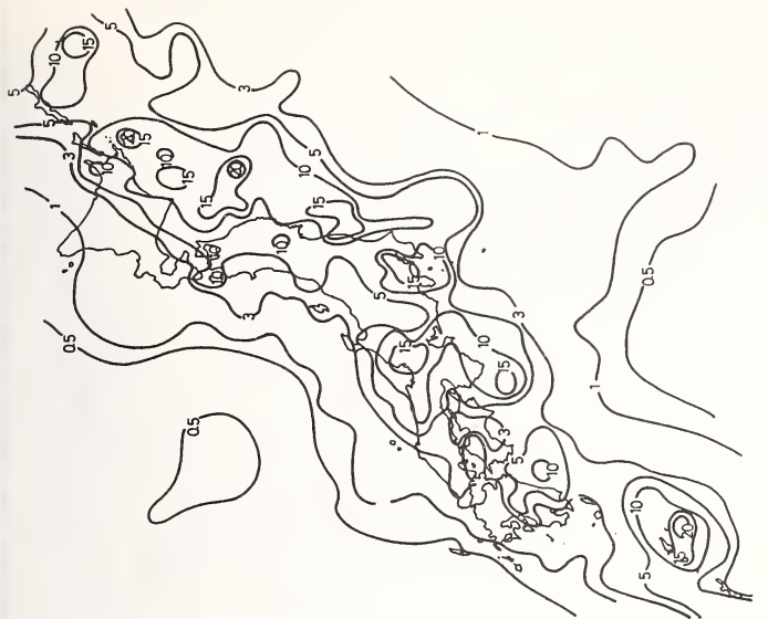
Fig. 12. Regional Distribution of the Expected Velocity Values (cm/sec) at the Base Rock ( \tau=100 years)
