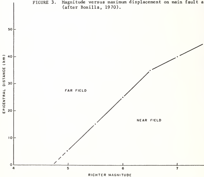
FIGURE 4. Near field and far field limits (after Krinitzky and Chang, 1975)
