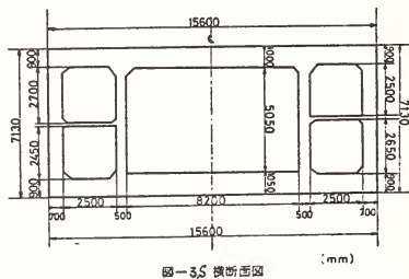
Fig. 3S Typical Cross Section
