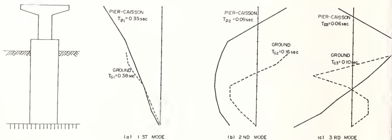
Fig. 4-10 VIBRATION MODES OF PIER-CAISSON AND GROUND
