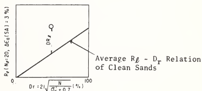
Fig. 27 Definition of DR_{\ell}
