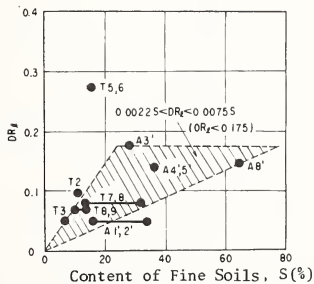
Fig. 28 : S - D R_{\ell} Relationship
