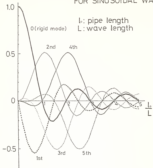
Fig. 4 Participation Factor of a Finite Length Pipe
