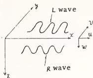
Fig. 2 Modes of Rayleigh and Love waves
