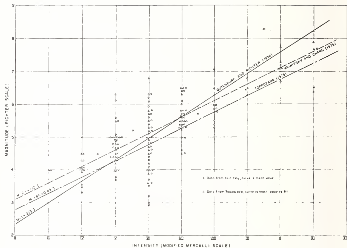
FIGURE 1. Comparisons of several curves relating magnitude and intensity values in the western United States (Gutenberg and Richter curve from Krinitsky and Chang, 1975).
