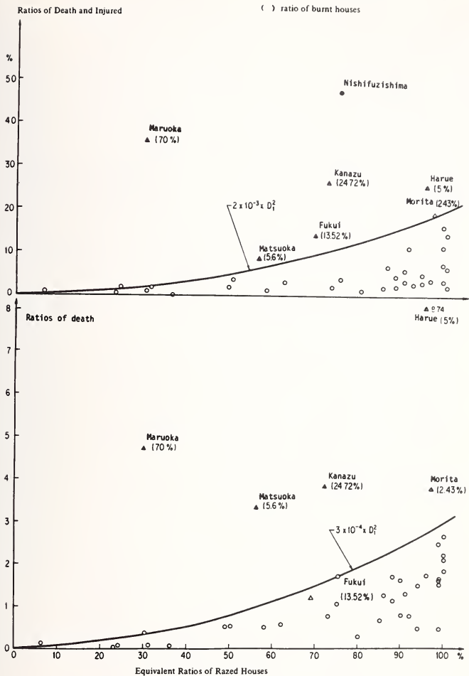
Fig. 2 Relationships between Equivalent Ratio of Razed Houses and Losses of Lives in Fukui Earthquake 3)
