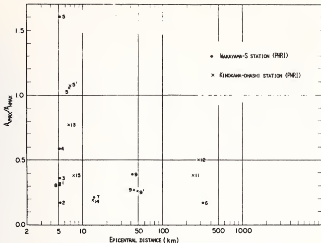
Fig. 9 Ratios of max. vertical acceleration to max. horizontal acceleration ( A_{vmax}/A_{hmax} ) at Wakayama-z-i-S station
