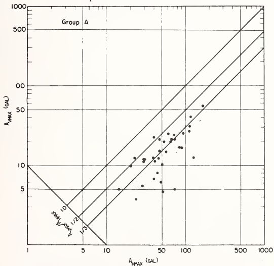
Fig. 6 Relationship between max. vertical acceleration ( A_{vmax} ) and max. horizontal acceleration ( A_{hmax} ), for Group A
