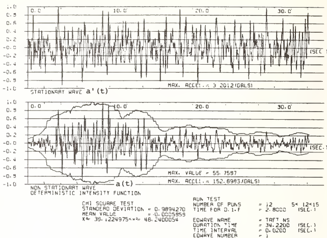
Fig.-6a Deterministic Intensity Function (Horizontal Components)
