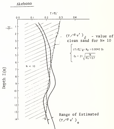
Fig. 30 Comparison of (\tau/\sigma'v)_l of Clean Sand for N = 10 with (\tau/\sigma'v)_e
