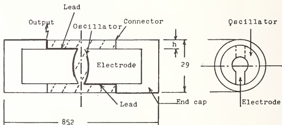
Figure 5-1. Tsunami-meter Sensor
