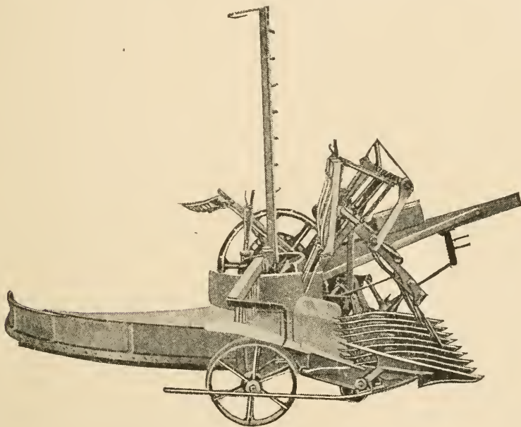
SPECIAL PEA VINE HARVESTER.
