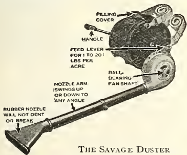
THE SAVAGE DUSTER
