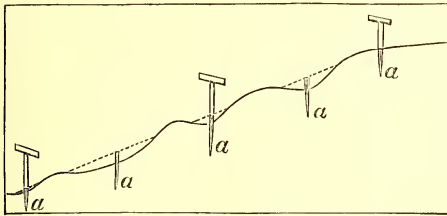
Fig. 37. LEVELLING.—OBTAINING UNIFORM SLOPE. (See text.)
