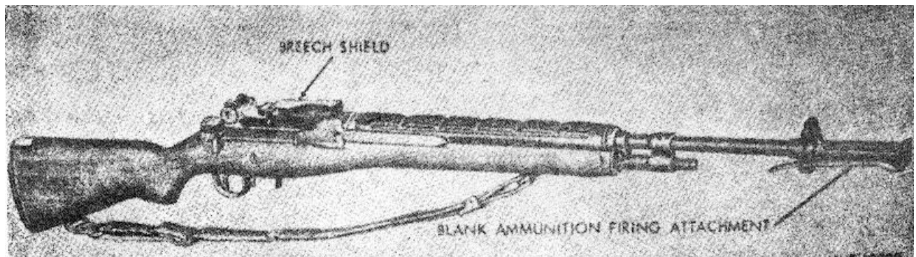
Figure 1-6. 7.62-MM Rifle ,M14 and blank ammunition firing attachment and breach shield.
