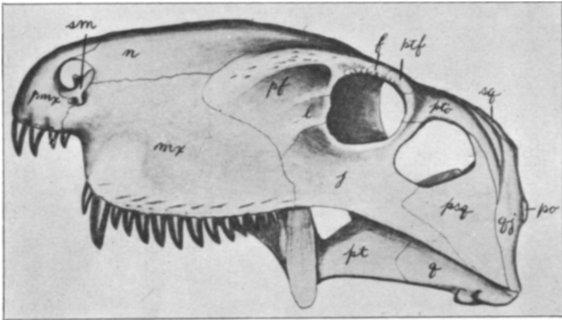
FIG. 2.—Restoration of the left side of the skull of D. gigas . bo , basi-occipital; bs , basi-sphenoid; j , frontal; j , jugal; l , lachrymal; mx , maxillary; n , nasal; pmx , premaxillary; pv , prevomer; pt' , ascending plate of pterygoid; pt , pterygoid; pl , prefrontal; plj , postfrontal; pto , postorbital; pa , parasphenoid; psq , prosquamosal; ps , ethmoid; po , paroccipital (opisthotic); q , quadrate; sq , squamosal; st , stapes.
