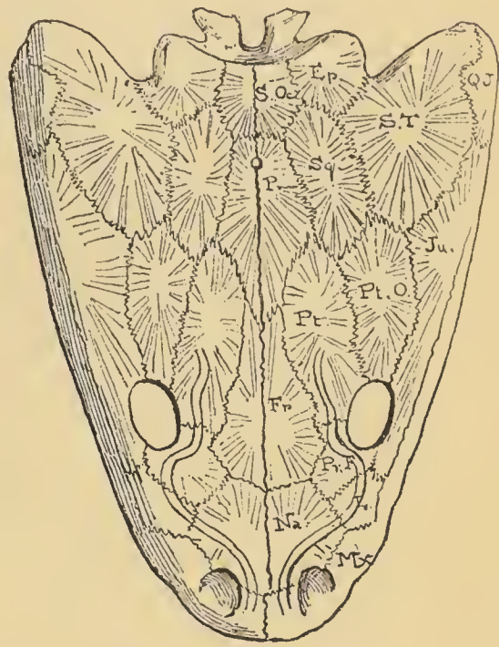
FIG. 87.—Frontal aspect of the cranium of Metoposaurus diagnosticus (Meyer), Upper Trias, near Stuttgart. Letters as in Fig. 84. ( \frac{1}{3} nat. size.)
