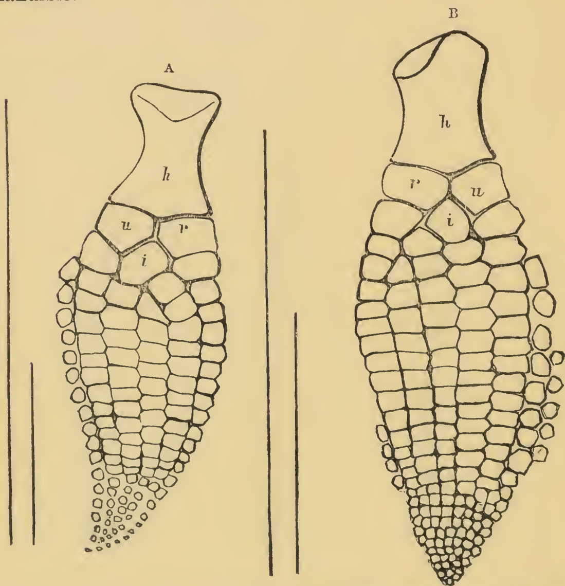
FIG. 45.—(A) Ventral aspect of the left pectoral limb of Ichthyosaurus Conybeari , (Lydekker), Lower Lias, Lyme Regis ( \frac{1}{2} nat. size). h , humerus; r , radius; u , ulna; i , intermedium. The vertical lines show the relative lengths of the limb and the skull, the longer line being that of the skull. The notches in the anterior border of the first row of phalangeals are omitted. (B) Dorsal aspect of the left pectoral limb of Ichthyosaurus communis , (Conybeare), Lower Lias, Lyme Regis. The letters and lines are the same as in Fig. A.
