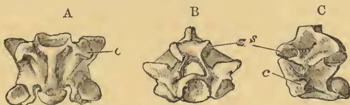
FIG. 30.—(A) Hæmal, (B) Anterior, (C) left lateral views of a trunk-vertebra of Paleryx rhombifer (Owen), from the Eocene Phosphorites of Caylux, France. c, costal articulation; z, s, zygosphenes.
