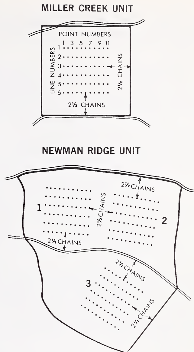
Figure 6.—Plot layout and sampling point locations on typical units.
