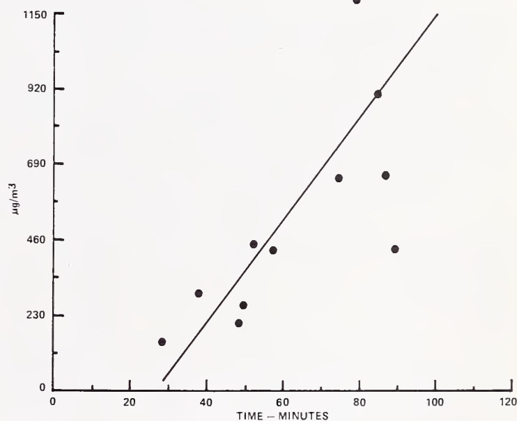
Figure 13.—Particulate concentration over time in the smoke plume from unit S-2 at Newman.
