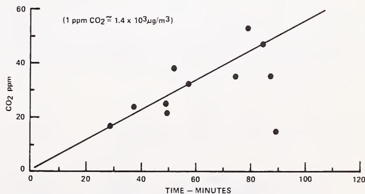
Figure 14.—Carbon dioxide concentration in the smoke plume from unit S-2 at Newman.
