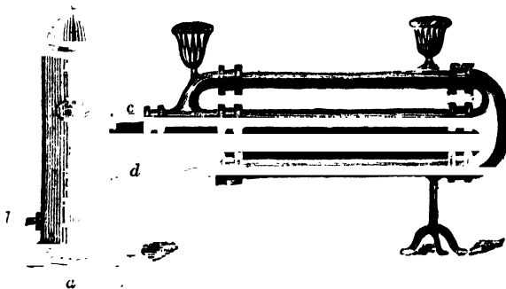
FIG. 178. WRIGHT AND CO.'S GAS BOILER.
