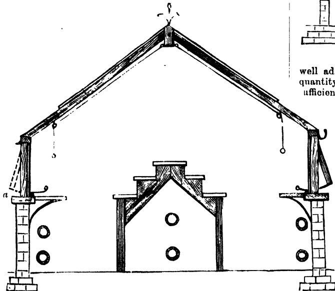
FIG. 148. SECTION OF SPAN-ROOF PLANT HOUSE.
