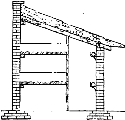
FIG. 619. SECTION OF LEAN-TO MUSHROOM HOUSE.
