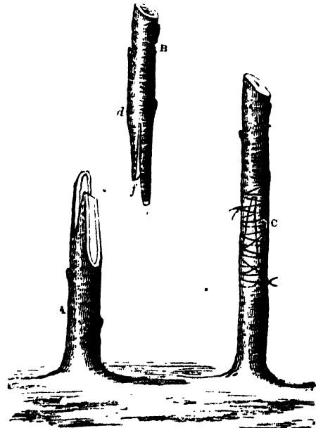
FIG. 136. WHIP OR TONGUE-GRAFTING.
