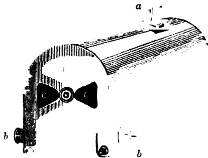
FIG. 174. CRUCIFORM SADDLE BOILER.
