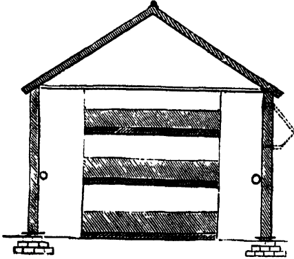
FIG. 618. SECTION OF SPAN-ROOFED MUSHROOM HOUSE.
