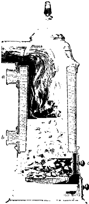
FIG. 177. UPRIGHT CYLINDER BOILER. VERTICAL SECTION.
