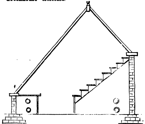
FIG. 150. HIP-ROOFED GREENHOUSE.
