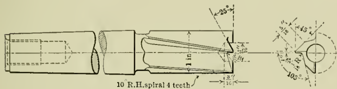
Fig. 3—New Design of End Mill with Four Teeth.
