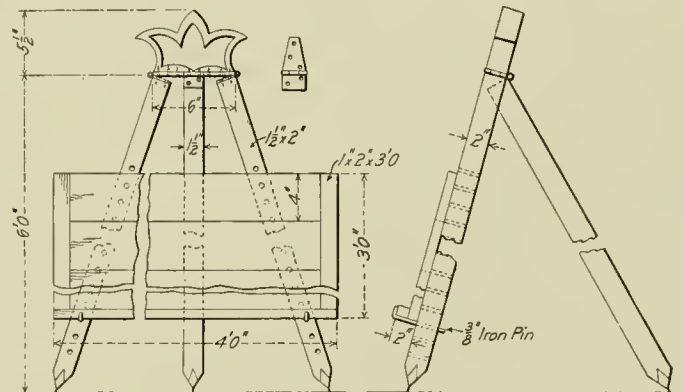
Fig. 2—Paint Shop Easel.
