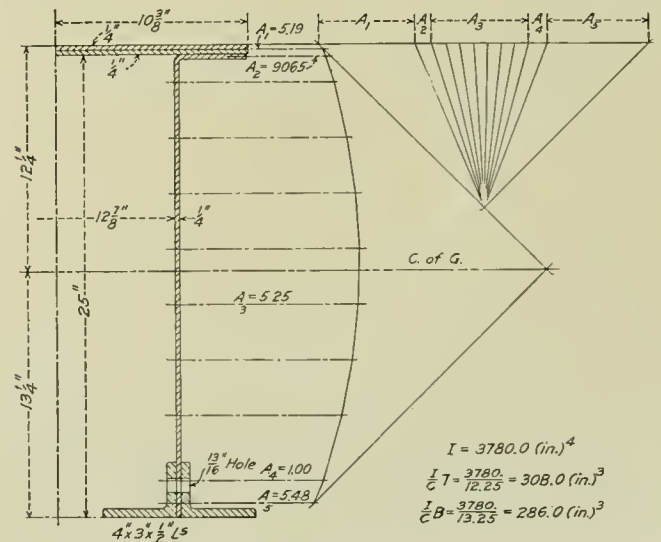
Fig. 10—Center Girder Section at N , Fig. 2.
