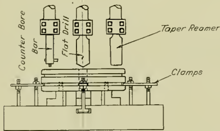
Piston Heads. Operations No. 4, 5 & 6.
