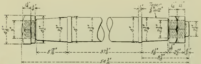
Standard Piston Rod.—Central of Georgia.
