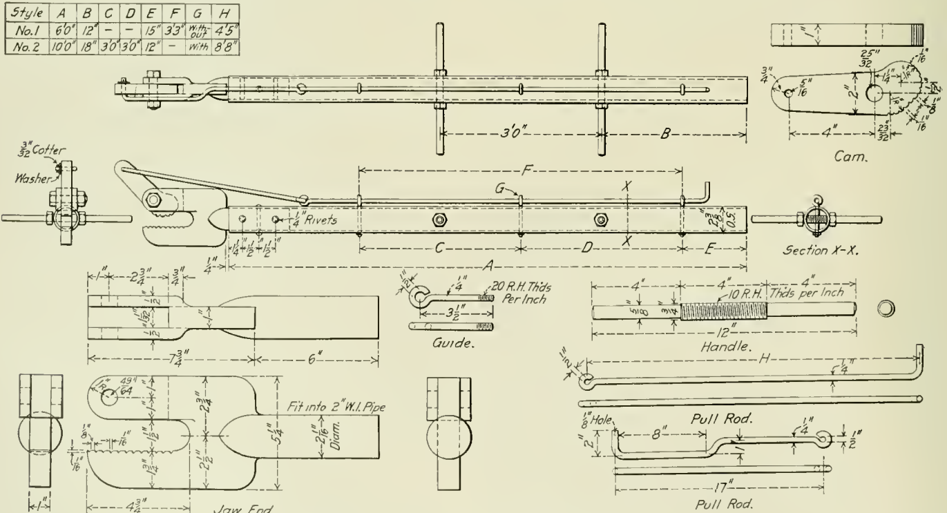
Fig. 1—Tongs for Handling Hot Steel Plates.
