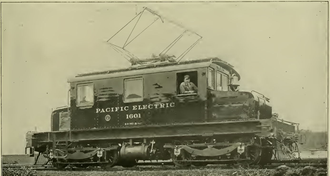
Electric Locomotive for the Southern Pacific.
