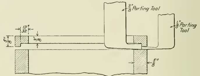
Parting Tools for Piston Valve Packing Ring.
