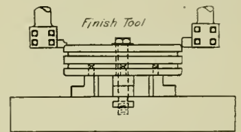
Piston Heads Operation No. 3.
