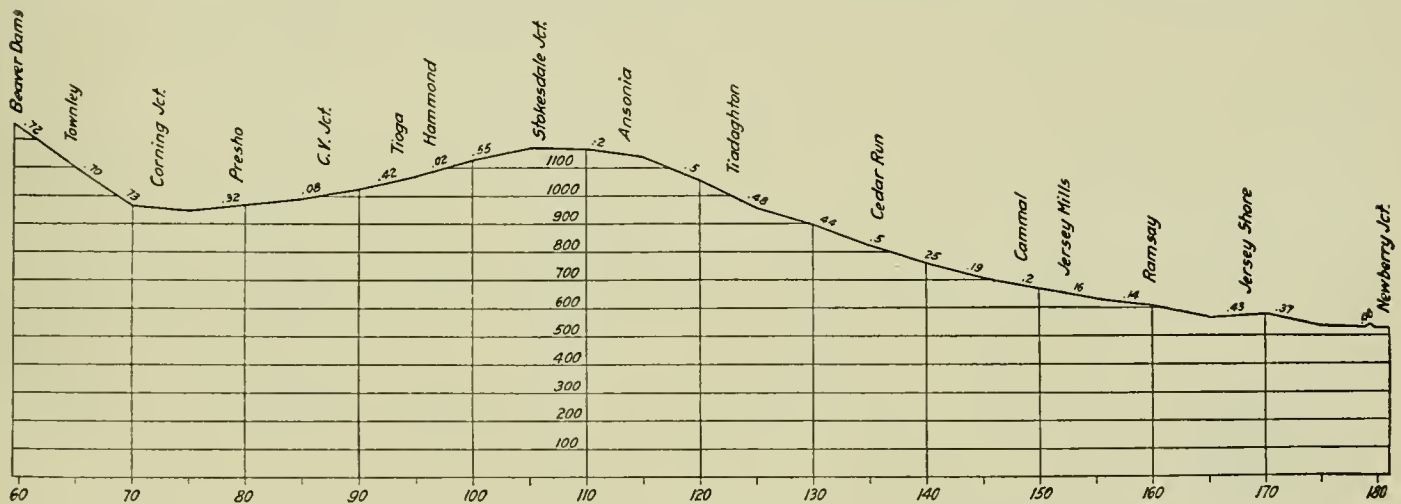
Fig. 1—Profile of Pennsylvania Division of the New York Central & Hudson River Between Jersey Shore and Corning.
