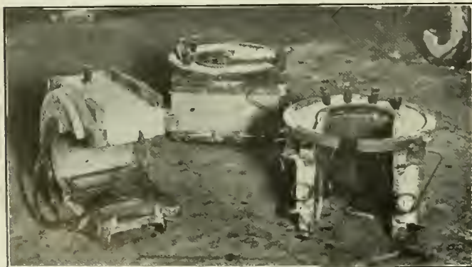
Fig. 7—Boxes After Hub Face and Shoe and Wedge Liners Have Been Poured.
