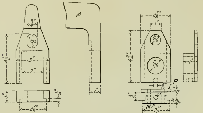
Fig. 4—Details of Spindle Support Block.
