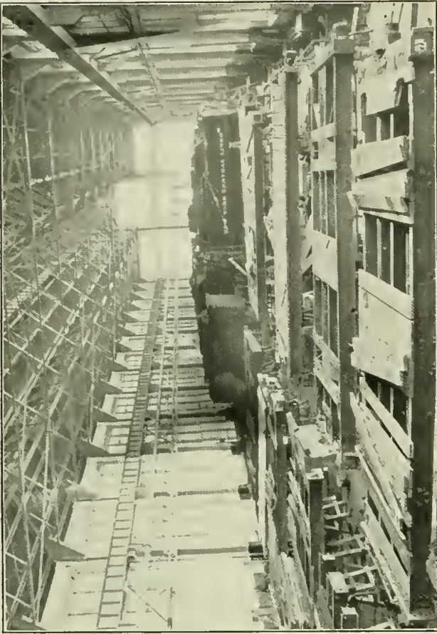
General View of the Tank Shop; Beech Grove Shops.
