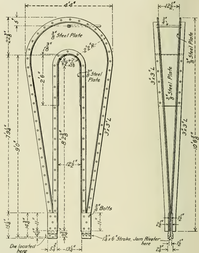
Yoke Riveter for Removing Staybolts.
