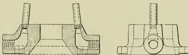
Fig. 3—Rectangular Nozzle Used on the Lake Shore.
