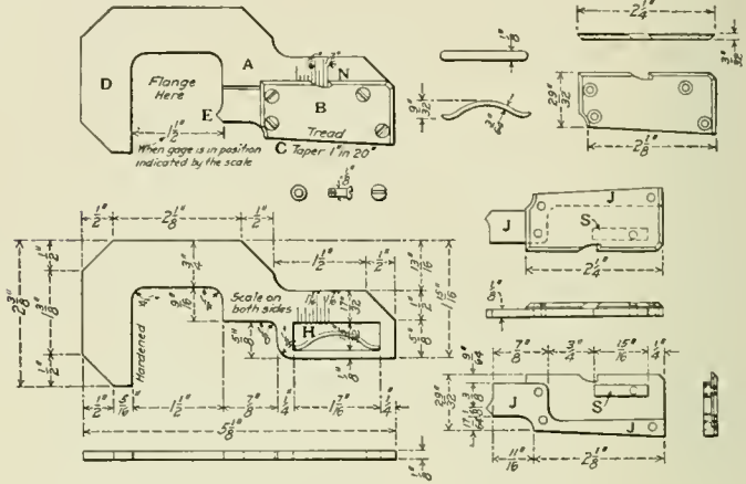
Fig. 7—Gage for Measuring Flange Thickness.
