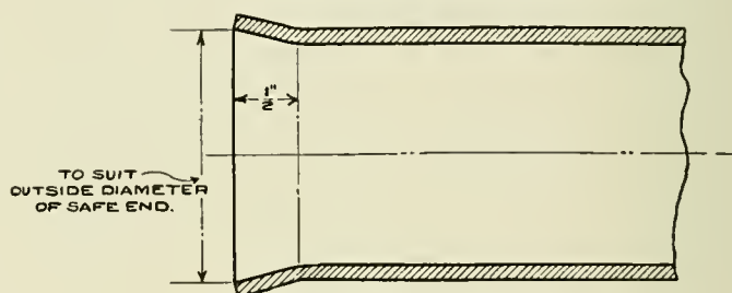
Fig. 2—Flue Flared for Safe-End.
