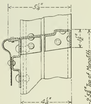
Sash Rest at Main Post.
