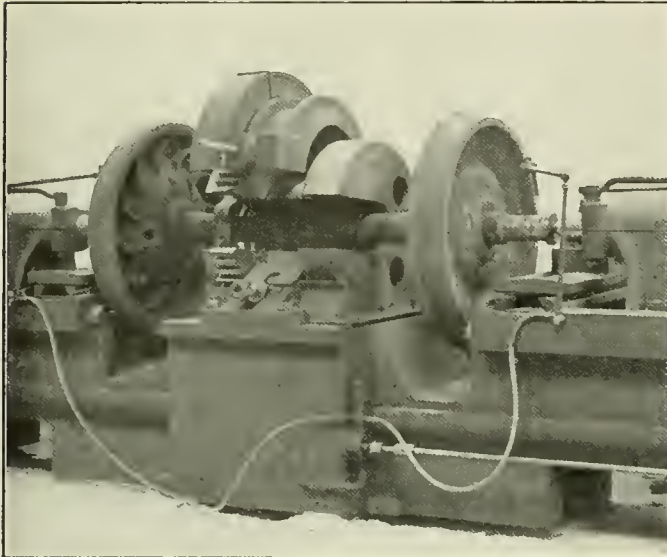
Journal Turning Lathe; Can Also be Used for Turning Axles.
