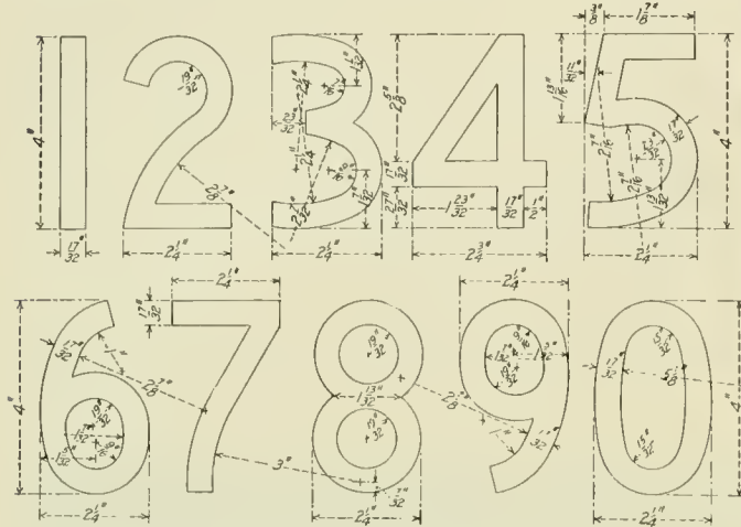
Headlight Numbers Used on the Canadian Pacific.
