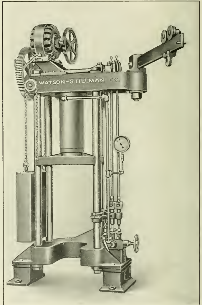
Compact Powerful Hydraulic Press for General Shop Use.
