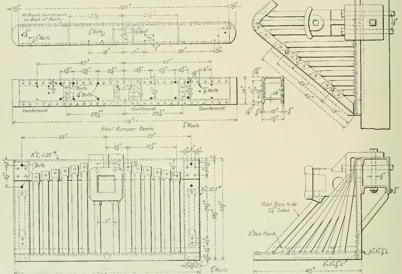
All-Steel Pilot and Bumper.
