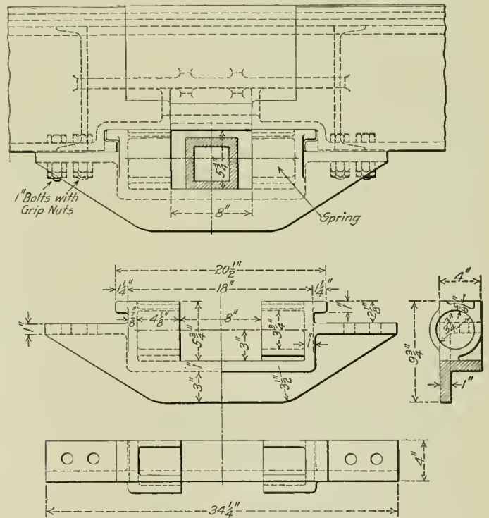
Cast Steel Drawbar Carrier for Tenders.
