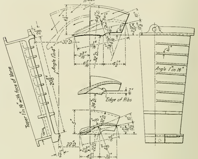
Details of the Gyru Spark Arrester.
