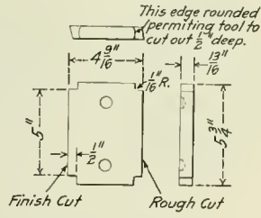
Jig for Finishing the Inner Faces of the Filling Blocks.
