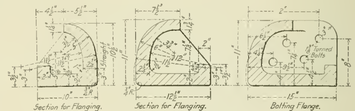
Fig. 1—Sections of Formers Suitable for 800-Ton Press.
