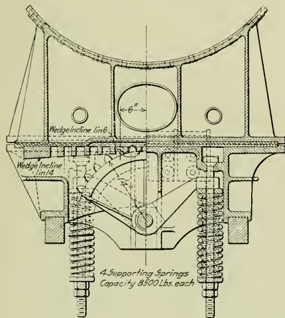
Forward Boiler Bearing and Centering Device; Canadian Pacific Mallet Locomotive.
