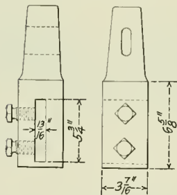
Tool to Bore Retaining Blocks.
