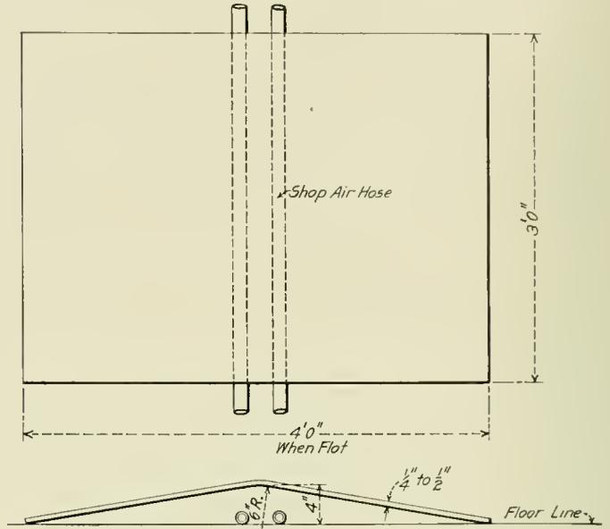
Fig. 2—Bridge Plate for Protecting Shop Hose.
