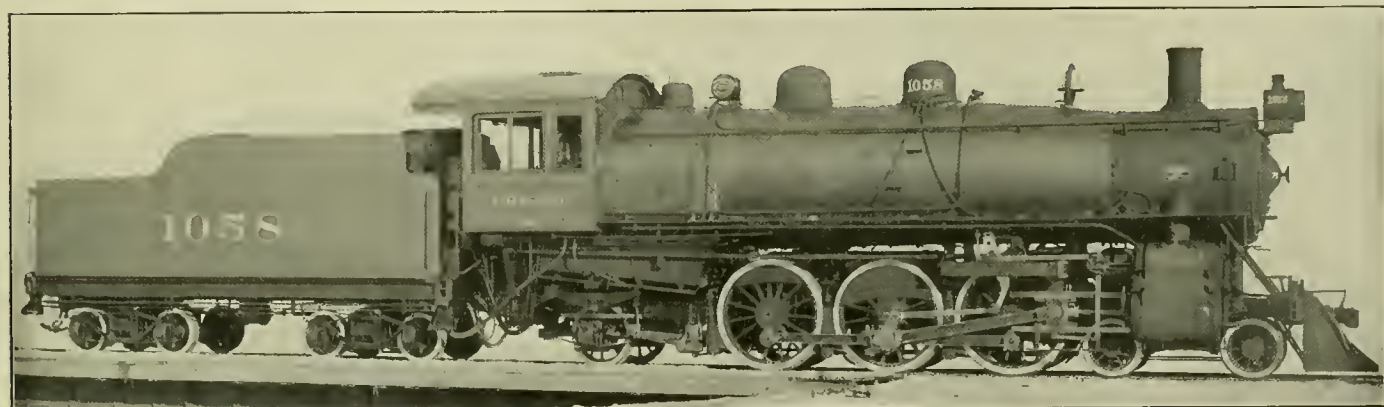
Pacific Type Superheater Locomotive of Exceptional Power at Moderate Speeds.
