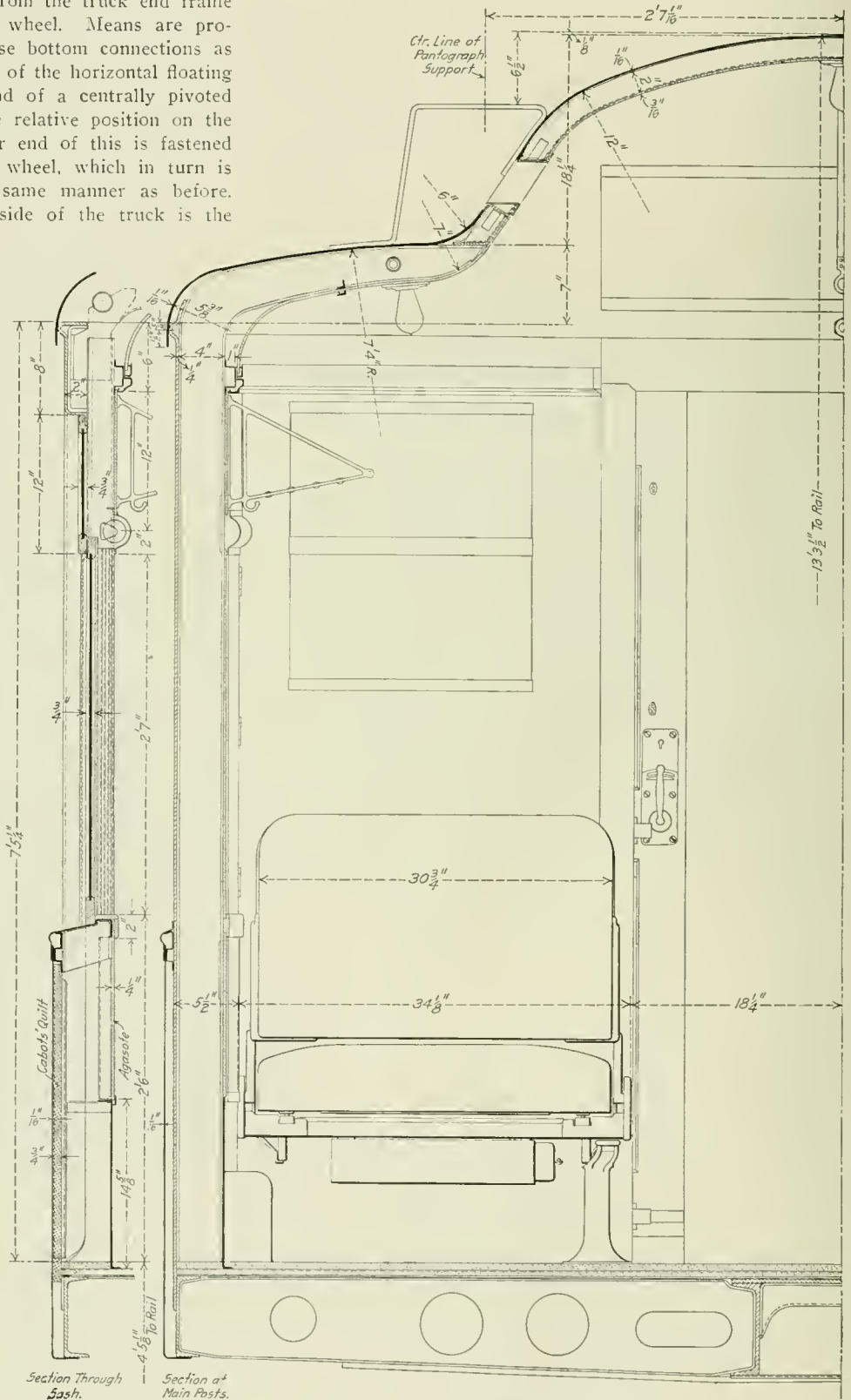
Cross Sections Showing Construction of Exterior and Interior Finish, All-Steel Suburban Car.
