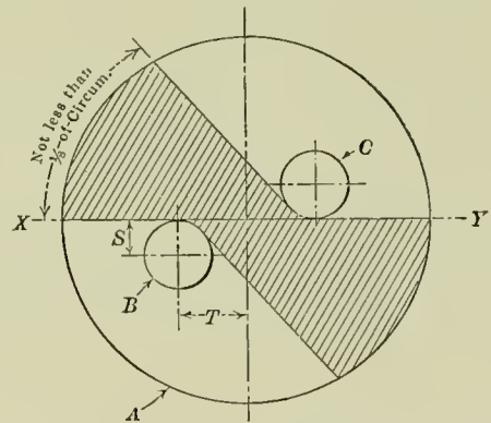
Circle A =circumference of drill. Diameter of circles B and C = \frac{3}{16} diameter of drill. S=\frac{3}{32} of diameter of drill. T=\frac{3}{16} of diameter of drill. XY =indicates cutting edges.
