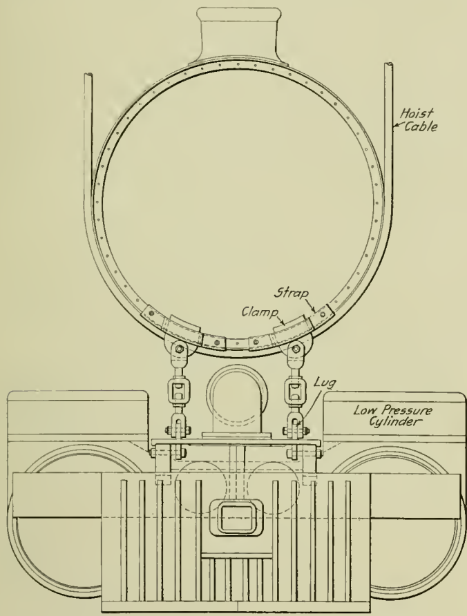
Method of Fastening Low Pressure Cylinders to the Boiler of a Mallet Locomotive so That it can be Lifted by a Crane.
