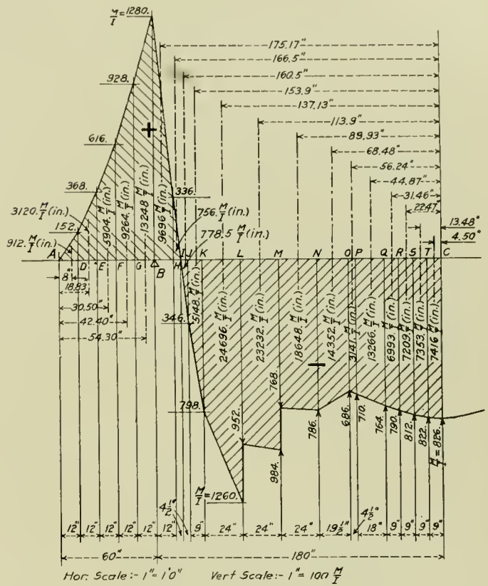
Fig. 12— \frac{M}{I} Curve for Center Girder.
