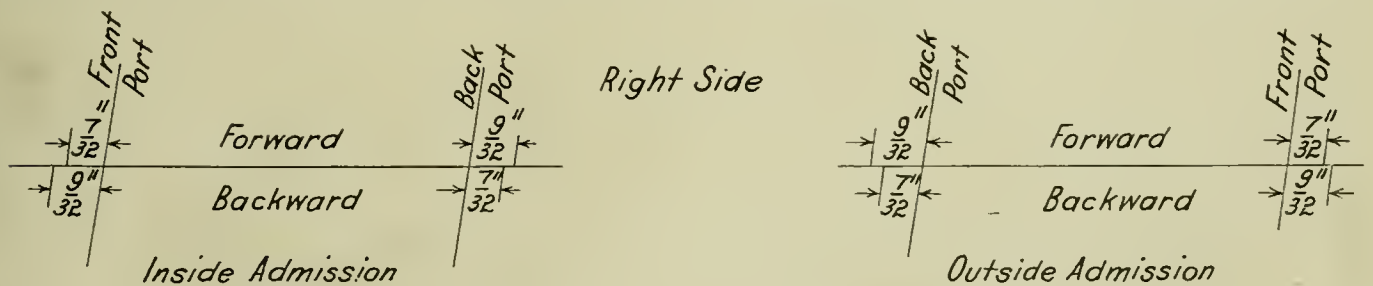
Fig. 6—Correct Adjustment of Valves of Baker Gear as Shown by Marks on Valve Stems.
