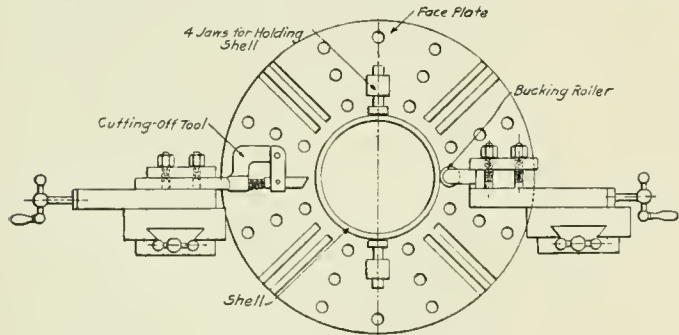
Fig. 3—Cutting Off the Rings.
