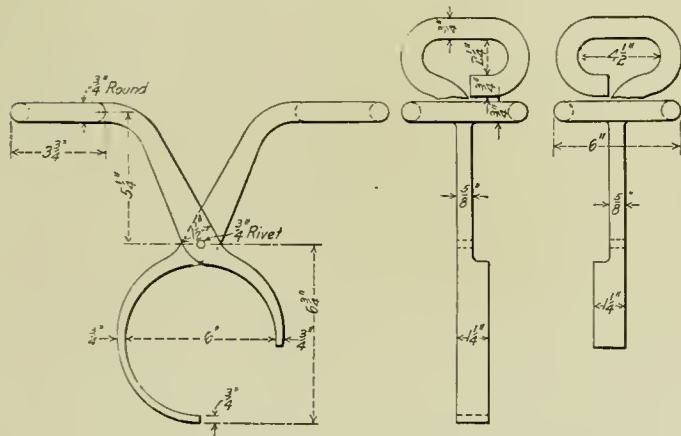
Fig. 1—Tongs for Handling Axles.
