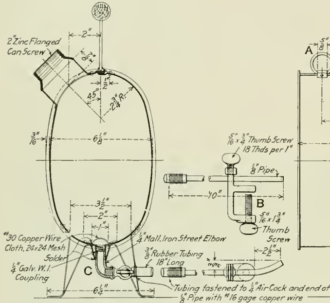
Fig. 4—Water Tank for Cooling Hot Journal Boxes.
