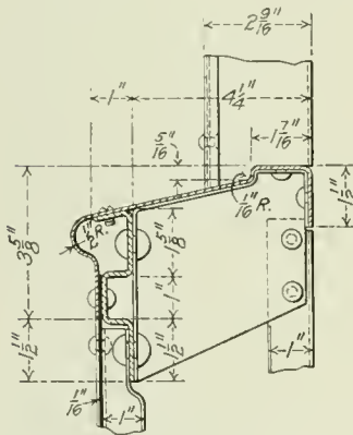
Sash Rest at Intermediate Post.
