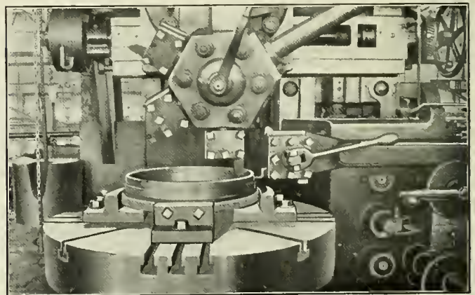
Machining Piston Valve Rings.
