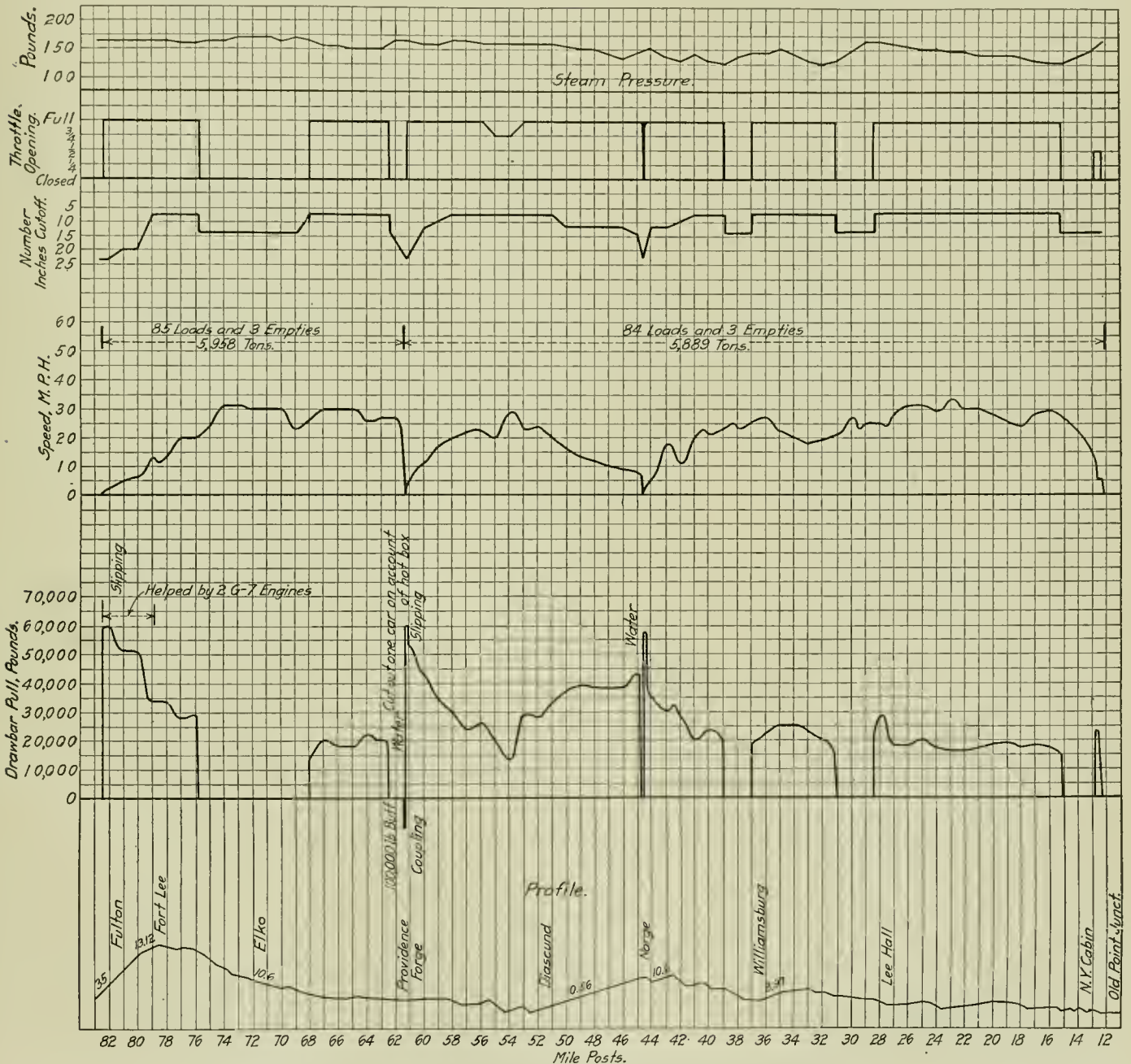
Graphical Record of a Recent Test of a Chesapeake & Ohio Mikado Locomotive.
