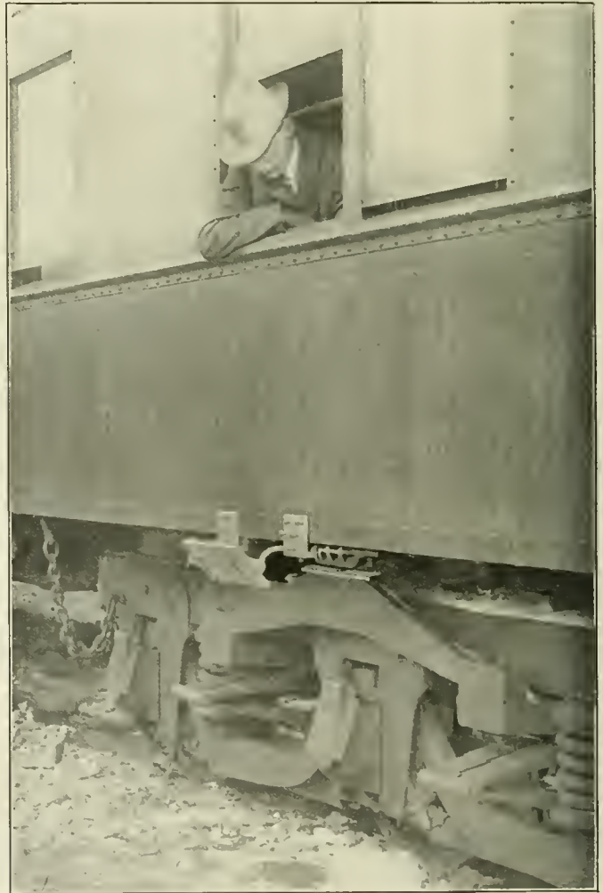
Mirror for Inspecting Side Bearing Motion.
