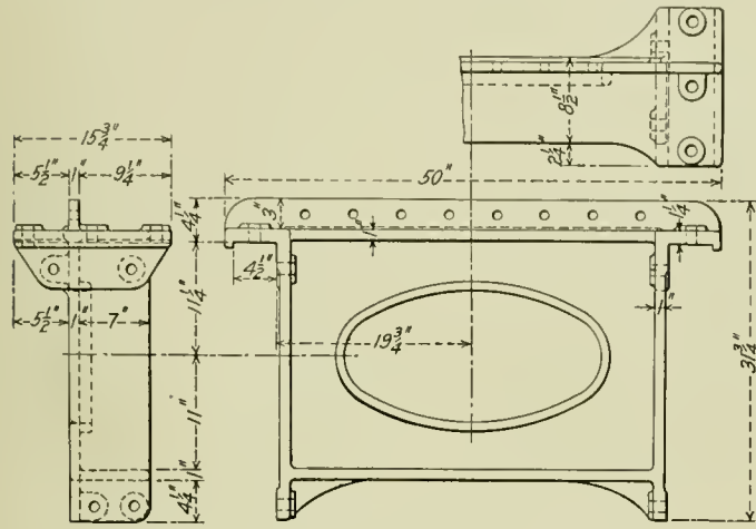
Frame Brace Ahead of Third Pedestal.
