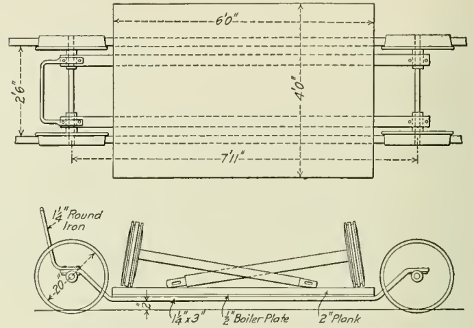
Fig. 3—Car Used for Handling Material Between Engine House and Shops.
