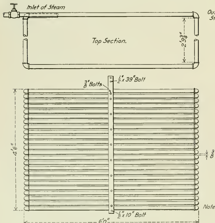
Fig. 2—Steam Coil for Drying Sand.
