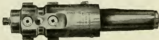
Expansion Boring Tool for Steel Wheels.
