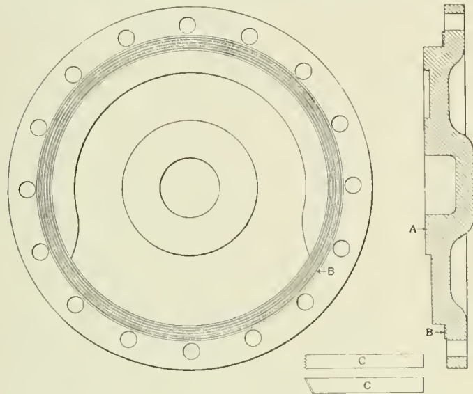
Fig. 8—Method of Grooving Cylinder Heads.
