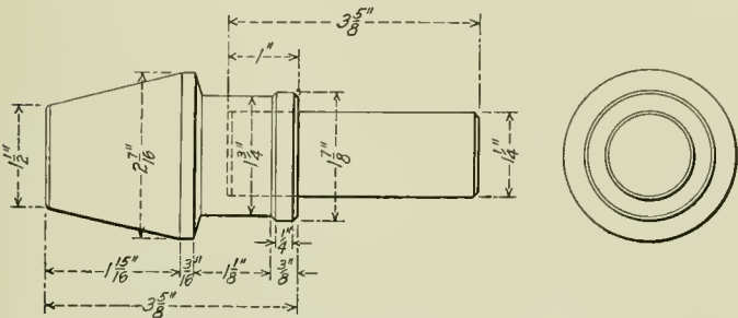
Fig. 12—Pneumatic Tool for Flaring Boiler Tubes.
