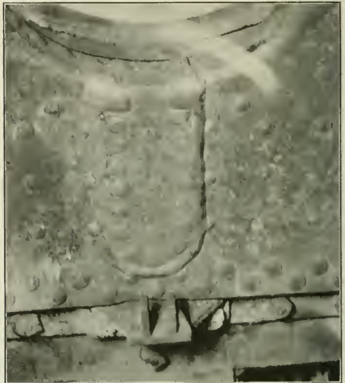
Fig. 5—Patch Under Fire Door with Edges Welded Instead of Calked.
