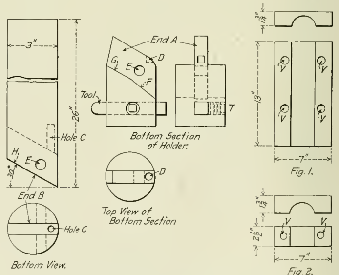
Tool Post for Slotting Machine.
