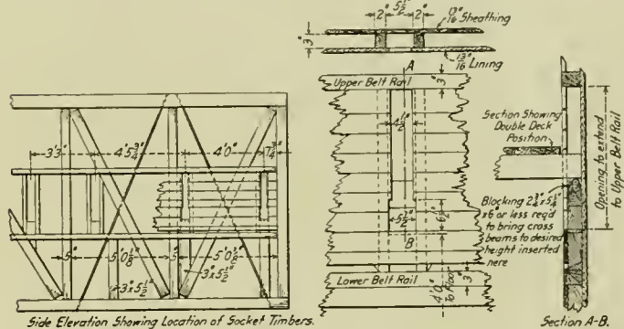
Arrangement of Double Deck Supports for Automobile Car.
