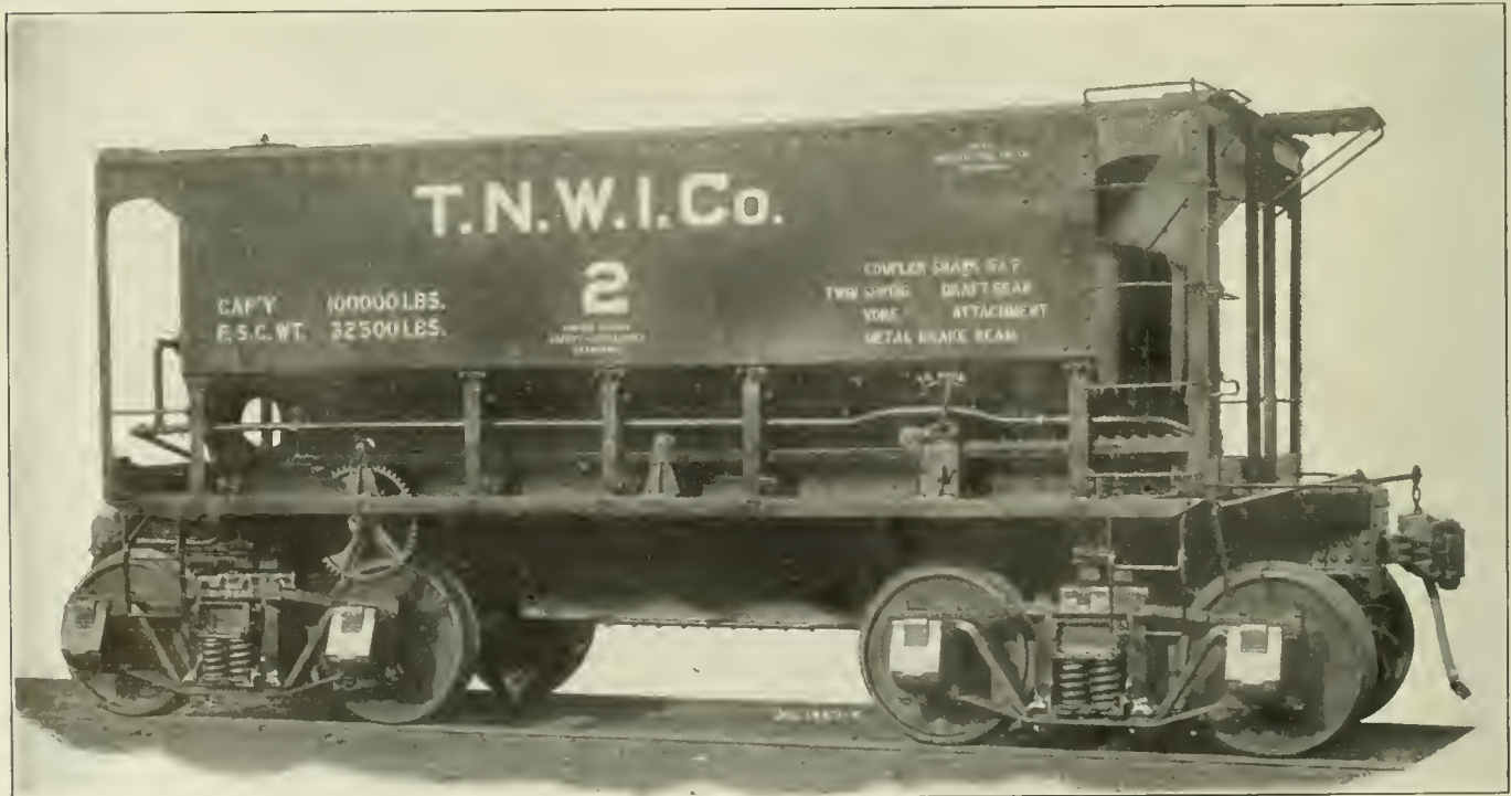
Steel Self-Clearing, Quick-Dumping Ore Car for the Northwest.
