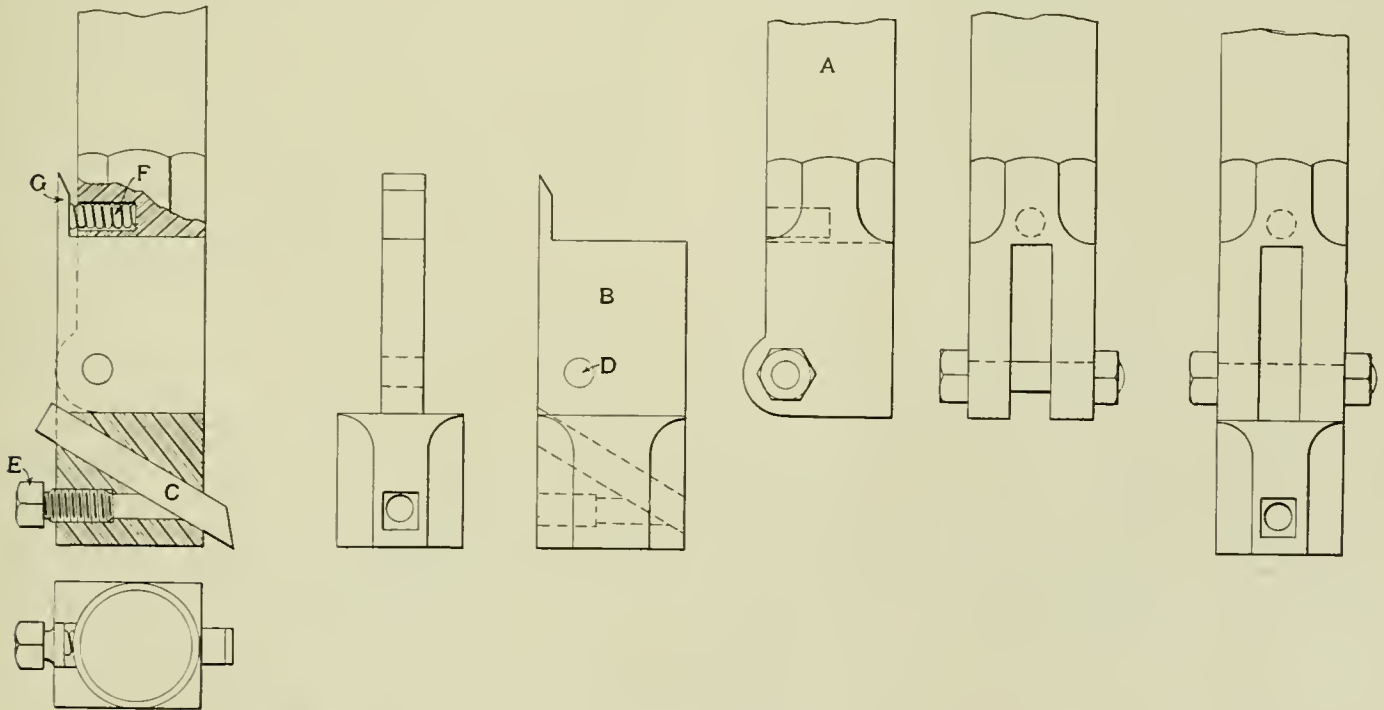
Fig. 7—Tool Bar for Slotting Machine.
