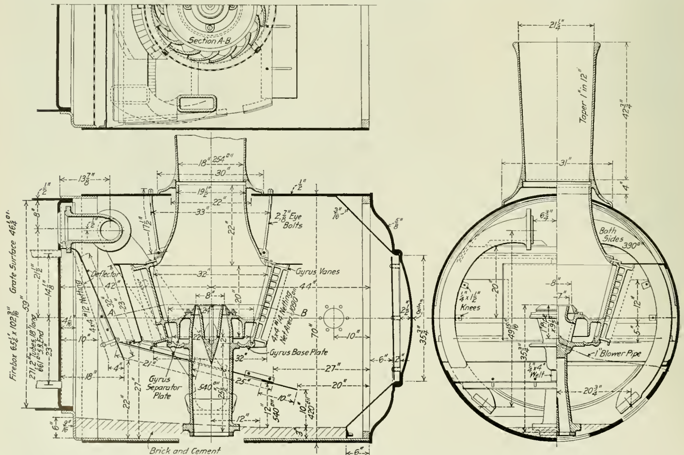
Gyrus Spark Arrester Applied to Smokebox of a Pacific Type Locomotive; Chicago & North Western.
