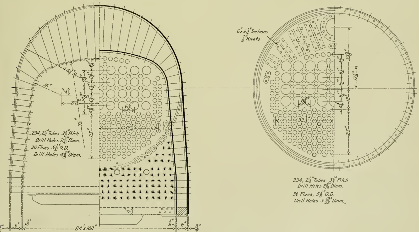
Sections of the Firebox and Boiler of the Rock Island Mikados.
