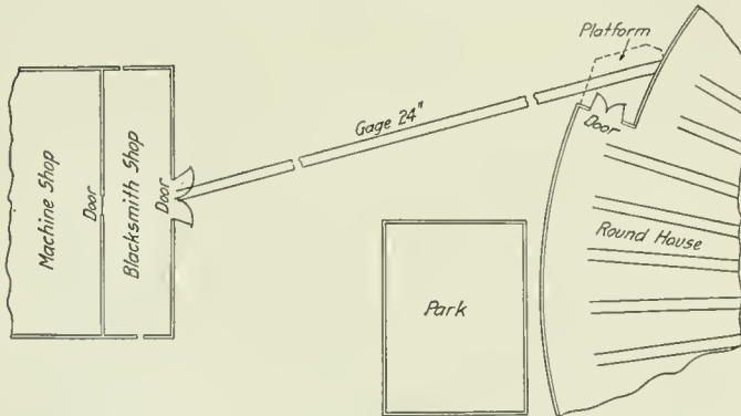
Fig. 2—Delivery Track Between Engine House and Machine Shop.
