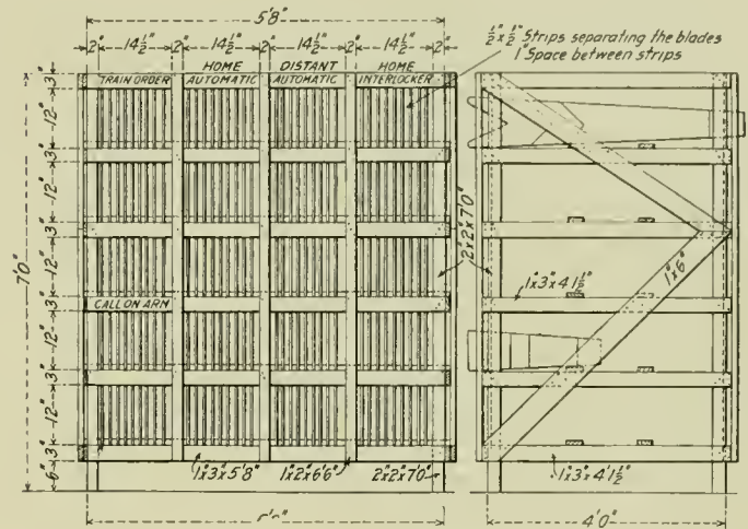
Fig. 1—Rack for Storing Painted Signal Blades.
