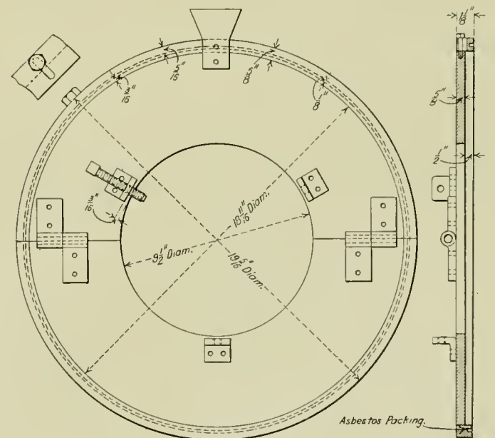
Fig. 8—Mold for Casting Hub Liners.
