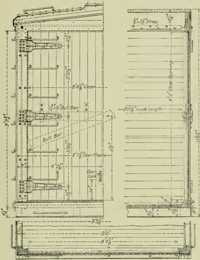
Construction of End Door on Automobile Car.
