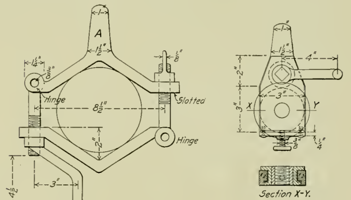
Fig. 3—Clamp and End View of Axle Center Facing Jig.
