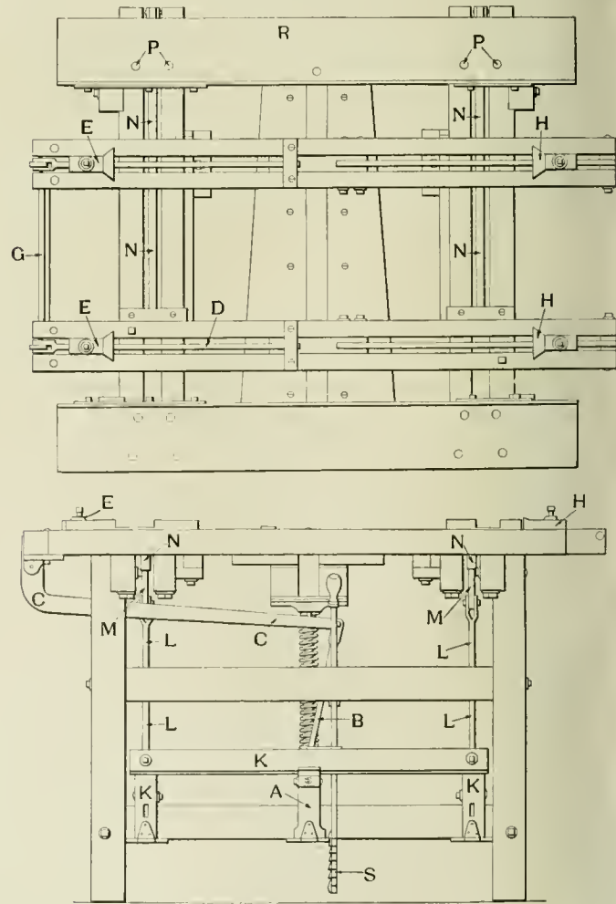
Fig. 6—Side, End and Top Views of Sash Clamp.
