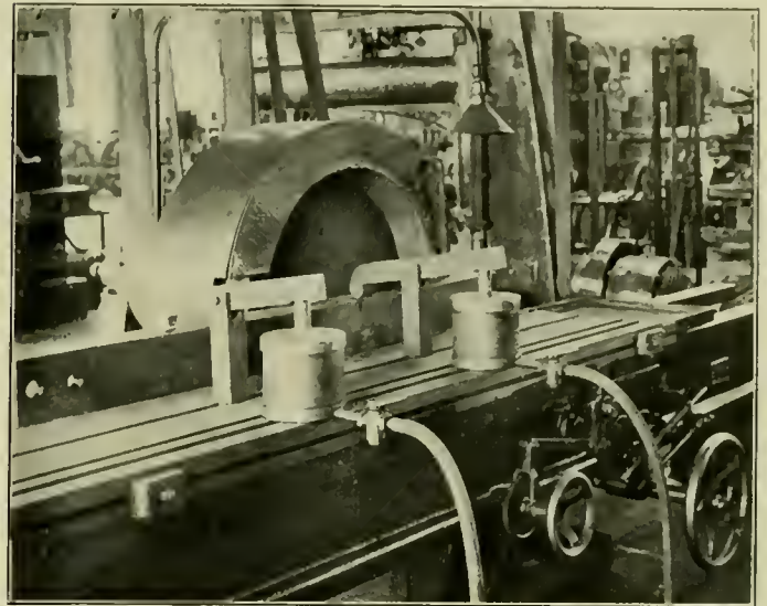
Fig. 7—Air Cylinders Used for Clamping Guide Bars to Grinding Machine.
