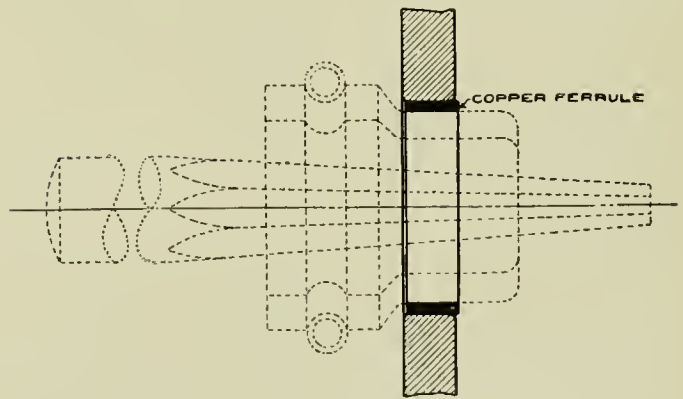
Fig. 6—Tightening Copper Ferrule in Back Flue Sheet.
