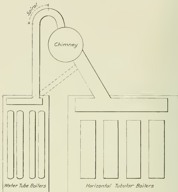
Arrangement of Boilers and Smoke Flues.
