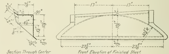
Fig. 2—Locomotive Ash Pan Wheel Cover.
