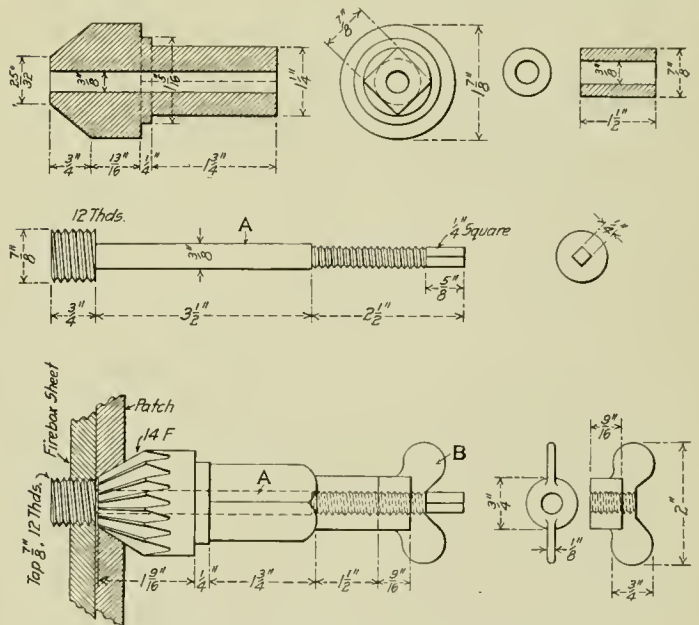
Reamer for Countersinking Patch Bolt Holes.
