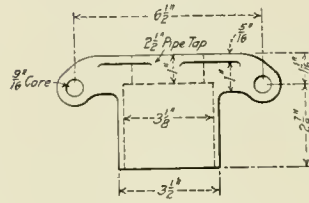
Drip Cup Support.
