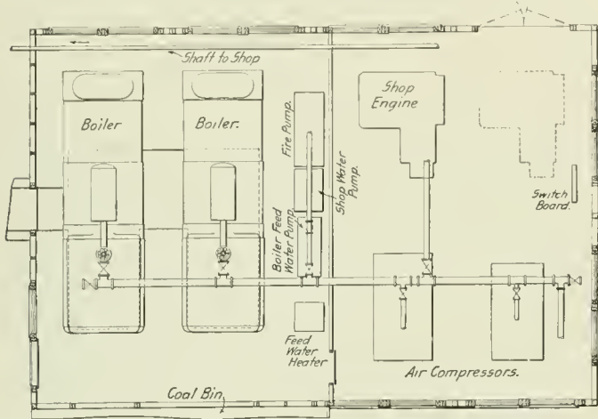
Fig. 3—Arrangement of Power House Equipment.
