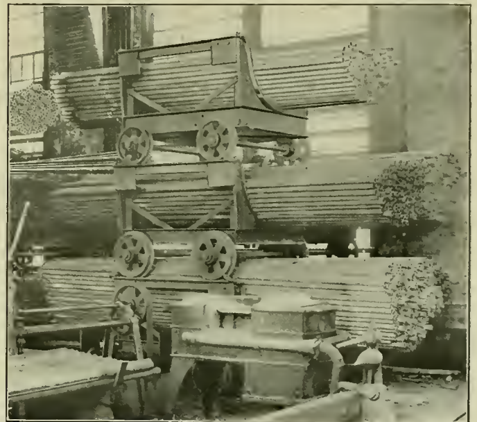
Fig. 6—Method of Tiering Flue Cars on Storage Tracks, Each Car Holds One Complete Set of Tubes.
