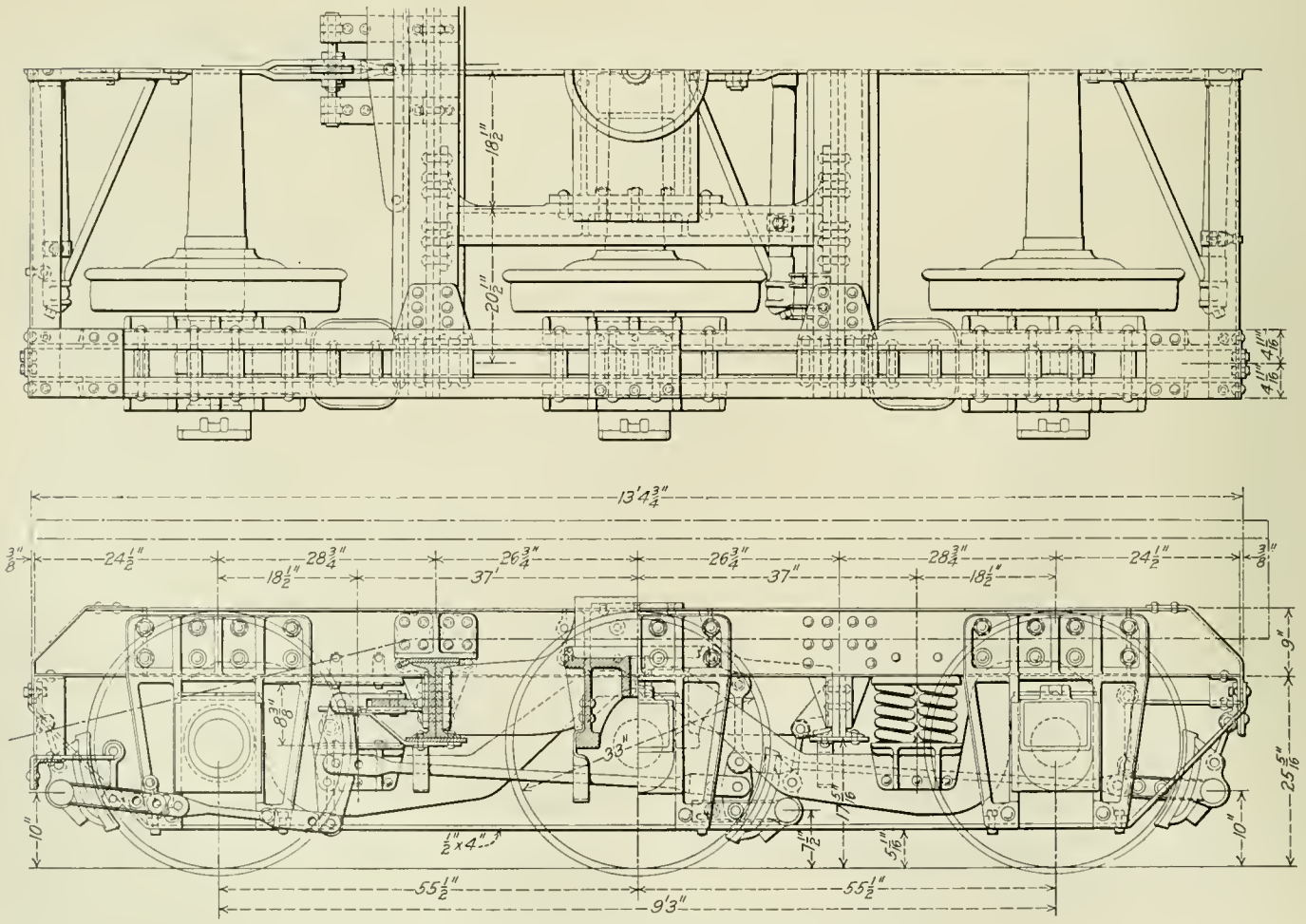
Six-Wheel Truck Used Under 200,000-Lb. Capacity Flat Car.
