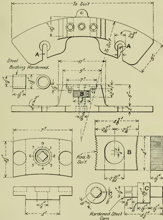
Fig. 6—Chuck for Holding Tires.
