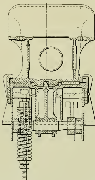
Forward Boiler Bearing and Centering Device; Canadian Pacific Mallet Locomotive.
