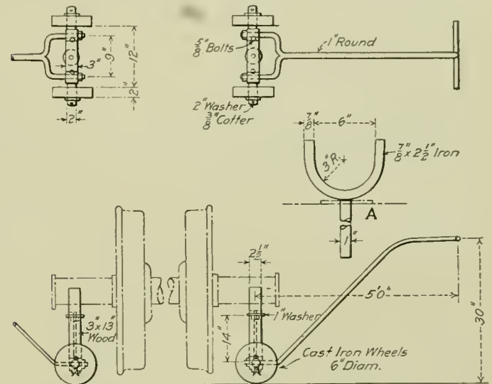
Fig. 2—Truck for Handling Mounted Car Wheels.
