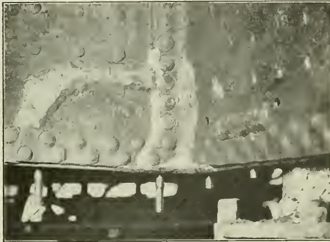
Fig. 9—Electrically Welded Crack in Corner of Firebox.
