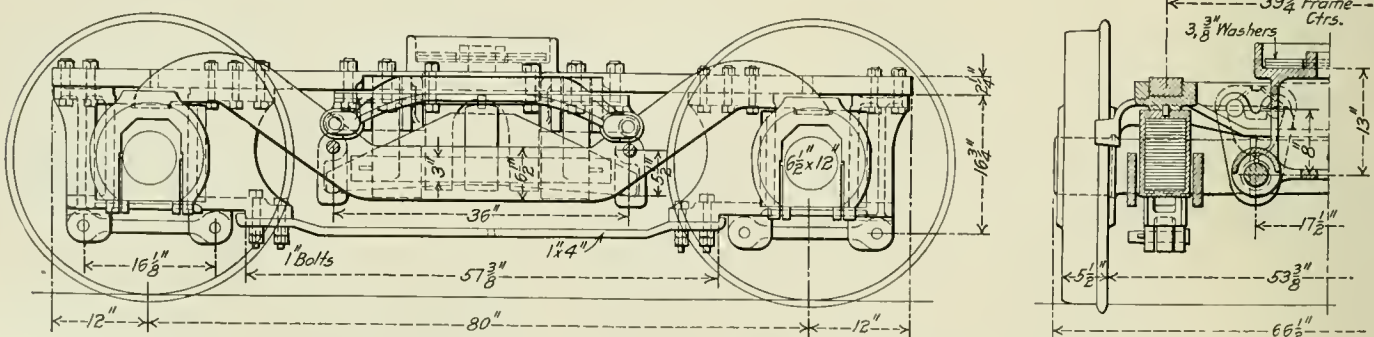
Engine Truck with Collar on the Axle Inside of the Journal Box; Lackawanna 4-6-2 Type Locomotive.
