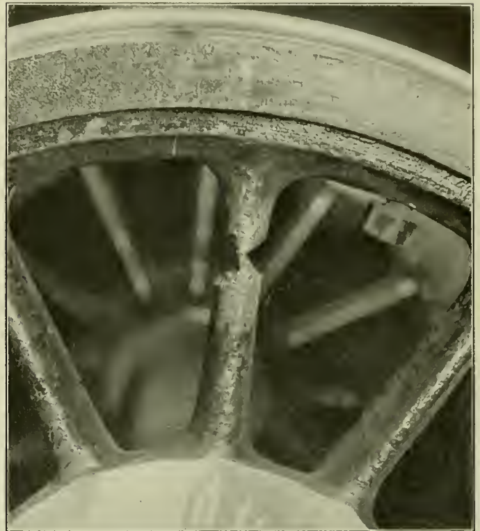
Fig. 14—Cracked Wheel Spoke Chipped Preparatory to Welding.
