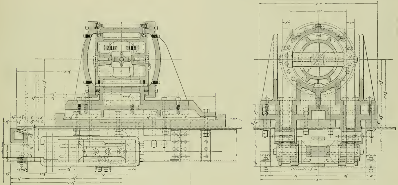
Dynamometer of 1,000,000 Lbs. Capacity; Santa Fe Dynamometer Car.
