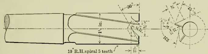
Fig. 4—New Design of End Mill with Five Teeth.
