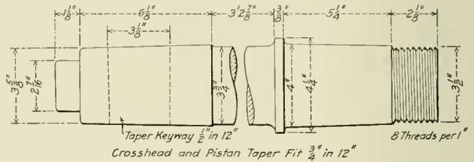
Piston Rod to Which the Operations Specified Apply.
