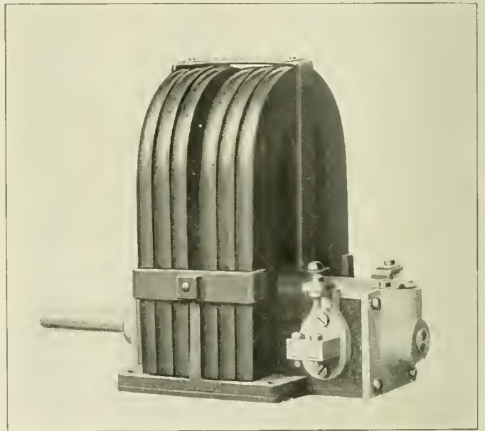
Magneto-Generator Arranged as a Speed Indicator.
