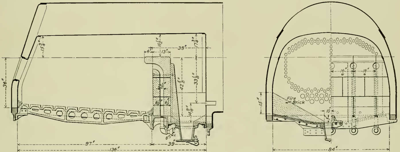
Fig. 5—Details of Construction of Gaines Combustion Chamber.
