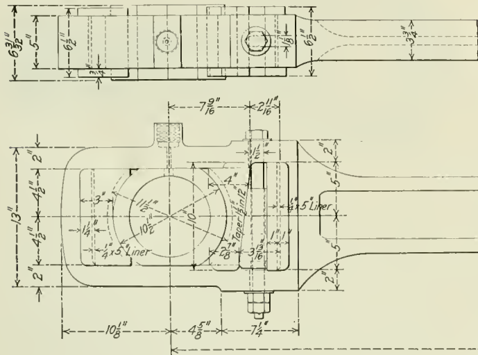
Solid End Main Developed at the Clinton Shops of the Chicago & North Western.
