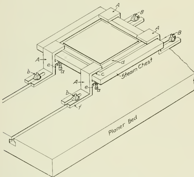
Jig for Planing Balance Plates.
