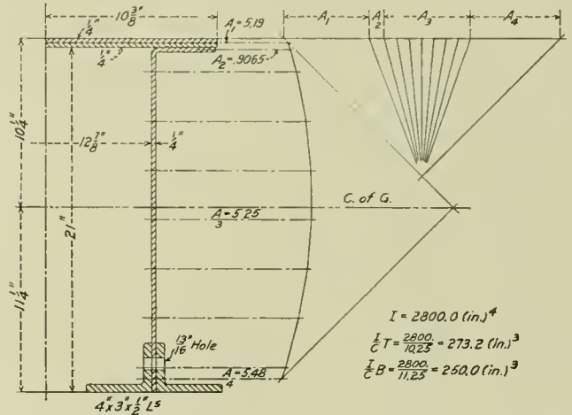
Fig. 9—Section at M , Corresponding to Curve 4, Fig. 2.
