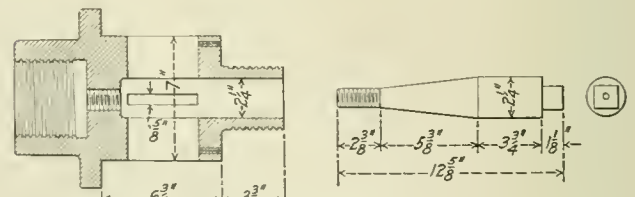
Mandrel for Turning Main Rod Brass.
