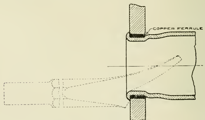
Fig. 10—Beading Flues in Firebox Flue Sheet.
