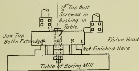
Piston Heads Operation No. 1.
