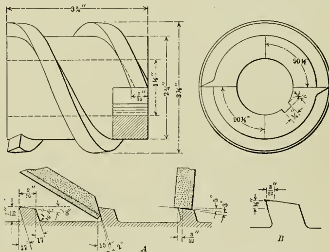
Fig. 7—New Design of Helical Cutter.
