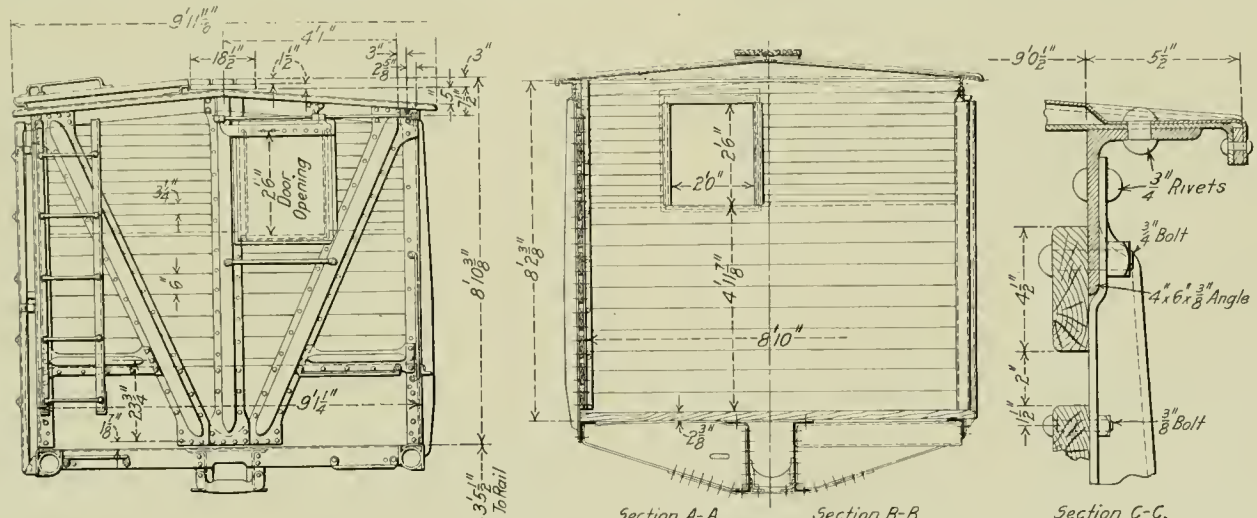
End Elevation and Sections of Steel Frame Stock Car.
