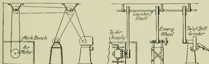
Fig. 5—Pneumatic Drive for Tool Room.
