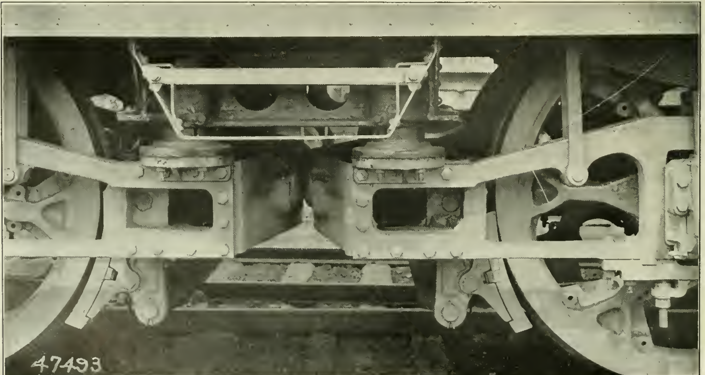
Articulated Connection and Cab Supports of Electric Locomotive.
