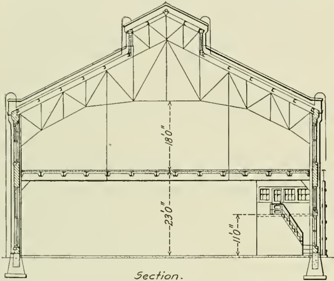
Sectional and End Elevation of the Planing Mill.
