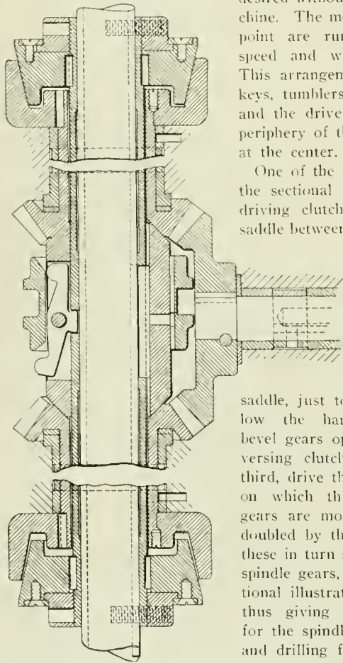
Driving Clutch on Rochester Boring Machine.
