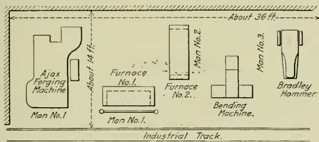
Fig. 1—Arrangement of Machines and Furnaces for Manufacturing Brake Beam Hangers.
