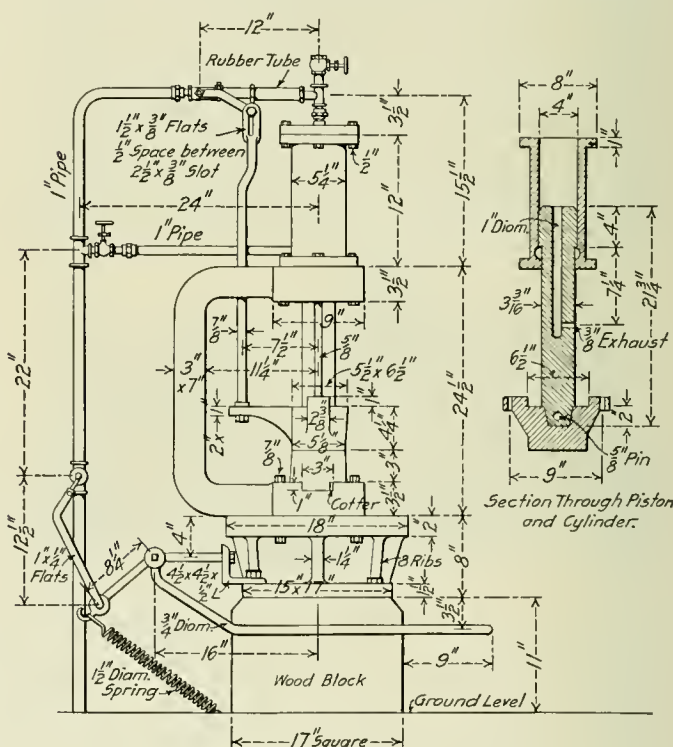
Air Hammer for Light Smith Shop Work.
