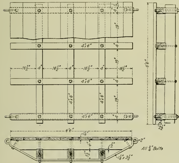
Fig. 1—Wooden Platform for Carrying Scrap.
