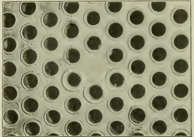
Fig. 21—Welded Tubes After Being Chipped and Trimmed.
