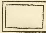
Terminus inversum positus.
