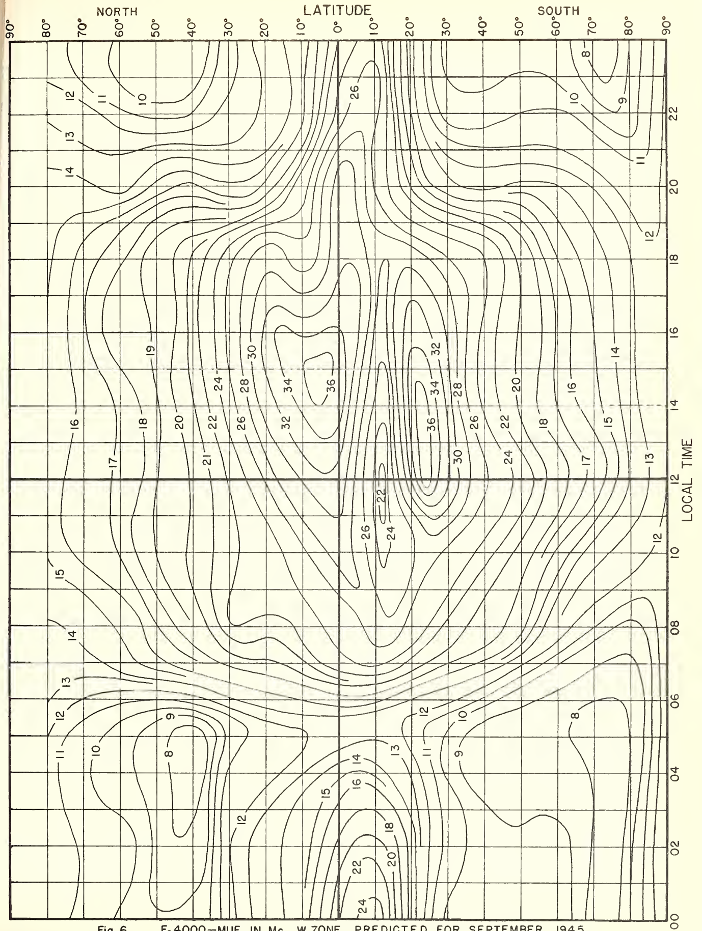
Fig. 6. F_2 4000-MUF , IN Mc, W ZONE, PREDICTED FOR SEPTEMBER, 1945.
