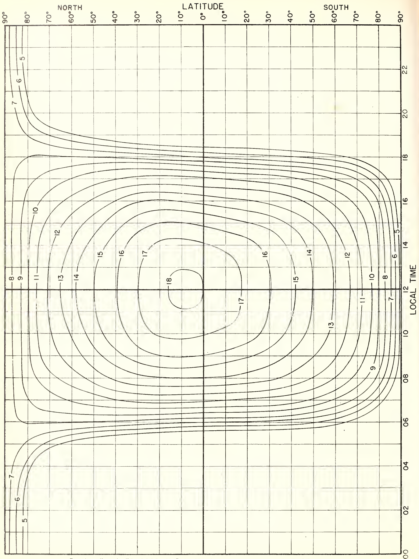
Fig.II. E-LAYER 2000-MUF, IN Mc, PREDICTED FOR SEPTEMBER, 1945.
