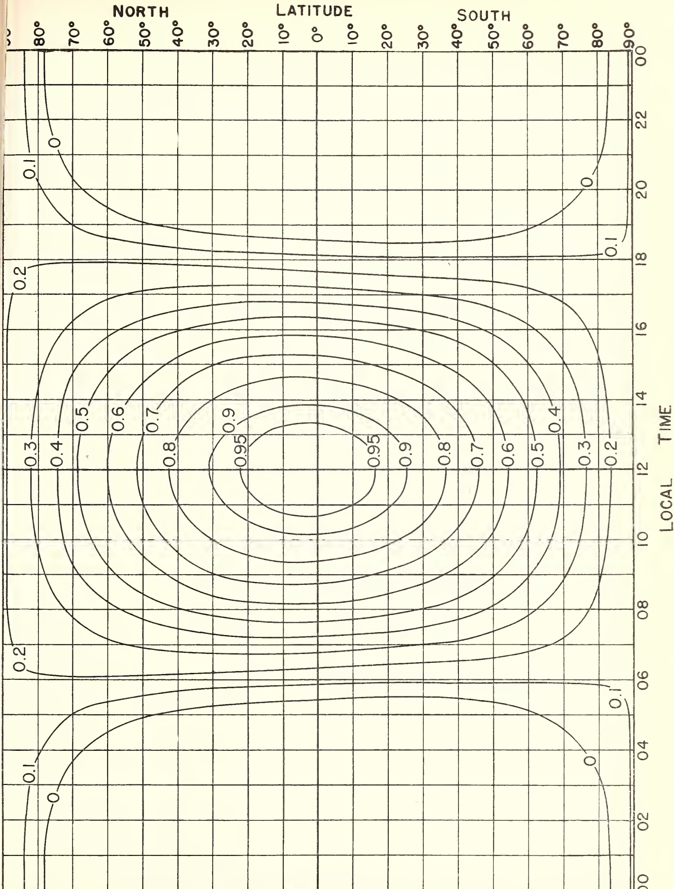
Fig. 16. ABSORPTION INDEX CHART (EXCLUDING AURORAL ABSORPTION) FOR SEPTEMBER.
