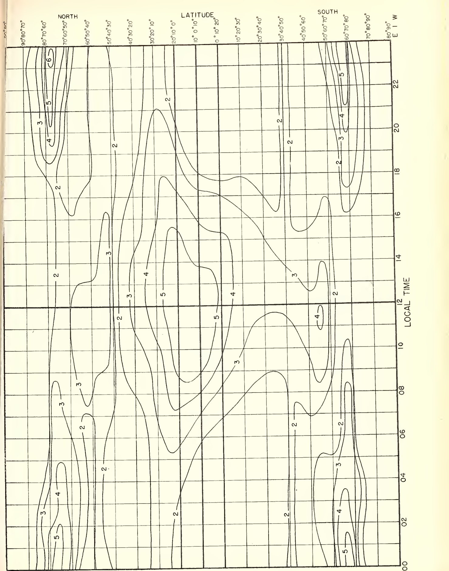
Fig. 12. MEDIAN fE_s , IN Mc, PREDICTED FOR SEPTEMBER, 1945.
