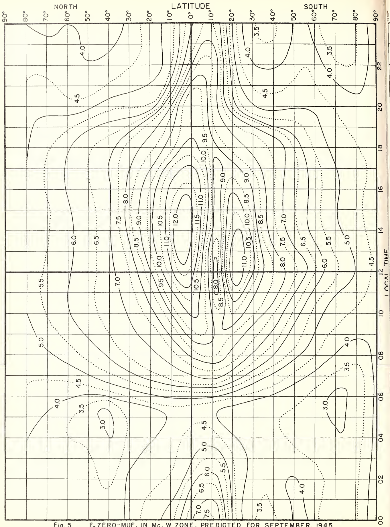
Fig. 5. F_2 ZERO-MUF, IN Mc, W ZONE, PREDICTED FOR SEPTEMBER, 1945.
