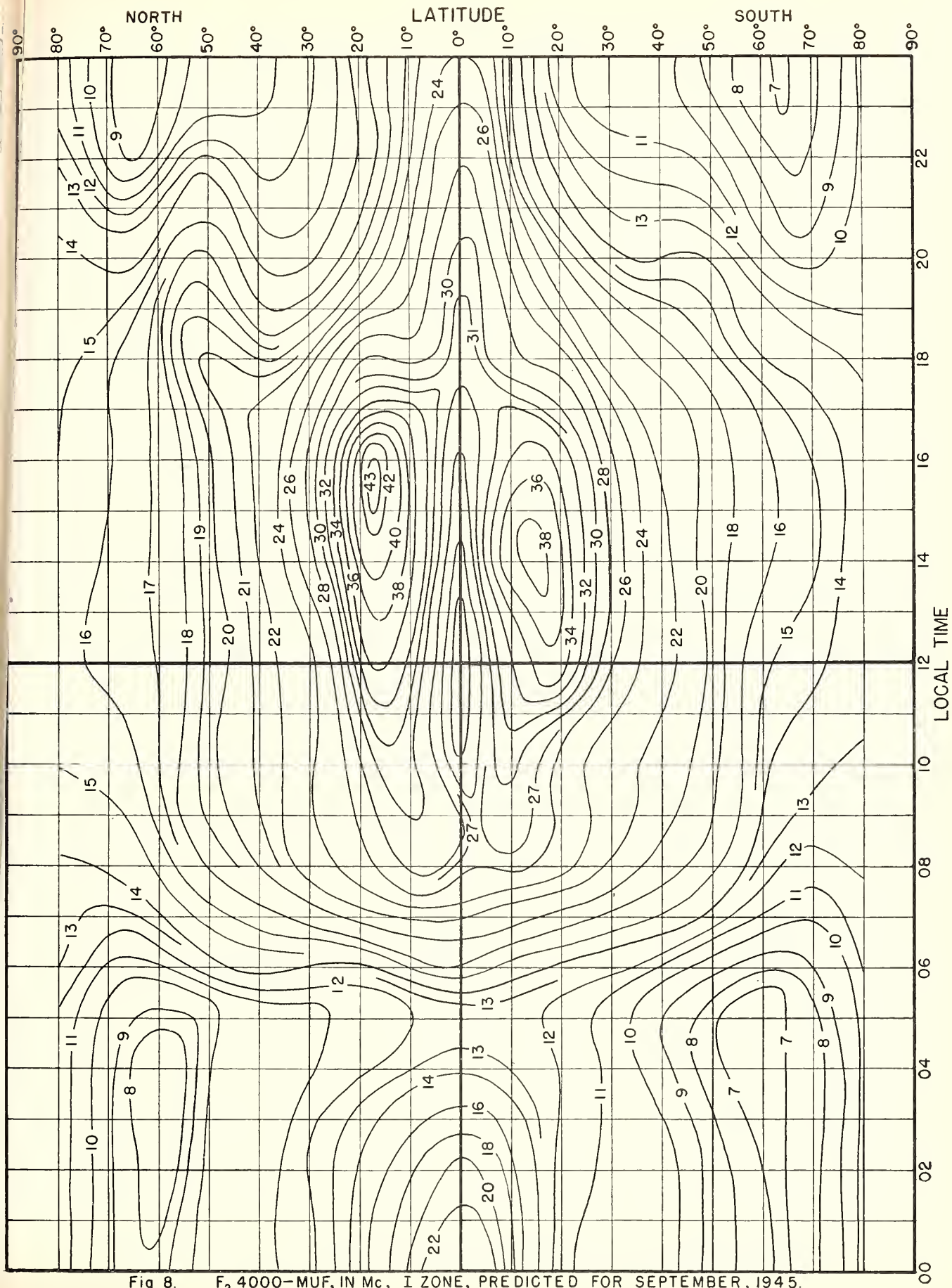
Fig 8. F 2 4000-MUF, IN Mc, I ZONE, PREDICTED FOR SEPTEMBER, 1945.
