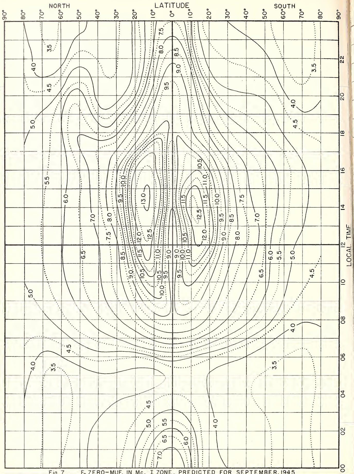
Fig. 7. F 2 ZERO-MUF, IN Mc, I ZONE, PREDICTED FOR SEPTEMBER, 1945
