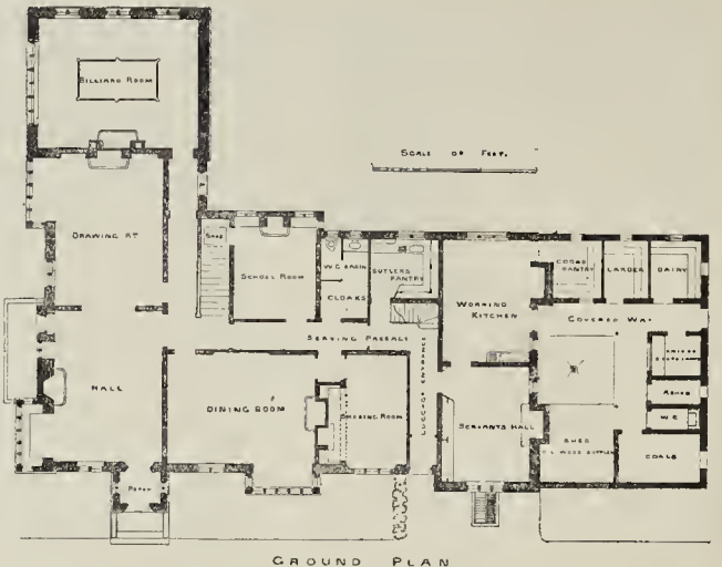
Plan of "Firsdene."—Messrs. Latman & Bateman, Architects.
