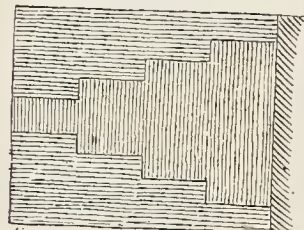
Arrangement of Bricks, as seen on Underside of Arch.
