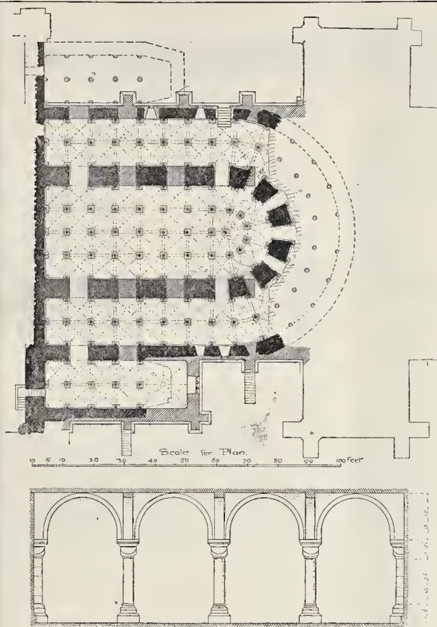
Worcester Cathedral: Plan and Part Section of Crypt. Measured and Drawn by Mr. Harold Brakspear.
