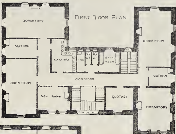
NEW ORPHANAGE FOR GIRLS WHITEINCH:GLASGOW.
