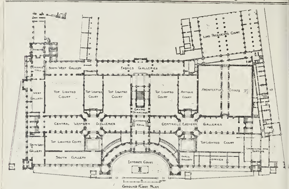
Competition Design for Completing South Kensington Museum: Submitted by Mr. John Belcher, F.R.I.B.A.
