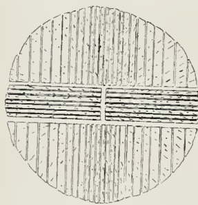
Transverse Section of Oak Log cut on the quarter. Dotted lines show the ray or silver grain in the wood, and the boards in which figure will be conspicuous on their surface.
