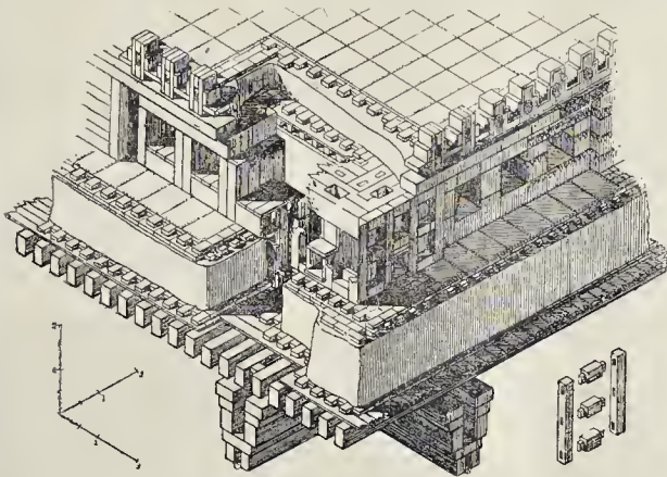
Fig. 7.—Restoration of Timber Roof, Persepolis.
