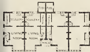
Plan of Almshouses.
