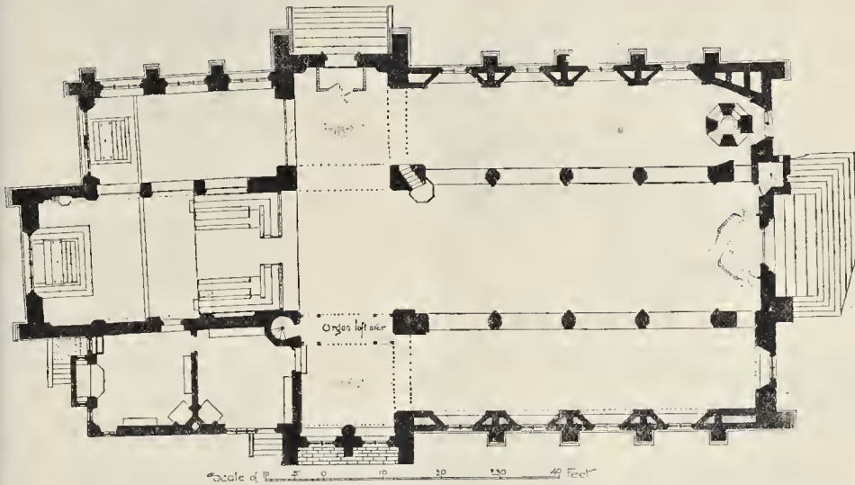
Competition Design for St. Luke's Church, Wincington: Plan.
