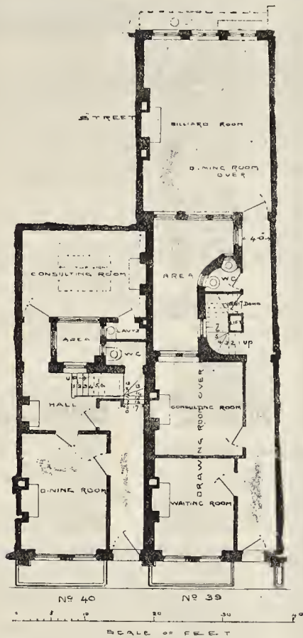
Plan of Houses in Margaret-street.
