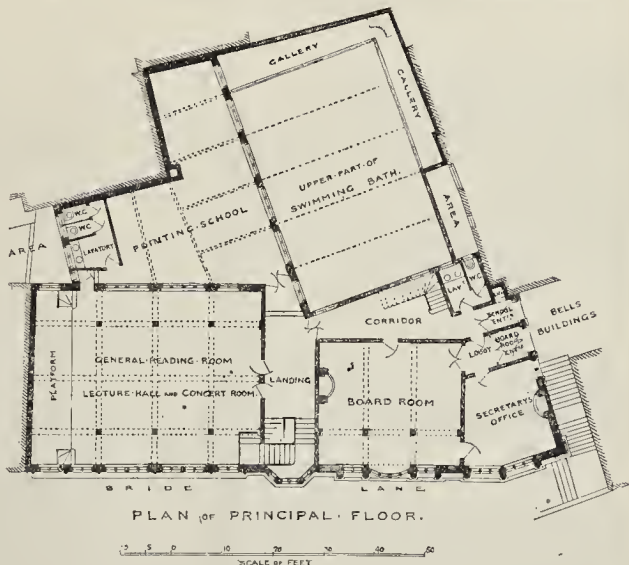
Competition Design for St. Bride's Foundation Institute.
