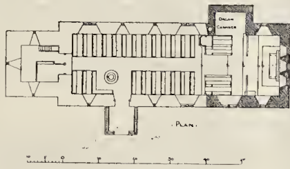
Plan of Norbury Church.
