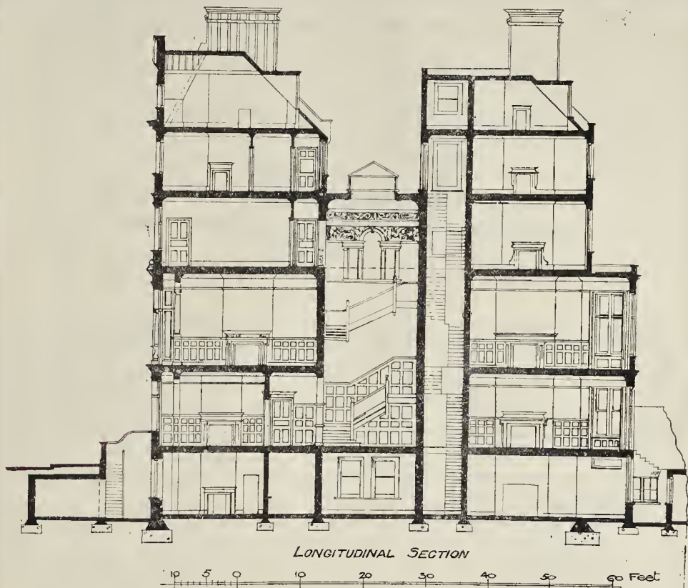
Design for a Town House.
