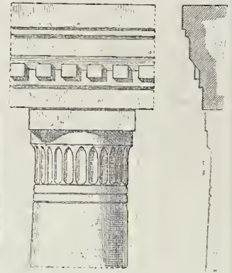
Fig. 4.—Detail of Capital in Fig. 3.
