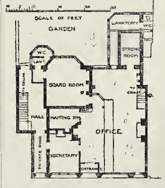
The Alliance Assurance Offices, Abbeygate-street, Bury St. Edmunds.—Mr. J. S. Corder, Architect.
