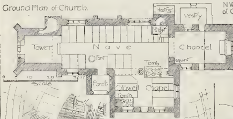
Ground Plan of Church.
