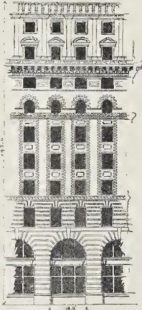
Part Elevation of Crocker Wolworth National Bank Building, San Francisco. (Total length of two street fronts, 329 ft.)
