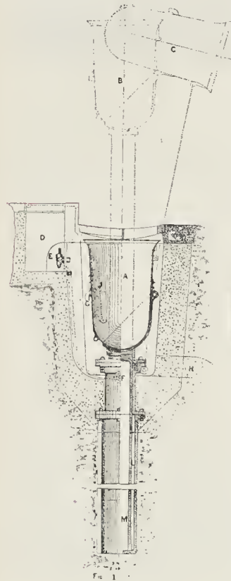
SECTION Bennett's Hydraulic Self-Cleaning Street Gully.
