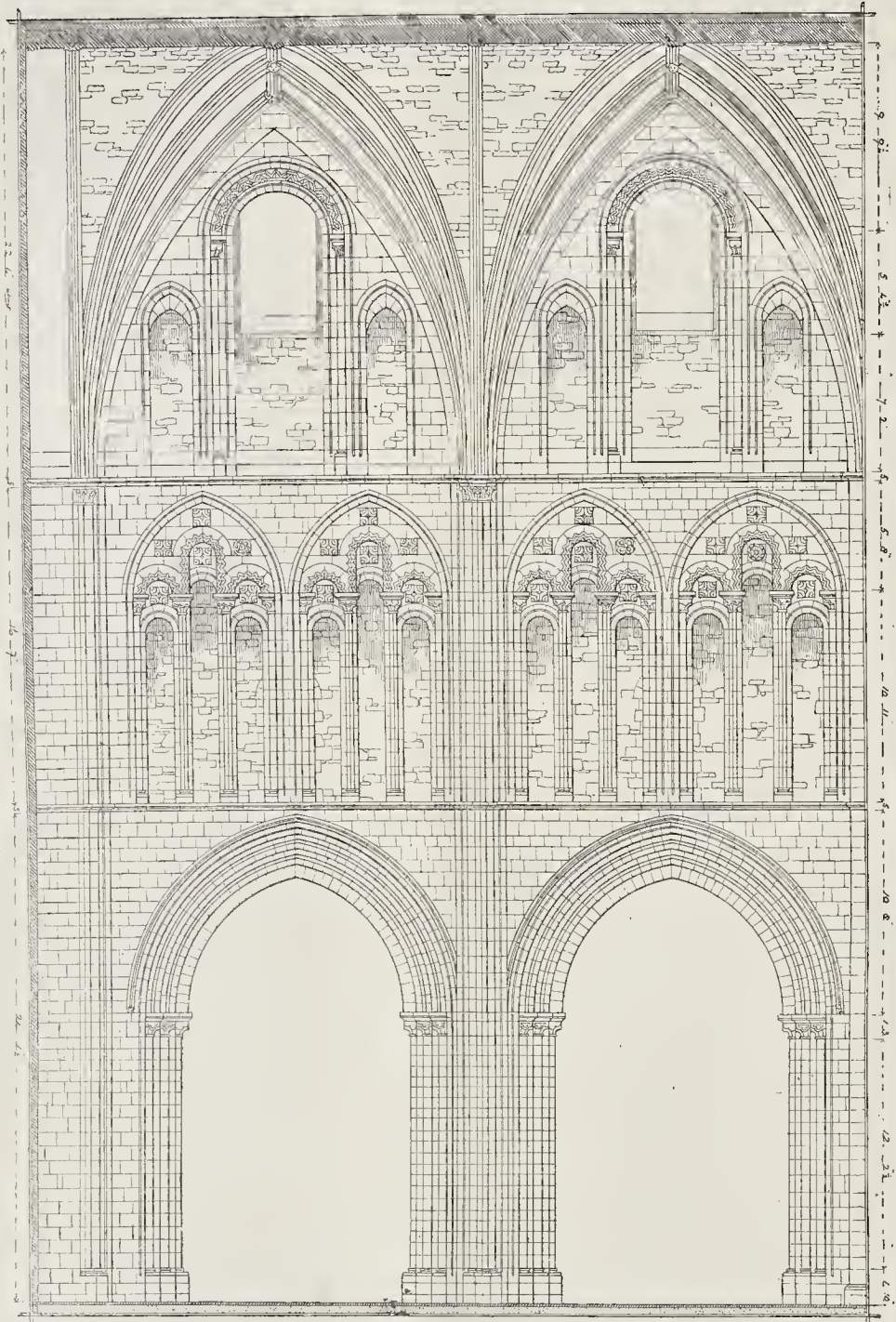
Worcester Cathedral: Interior Elevation of Two Western Bays of Nave. Measured and Drawn by Mr. Harold Brakspear.
