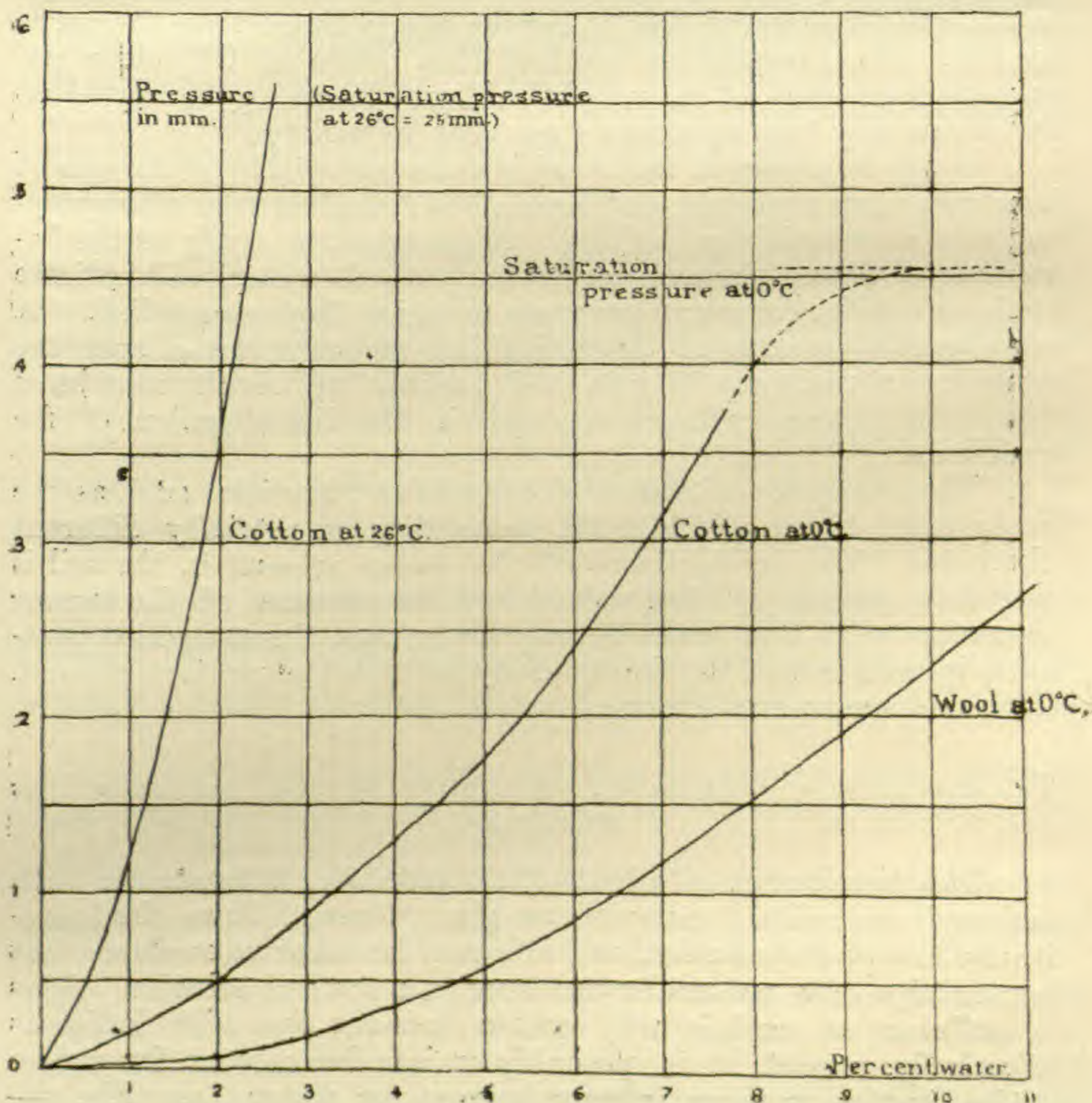
FIG. 2.—Absorption of water by cotton and wool.
