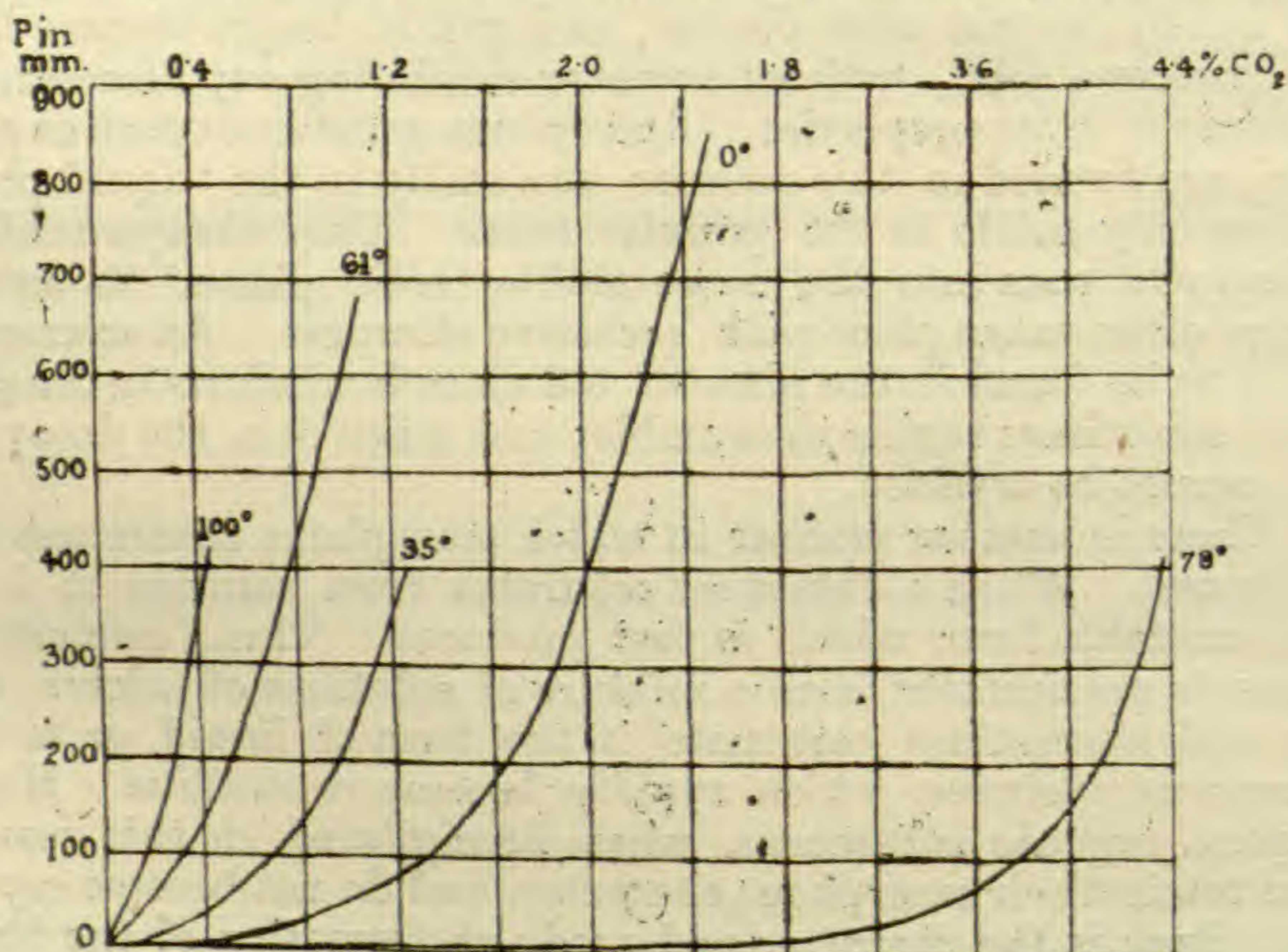
FIG. 1.—Absorption of carbon dioxide by charcoal.
