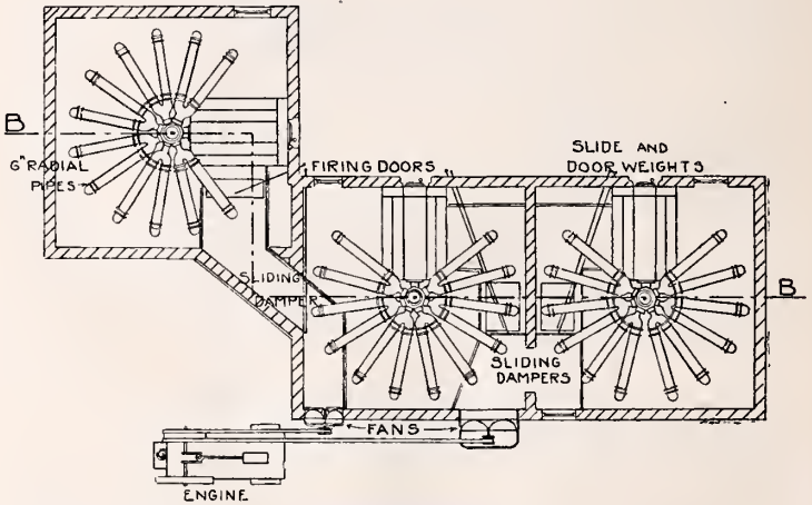
— SECTIONAL PLAN —
