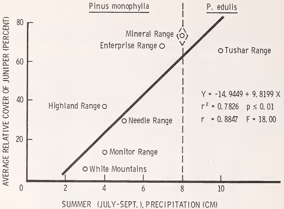
Figure 8.--Relationship of relative juniper tree cover to amount of summer precipitation, derived from Visser (1966).
