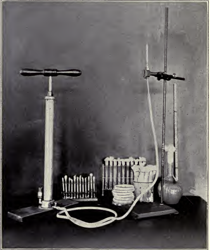
FIG. 32. Air pump, sand filters and other apparatus for bacteriological analysis of air.
