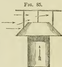
Emerson's Ejector.
