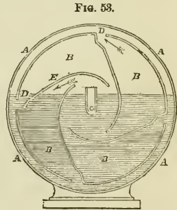
Meter for measuring the flow of Gas.
