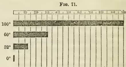
The length of the bars indicates the relative proportions of moisture that a cubic foot of air will hold at the different temperatures.
