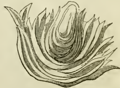
Starch grain ruptured by boiling.
