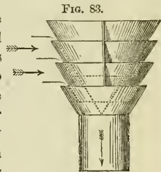
Emerson's Injector.
