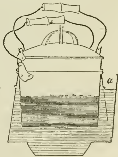
Section of a culinary bath: \alpha opening to introduce water.
