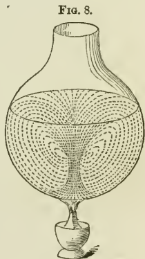
Currents produced in water by boiling.
