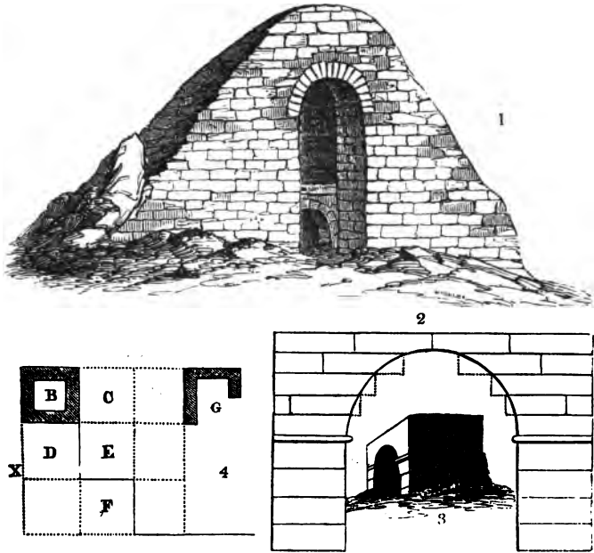
452. Fig. 1. Vaulted rooms and doorway of a crude brick pyramid at Thebes. 2. An imitation of an arch at Thebes. 3. Another at Abydos. 4. Mode of commencing a quarry.
