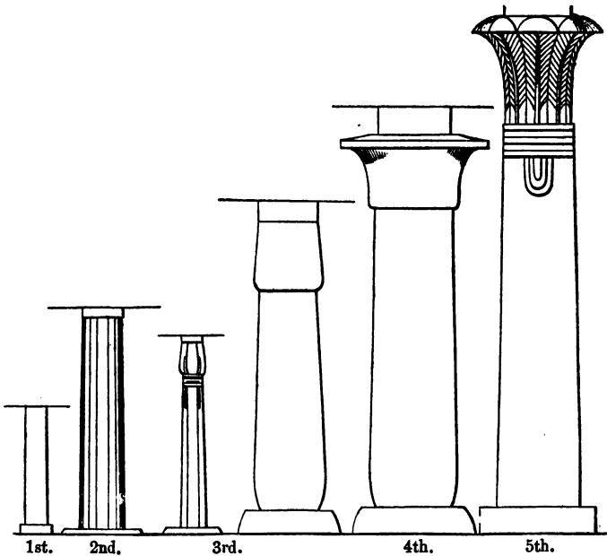
The five first orders of columns; to the same scale.
