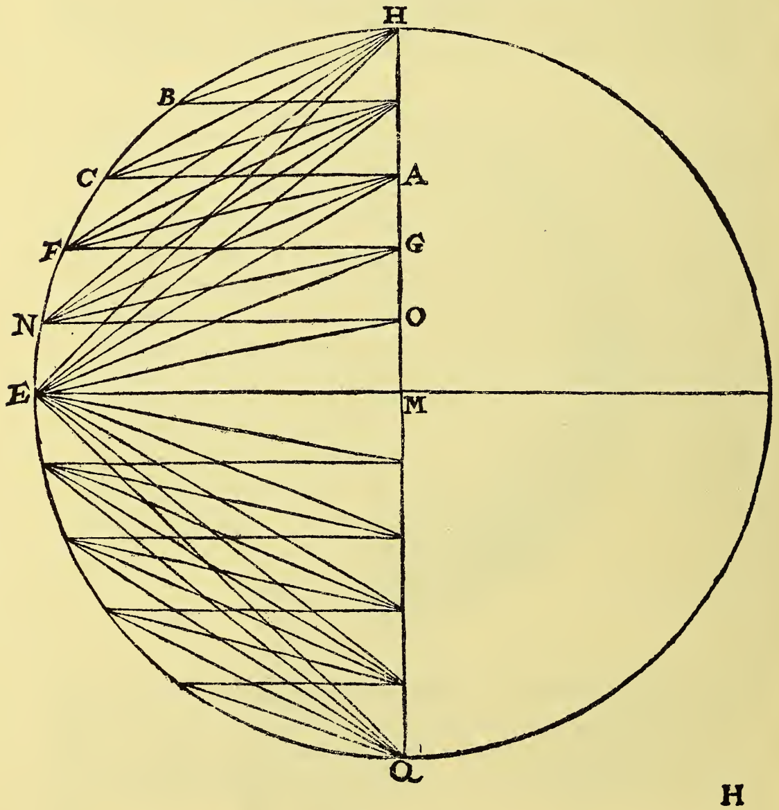
Diagramma magnetici vigoris, a plano Aequatoris in peripheriam terrelle aut telluris, fusi.
