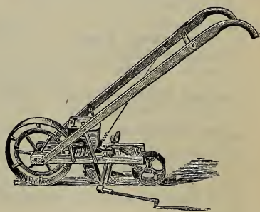
Fig. 28. The "New Model" Seed Drill
