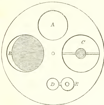
FIG. 2.—DIAPHRAGM. A, for direct light. B, for difficult test-objects. C, dark-ground illuminator. D, small aperture, with shutter E, having a small hole in it. The features presented by this condenser are,—that it is applicable for both high and low powers,
