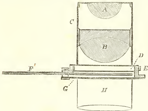
FIG. 1.—A, spot-lens, about \frac{1}{2} -inch focus. B, achromatic spot-lens, about \frac{1}{4} inch focus, placed at about the same distance as in a Kelnor eyepiece, in a tube C, screwed in a flat ring of metal D, which is supported on a flat plate G, secured by a holdfast E, allowing room between for a diaphragm F, to revolve freely on its axis, which is done by a screw passing through a holdfast into the plate G. H is a tube \frac{3}{8} -inch long for carrying polariscope.
