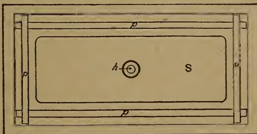
FIG. 3. Plan. Richardson Balanced Slide Valve.
