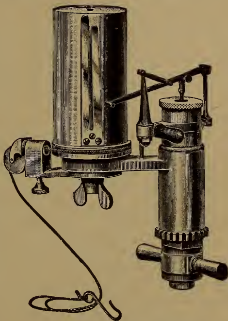
FIG. 1. The Thompson Indicator.
