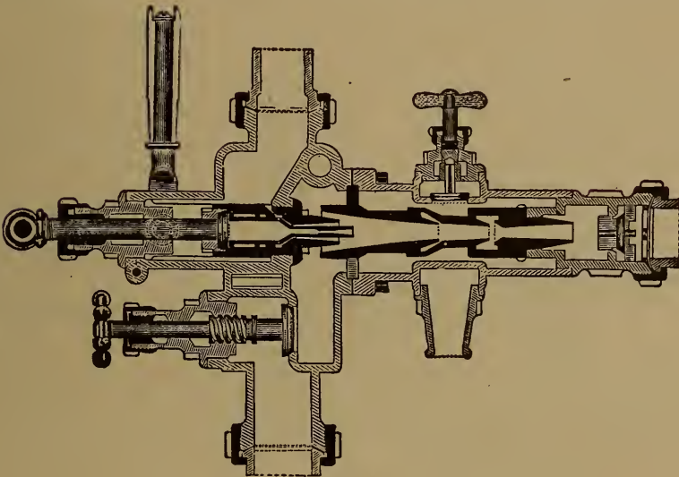
FIG. 12. The Ohio Locomotive Injector (Sectional View).
