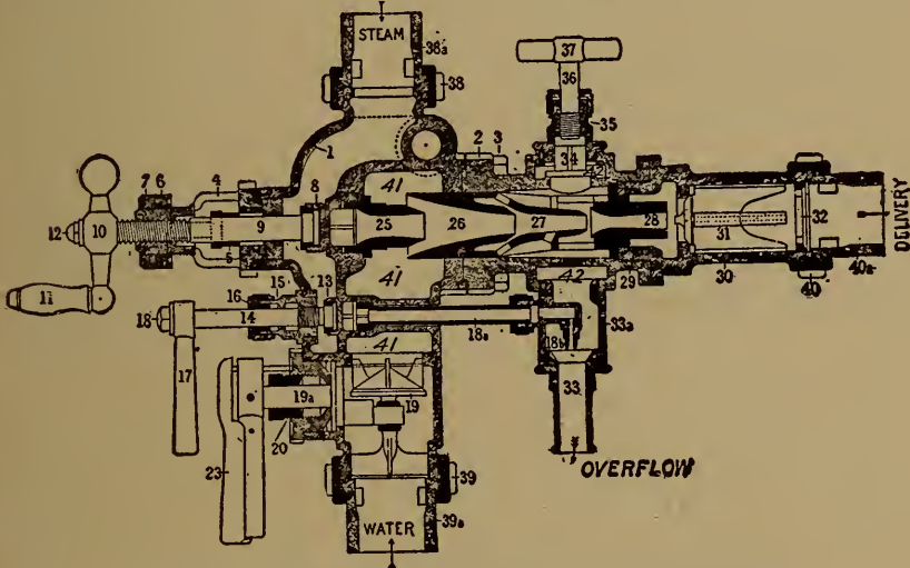
FIG. 6. Nathan "Monitor" Injector (Sectional View.)
