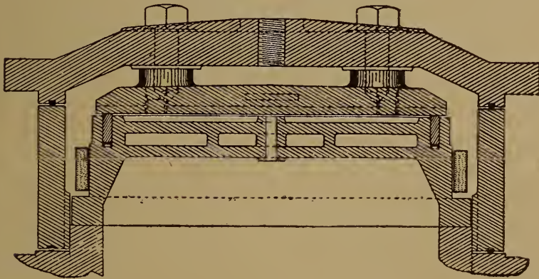
FIG. 6. Allen-Richardson Balanced Slide Valve. Transverse Section.
