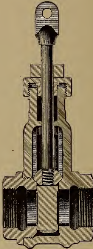
Johnstone Blow-Off Valve.
