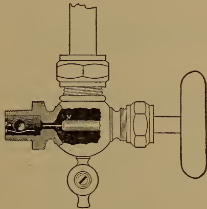
FIG. 3. Crosby Safe Water Gauge.
