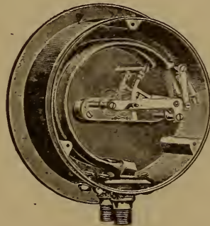
FIG. 27. Sectional View.
