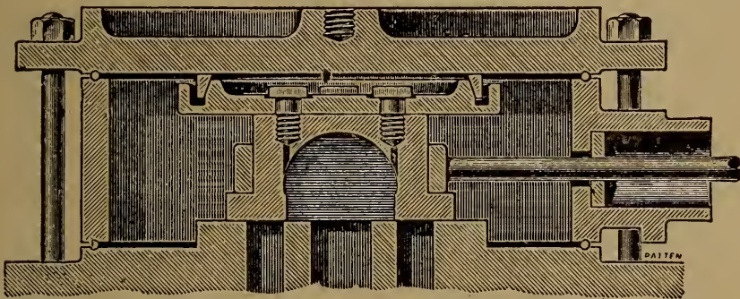
FIG. 1. The American Balance Valve. Single Disc Longitudinal Section.
