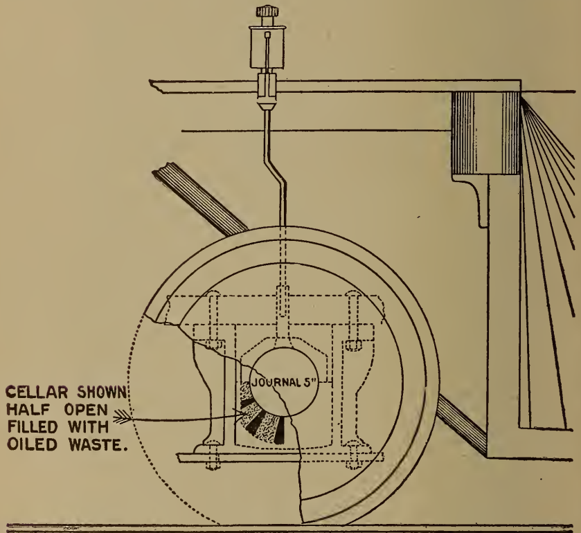
FIG. 1. Acme Engine Truck Cellar and Oil Cup.
