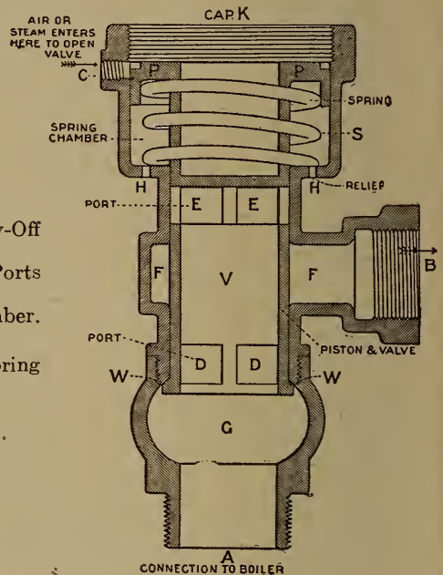
Climax Blow-Off Cock.
