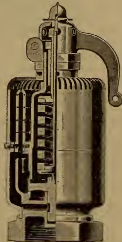
FIG. 11. Sectional View with Lever. Crosby Muffled Locomotive Pop Safety Valves.
