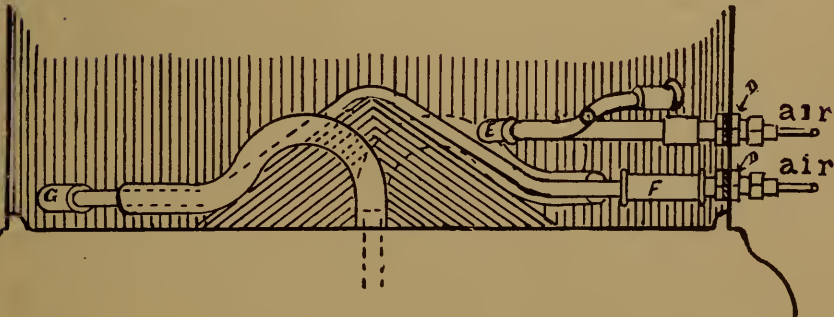
FIG. 3 The Mudd Track Sander. (Side View.)
