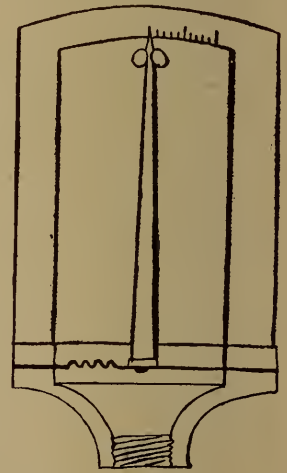
FIG. 5. Early Form of Diaphragm Gauge.
