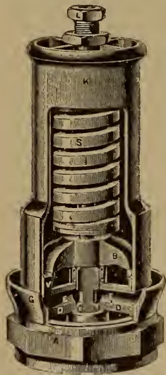
FIG. 7. Sectional View Crosby Locomotive Pop Safety Valve.
