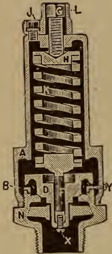
FIG. 7. Special Automatic Relief Valve.
