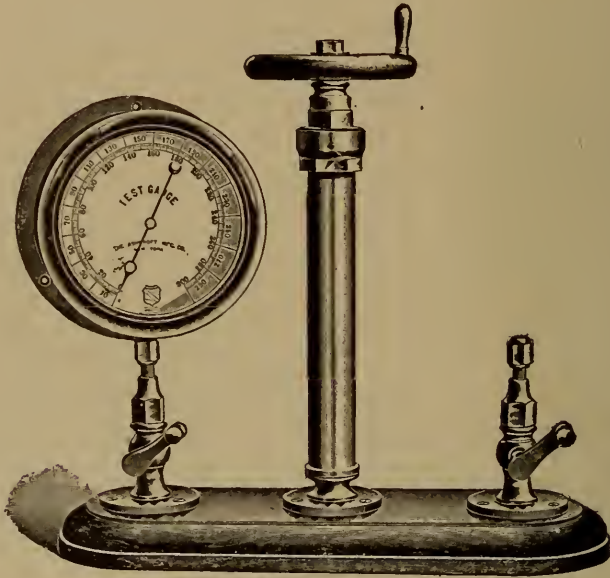
FIG. 39. Ashcroft Test Gauge.
