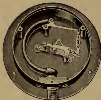
FIG. 10. Crosby Single Tube Gauge.
