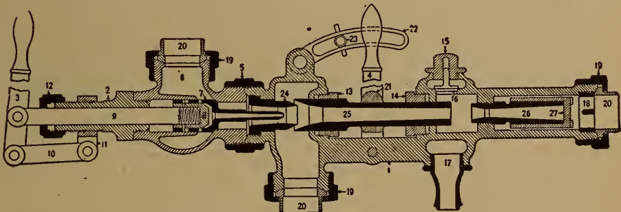
FIG. 14. Little Giant Locomotive Injector. (Sectional View.)
