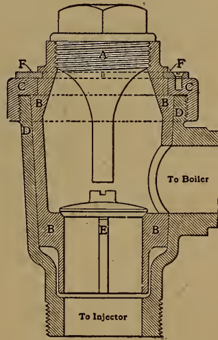
FIG. 3. Combined Check and Stop Valve.
