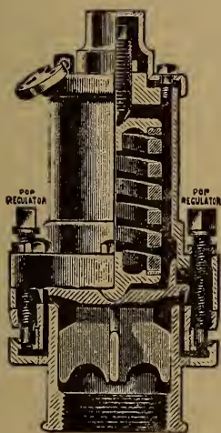
FIG. 15. Ashton Open Pop Safety Valve.
