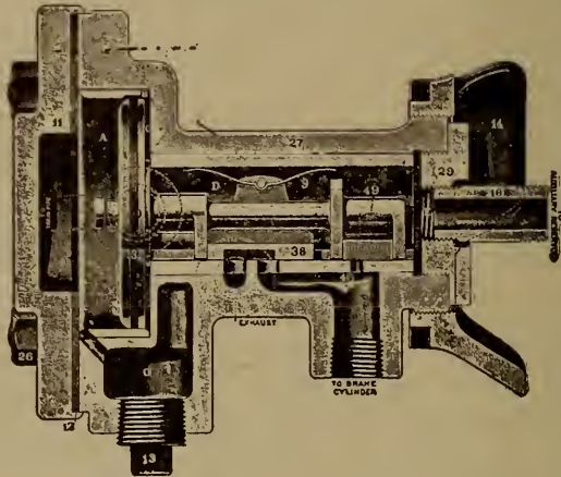
FIG. 1. Plain New York Triple Valve.
