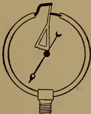
FIG. 3. Double Bourdon Spring Gauge.
