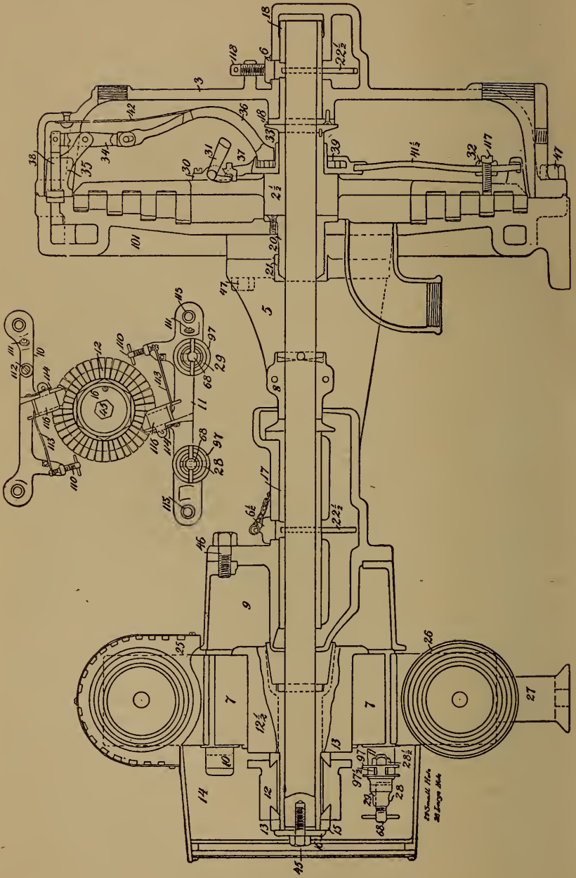
FIG. 2. Electric Headlight Engine.
