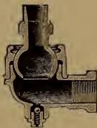
FIG. 2. Sectional View Moran Flexible Joint.
