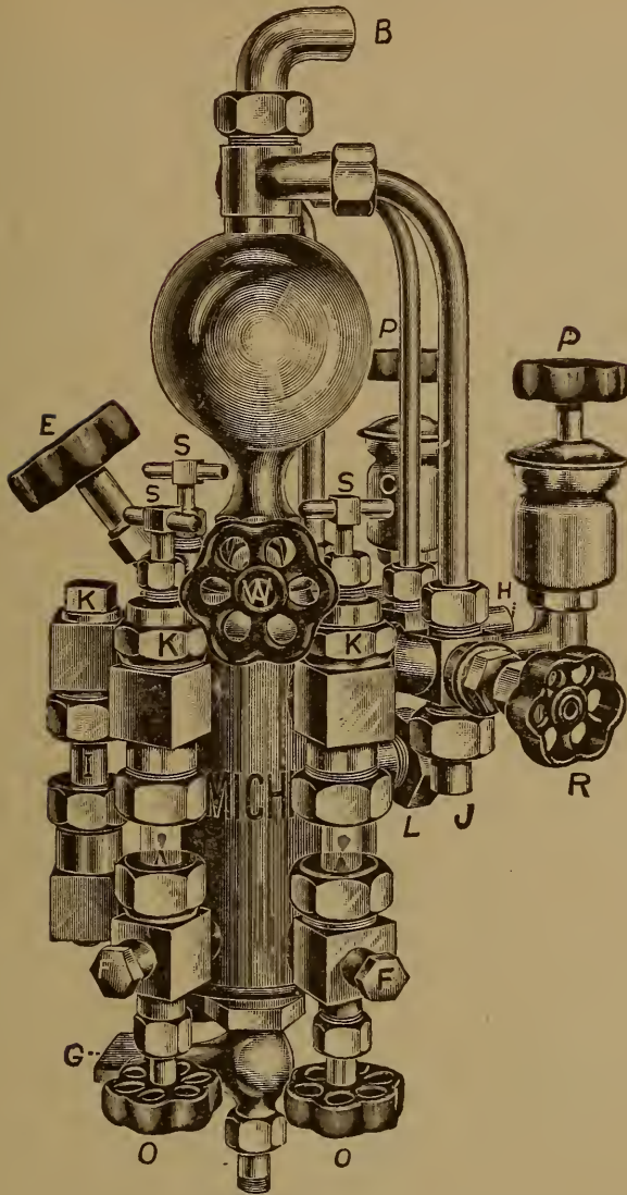
FIG. 1. Michigan Sight Feed Lubricator.
