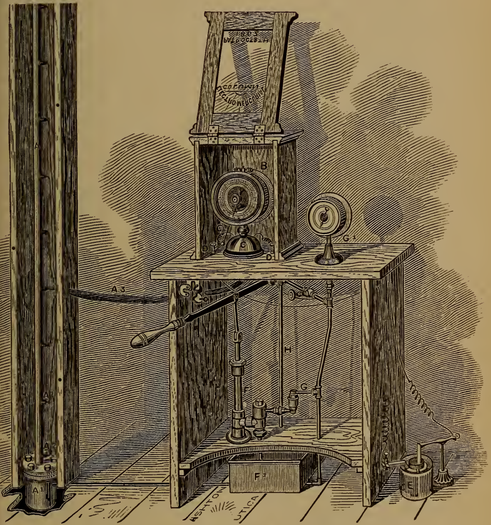
FIG. 1. Electro-Mercurial Gauge Tester.
