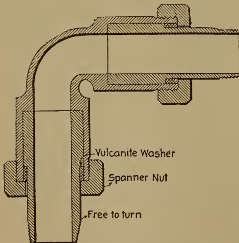
FIG. 1. Section of Swivel Joint.
