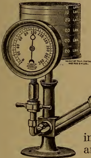
FIG. 38. Crosby Test Gauge.
