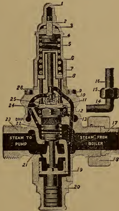
FIG. 1. Mason Air Brake Pump Regulator.
