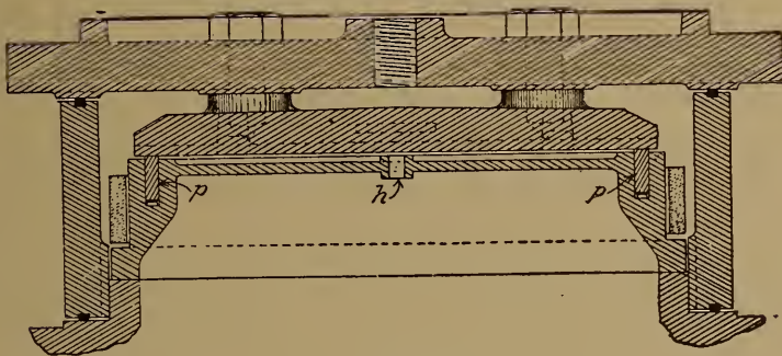
FIG. 2. Richardson Balanced Slide Valve. Transverse Section.
