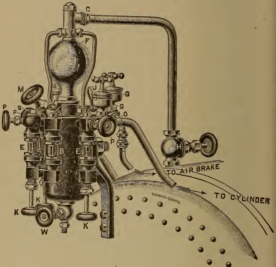
FIG. 1. Seibert Triple Sight Feed Lubricator.
