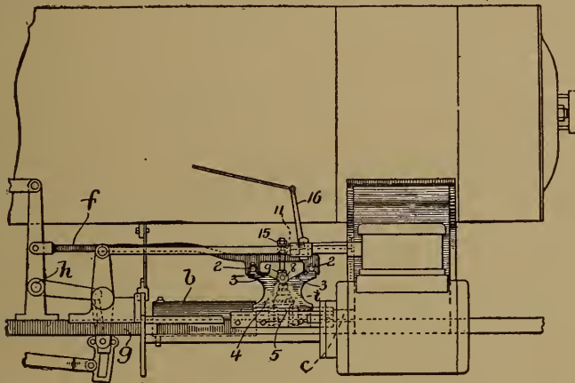
FIG 1. Huff Automatic Variable Exhaust. (Side View.)
