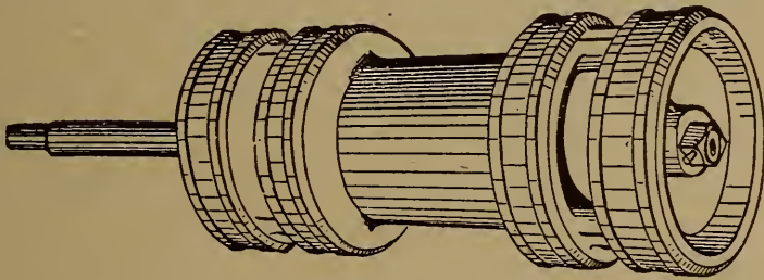
FIG. 1. Piston Valve for Baldwin Four-Cylinder Compound Locomotives.
