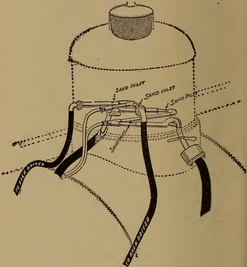
FIG. 1. The Mudd Track Sander.
