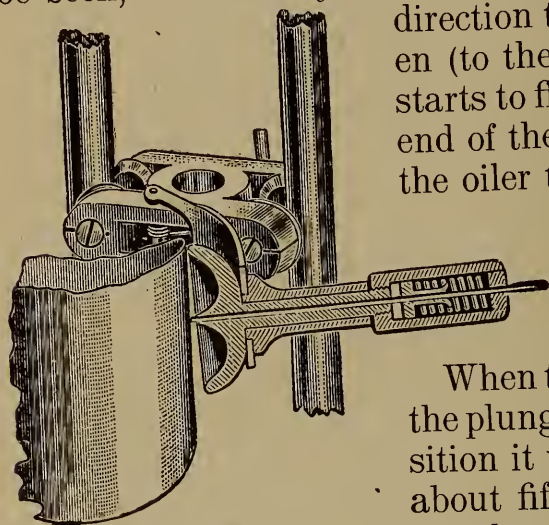
FIG. 5. Pencil Mechanism Boyer Speed Recorder.
