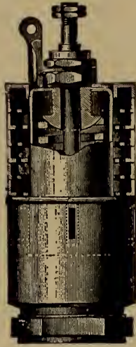
FIG. 12. Flat Top Muffler Valve with Lever.
