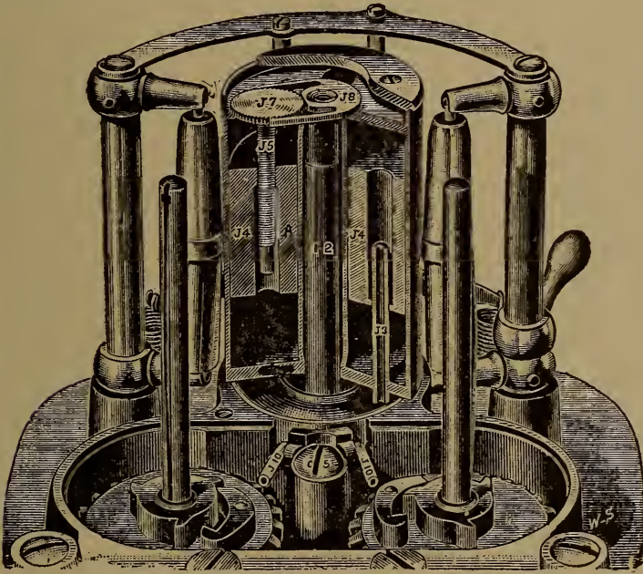
FIG. 4. Oiler—Boyer Speed Recorder.
