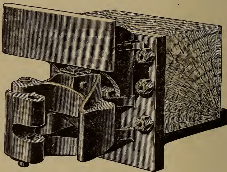
FIG. 1. Talbot Automatic Coupler for Tenders.
