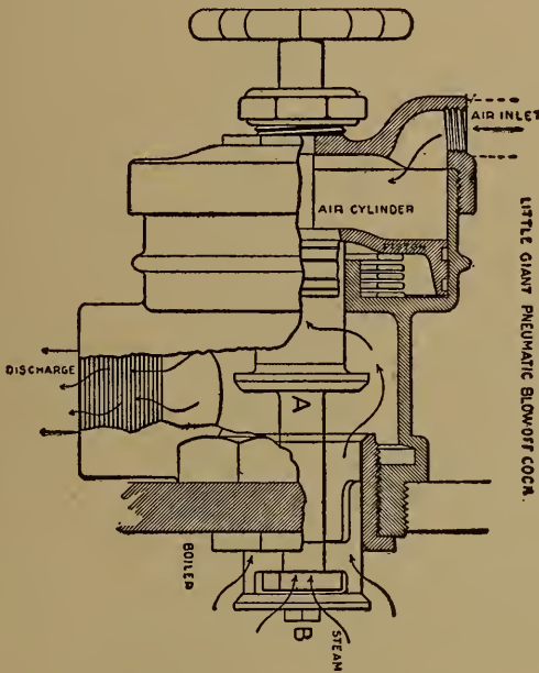
Little Giant Blow-Off Cock.
