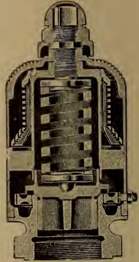
FIG. 5. Sectional View.
