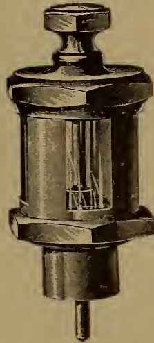
FIG. 4. Locomotive Bearing Cup for Connecting Rods.
