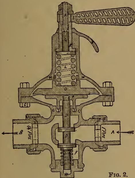
FIG. 2. Gold Pressure Regulator.
