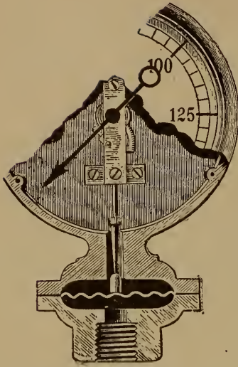
FIG. 4. Early Form of Diaphragm Gauge.
