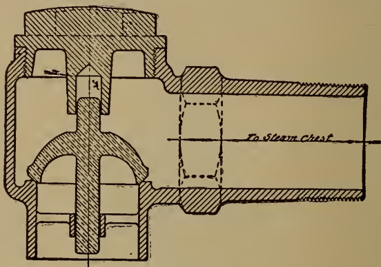
FIG. 4. Steam Chest Vacuum or Air Relief Valve.
