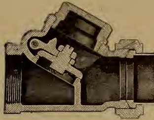
SECTIONAL VIEW. FIG. 1. Swing Intermediate or Line Check.
