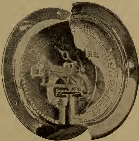
FIG. 23. Utica Locomotive Steam Gauge.
