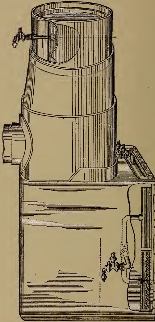
FIG. 1. Hornish Mechanical Boiler Cleaner.
