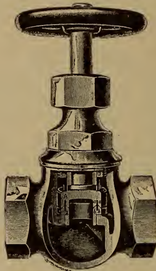
FIG. 2. Crosby Spring-Seat Valve.
