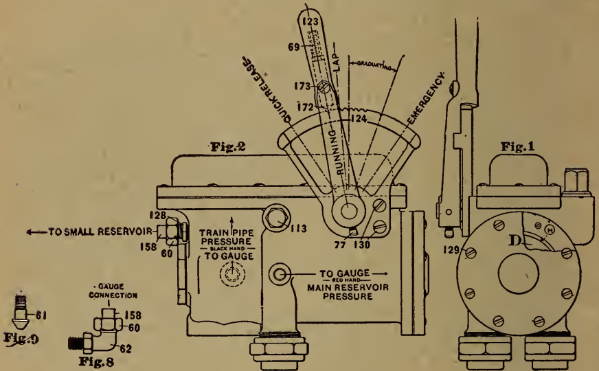
Positive Discharge Engineer's Brake Valve. New York Air Brake Co.
