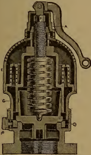
FIG. 1. The Coale Pop Safety Valve and Muffler.
