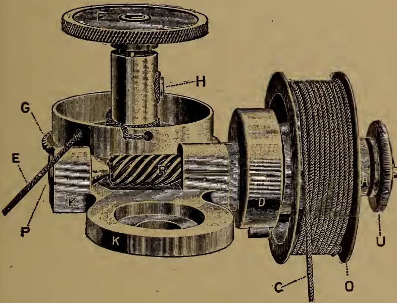
FIG. 2. Ashcroft Reducing Wheel.
