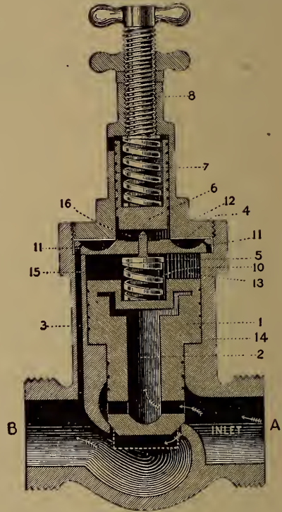
FIG. 3. Climax Steam Pressure Regulating Valve.
