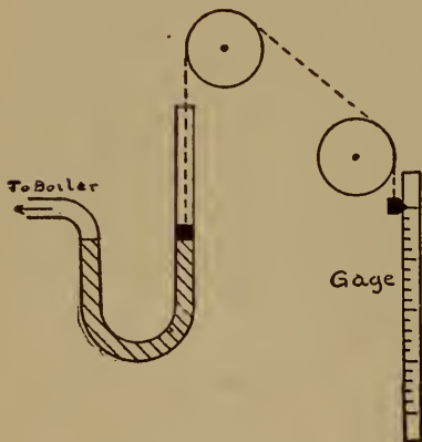
FIG. A. Mercury Column and Gauge.
