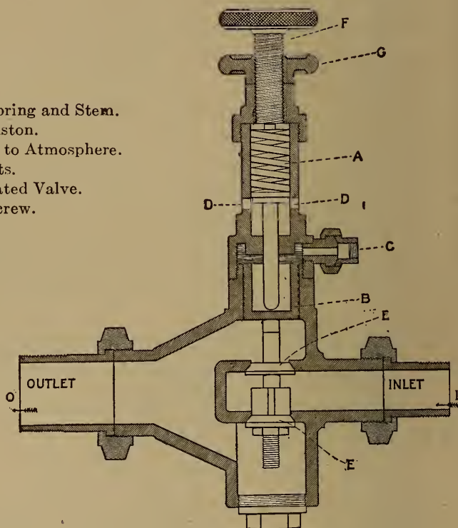
FIG. 4. Eclipse Reducing Valve.
