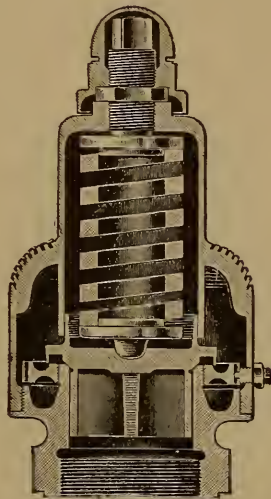
FIG. 3. Sectional View.
