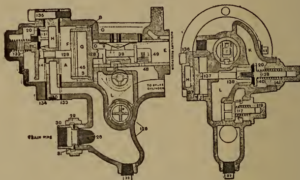
FIG. 2. New York Quick Action Triple Valve.
