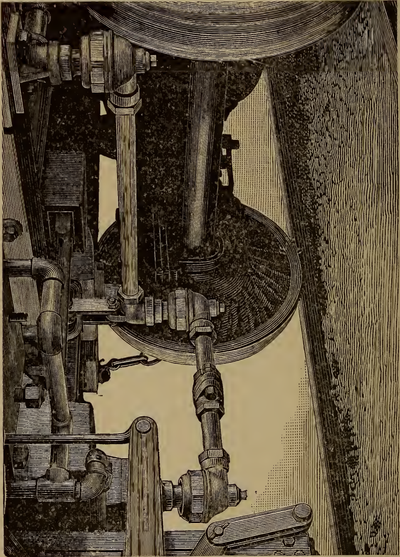
FIG. 1. Moran Flexible Joint.
