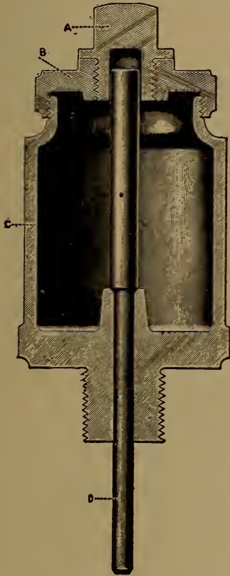
FIG 3. Spindle Feed Rod Cup.
