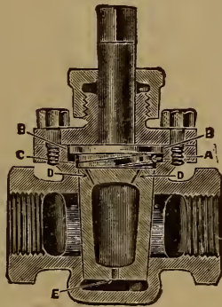
FIG 3 Homestead Straight-Way Valve.
