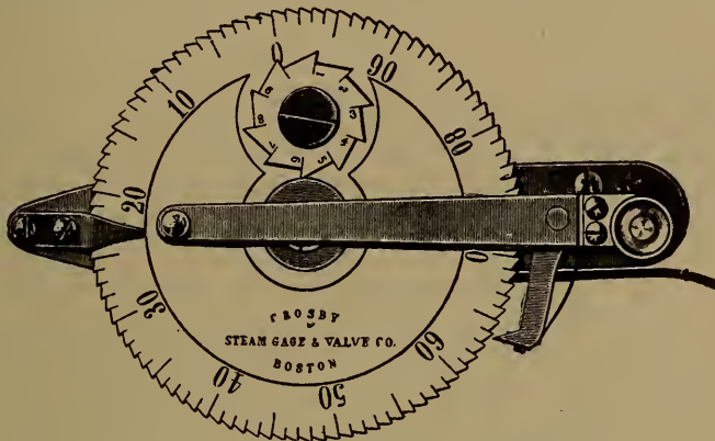
FIG. 1. Crosby Locomotive Counter.
