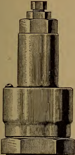
FIG. 8. External View. Crosby Plain Locomotive Pop Safety Valves.
