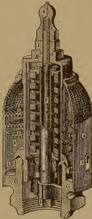
FIG. 6. Meady Muffled Locomotive Pop Safety Valve.
