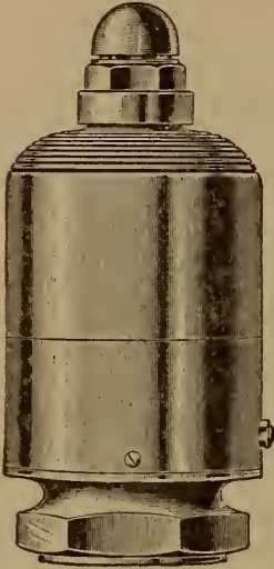
FIG. 4. Exterior View.
