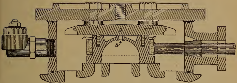
FIG. 1. Richardson Balanced Slide Valve. Longitudinal Section.
