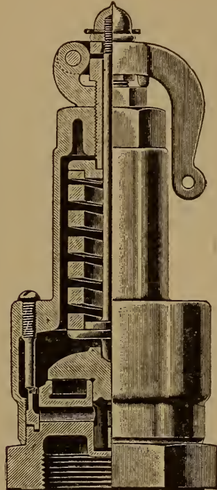
FIG. 9. Sectional View with Lever. Crosby Plain Locomotive Pop Safety Valves.
