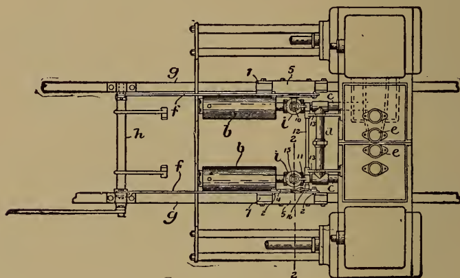
FIG. 2. Huff Automatic Variable Exhaust. (Plan View.)
