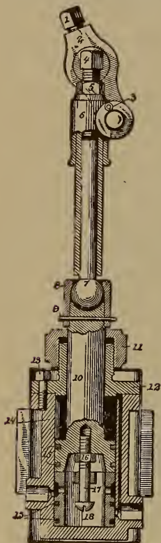
FIG. 3. Gollmar Bell Ringer. (Sectional View.)
