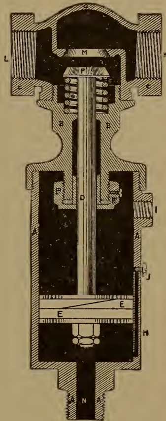
FIG. 2. Huff Automatic Steam Blower. (Sectional View.)
