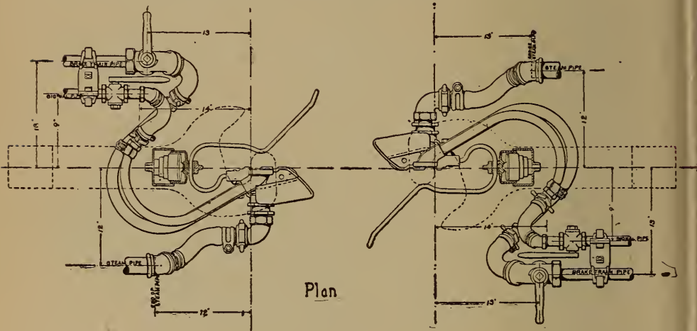
FIG. 1. Automatic Air and Steam Coupler.
