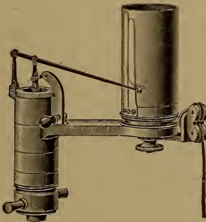
FIG. 1. The Crosby Indicator.
