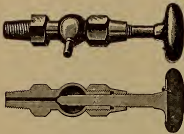
FIG. 4. Regrinding Locomotive Gauge Cock.
