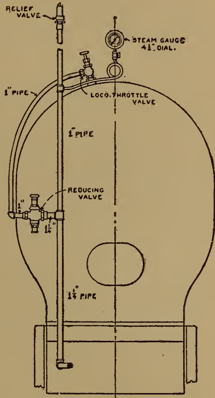
FIG. 8. Location of Steam Heating Cab Attachments.
