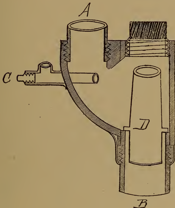
FIG. 1. A-B-C Track Sander.
