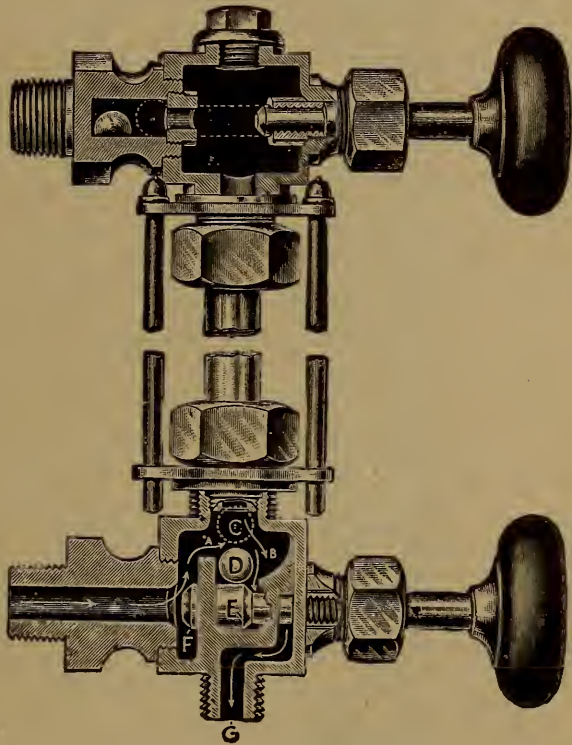
FIG. 1. Pemberthy Automatic Water Gauge.
