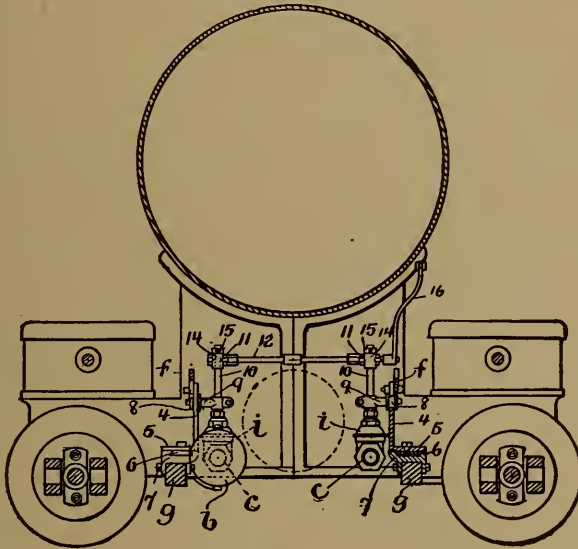
FIG. 3. Huff Automatic Variable Exhaust. (Front View.)
