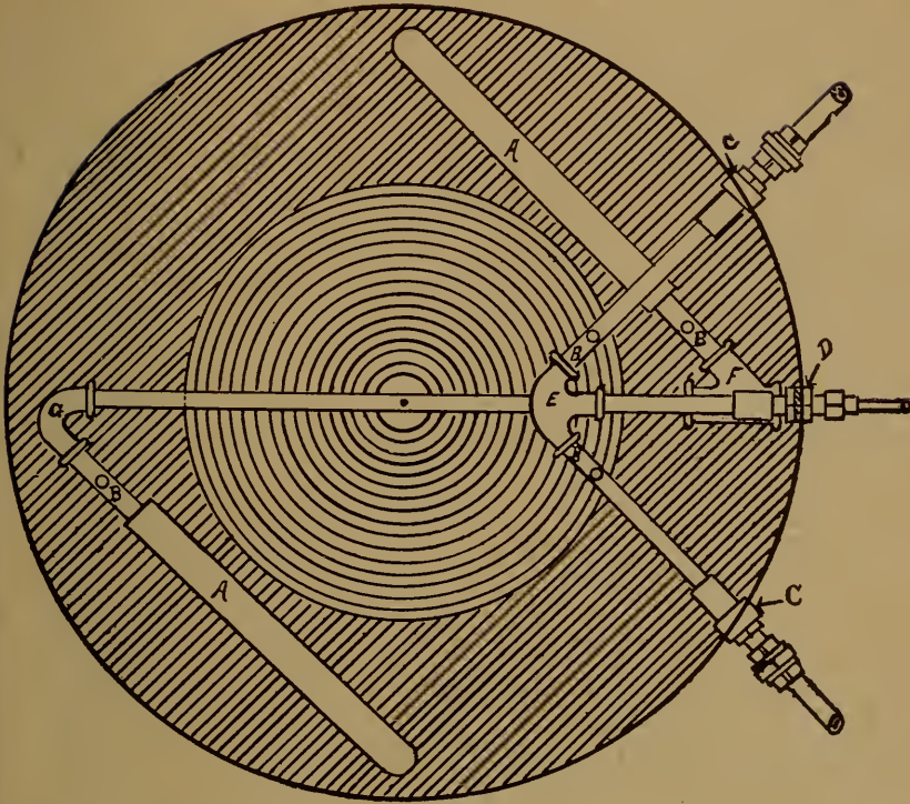
FIG. 2. The Mudd Track Sander. (Plan View.)
