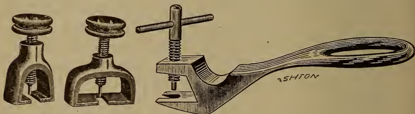
FIG. 35. FIG. 36. Gauge Hand or "Pointer" Pullers.
