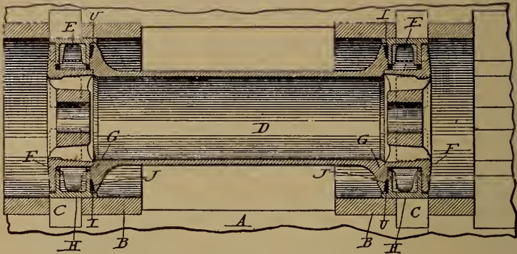
FIG. 2. Locomotive Piston Valve.
