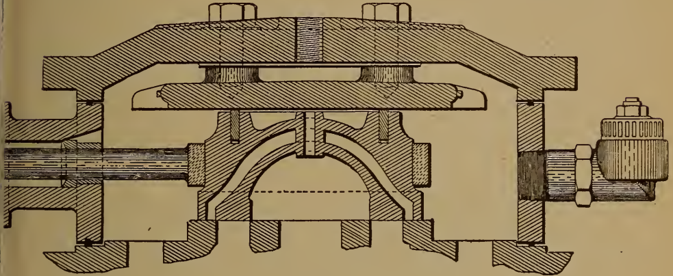
FIG. 5. Allen-Richardson Balanced Slide Valve. Longitudinal Section.
