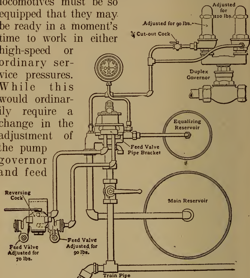
FIG. 3. High-Pressure Controlling Apparatus.
