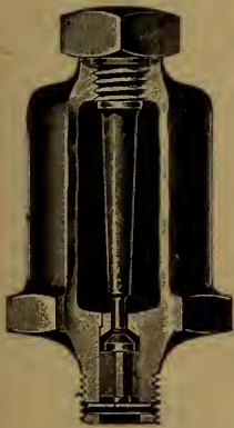
FIG. 1. Injector Oil Cup. (Sectional View.)
