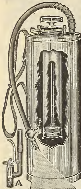
order and will last for years. Weighs about 6 lbs. Each machine is packed in a case complete, comprising 4 tubes, 6 nozzles, 2 straps and oil can. The reservoir holds 4 lbs. of Paris Green (or over a quart of powder). Is made in best manner, of tin, iron, steel and brass. We give this sprayer our unqualified endorsement. Price, $8.00.
