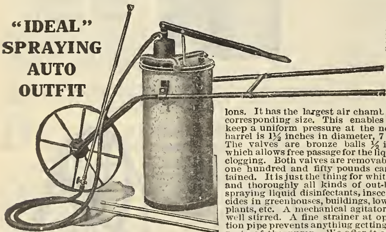
provided and the pump has the following equipment: 10 ft. 3/4 in. Pressure Hose; 10 ft. Pipe Extension, in three pieces; 1 T Handle Shut-off Cock; 1 "IDEAL" Self-cleaning Nozzle. Shipping weight, crated, 60 pounds. Price, $17.00.
