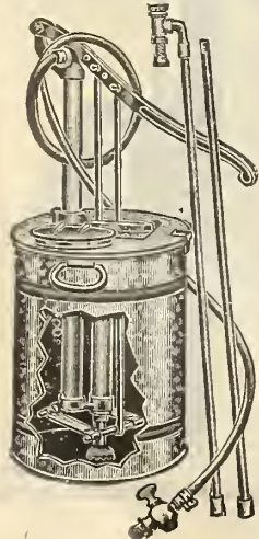
provided and the pump has the following equipment: 10 ft. 3/4 in. Pressure Hose; 10 ft. Pipe Extension, in three pieces; 1 T Handle Shut-off Cock; 1 "IDEAL" Self-cleaning Nozzle. Shipping weight, crated, 60 pounds. Price, $17.00.
