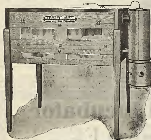
No. 400 Banta Incubator. Absolutely Fire-proof, Packed With Asbestos. Lamp Enclosed in a Metal Case.
