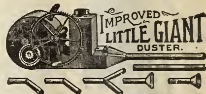
For Farm, Garden, Vineyard, Tobacco Fields. Dust potato vines as fast as you walk, two rows at a time. Reservoir holds nearly a quart of powder. Machine weighs 6 lbs. One packed in a case complete, 3 tubes, 5 nozzles and strap. Our Improved Little Giant differs but slightly from our Champion Duster except in size, being a trifle smaller. Price, $5.50.
