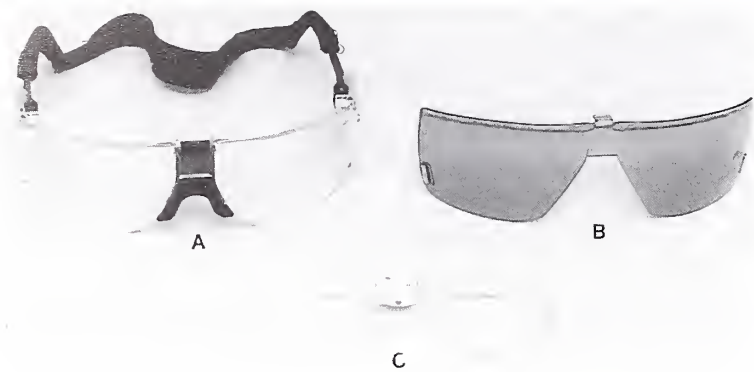
Fig. 26-7. Definitive eye armor (BLPS) components. (a) Polycarbonate eye armor. (b) Laser protective attachment. (c) Corrective lens carrier.
