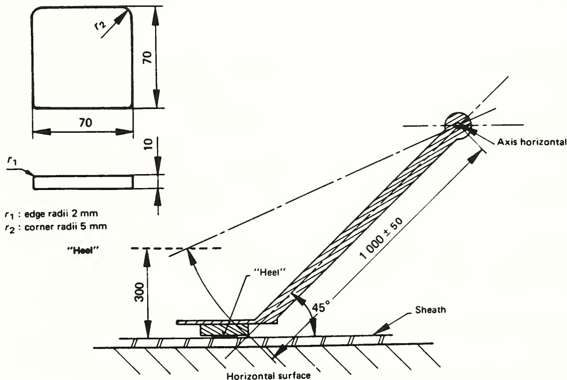
FIGURE 8.5 Crushing test
