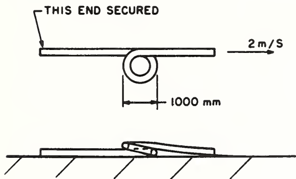
FIGURE 8.4 Kinking test
