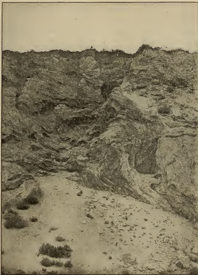
FIG. 8. Example of wind erosion on south fork of Rio Chico, Patagonia, from a photograph by the author.
