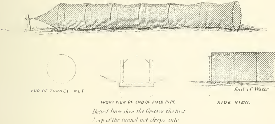
TUNNEL NET. Scale \frac{1}{4} inch to a foot.
