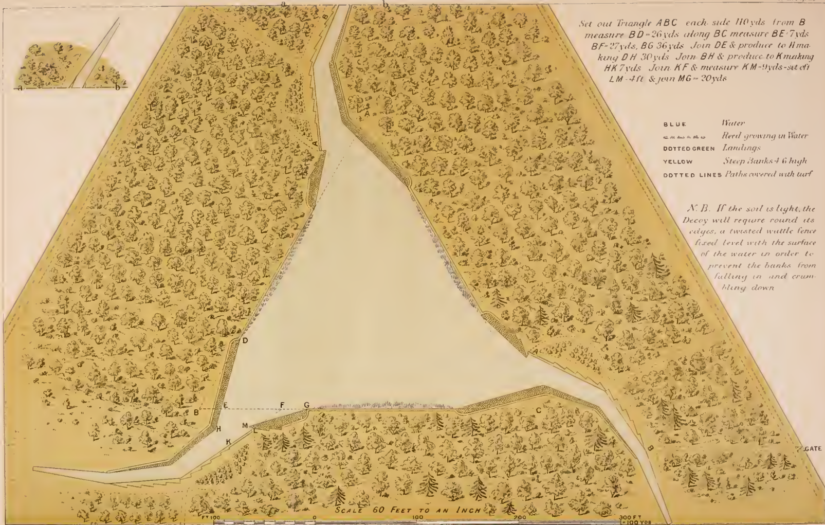
PLAN OF A THREE PIPE DECOY.
