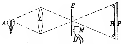
FIG. 23.—Apparatus for testing focal plane shutter speed throughout the travel of the curtain.
