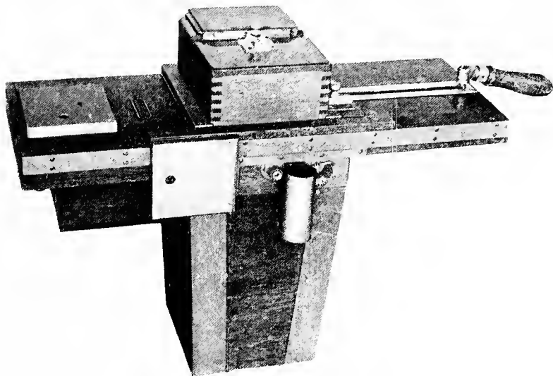
FIG. 45.—English C type aerial camera.
