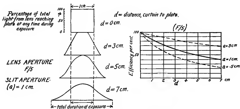
FIG. 22.—Characteristics of focal plane shutter.
