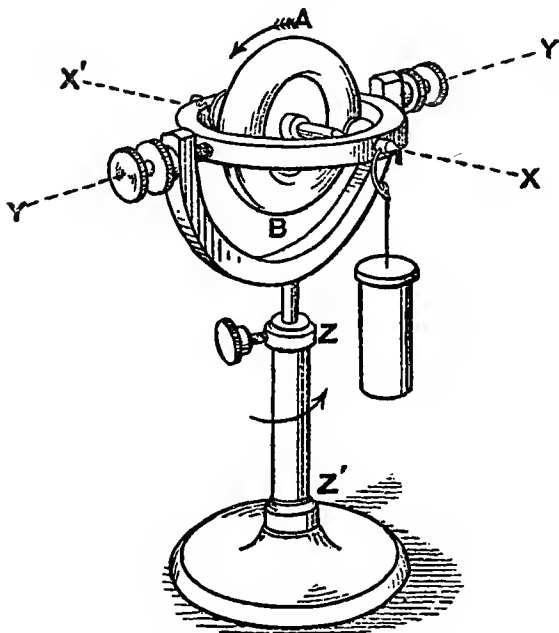
FIG. 79.—Diagram of simple gyroscope.
