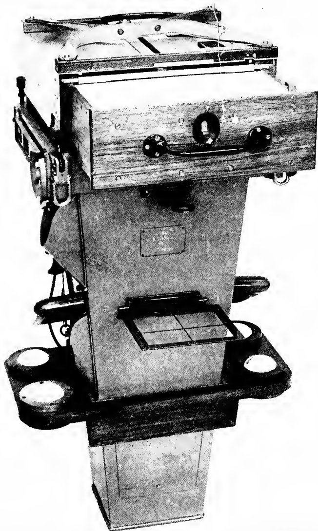
FIG. 40.—50 centimeter deMaria hand operated camera on tennis ball mounting.
