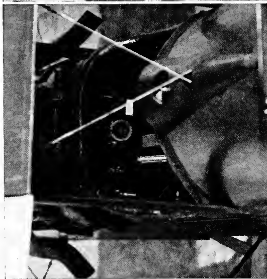
FIG. 2.—Forward cockpit of DeHaviland 4, showing instrument board.
