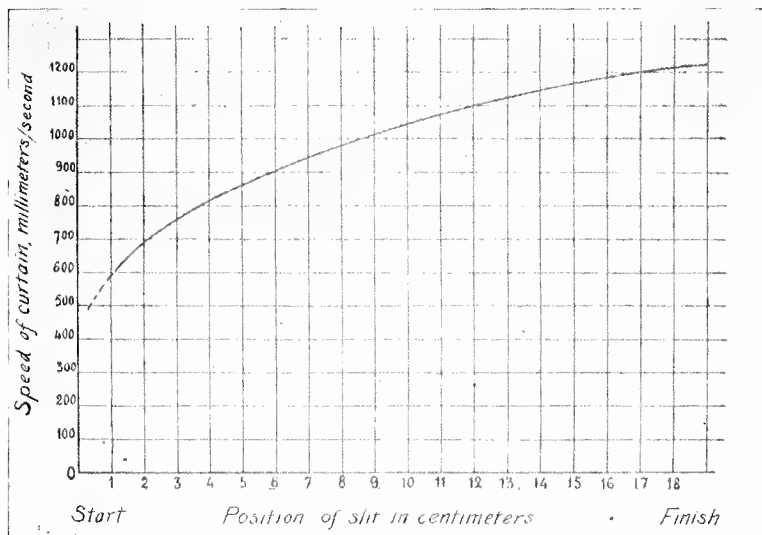
FIG. 24.—Performance of Kloplic shutter.
