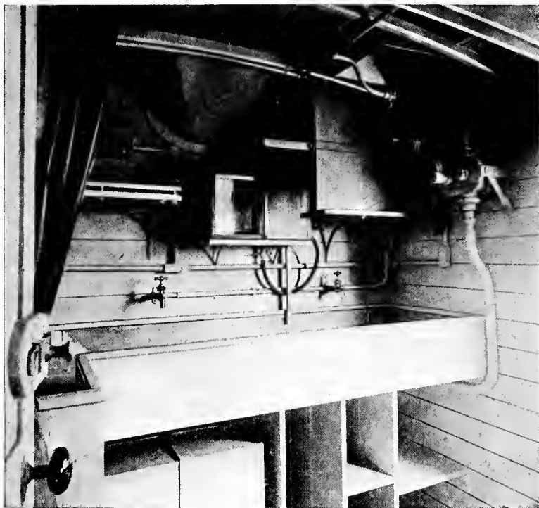
FIG. 114.—Interior of photographic trailer, developing room.
