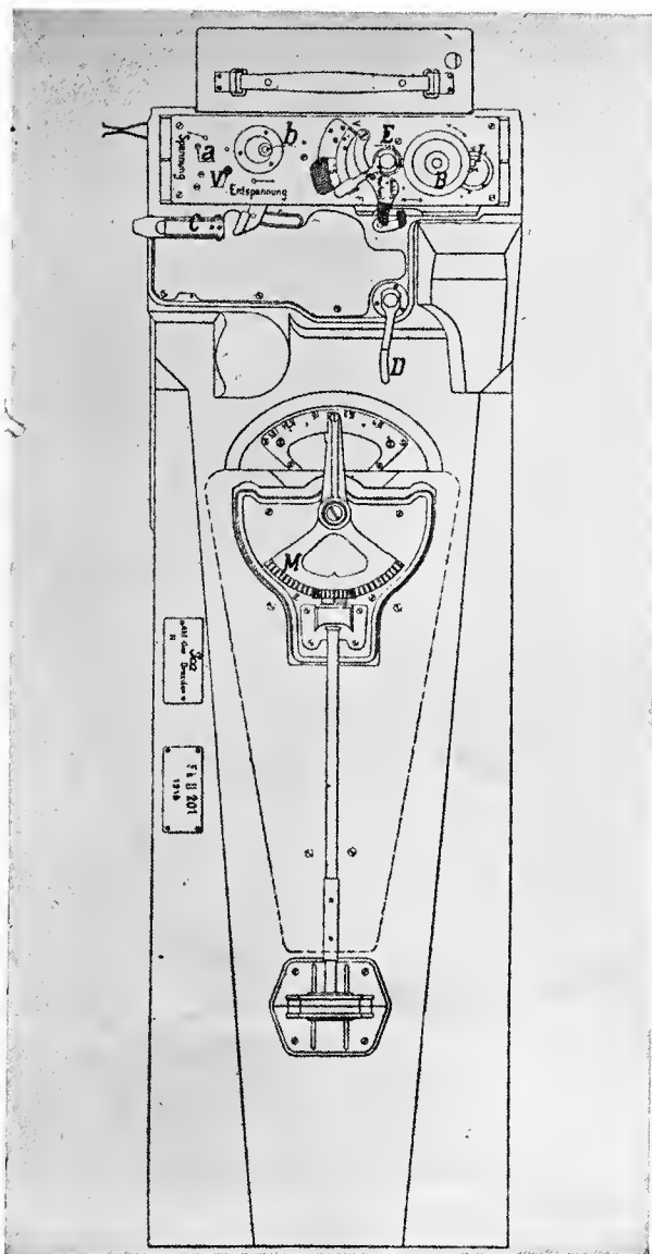
FIG. 43.—Diagram of German 50 centimeter camera.
