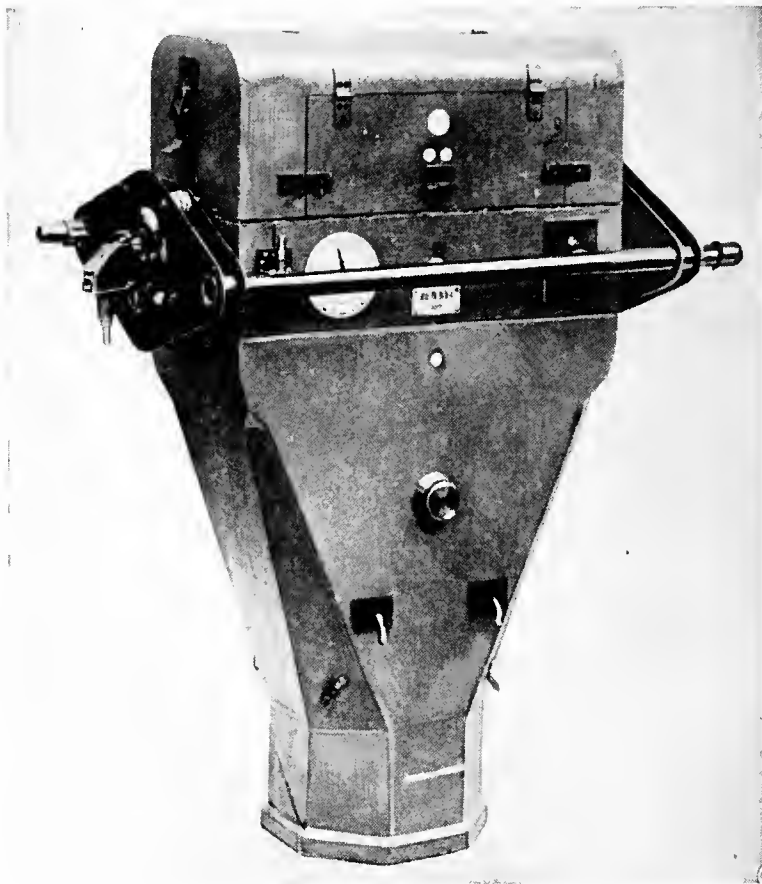
FIG. 61.—German automatic film camera.
