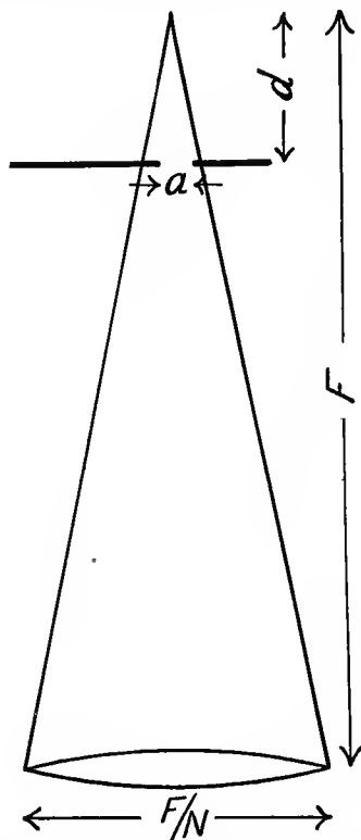
FIG. 21.—Calculation of focal plane shutter efficiency.
