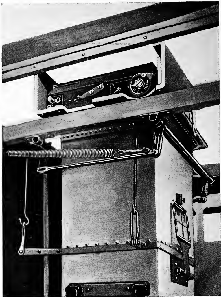
FIG. 86.—French spring and bell crank suspension.
