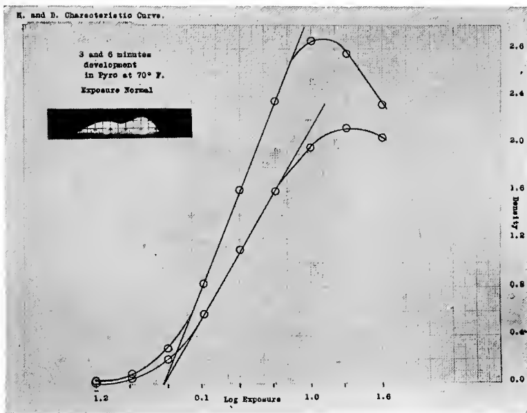
FIG. 103.—Typical characteristic curves of photographic plate.
