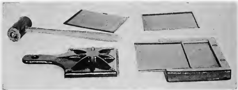
FIG. 35.—Apparatus for straightening plate sheaths.
