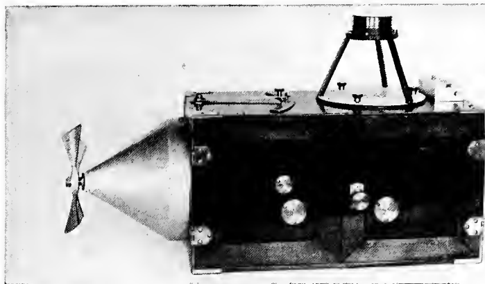
FIG. 57.—English type "F" (Williamson) automatic film camera.
