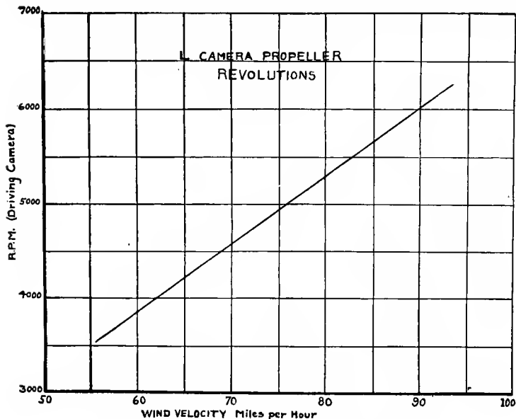
FIG. 67.—Relation between air speed and propeller revolutions.
