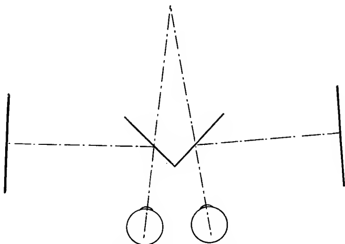
FIG. 152.—Diagram of mirror stereoscope.
