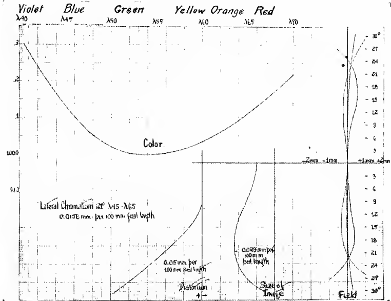
FIG. 16.—Chart recording measurements of lens characteristics.
