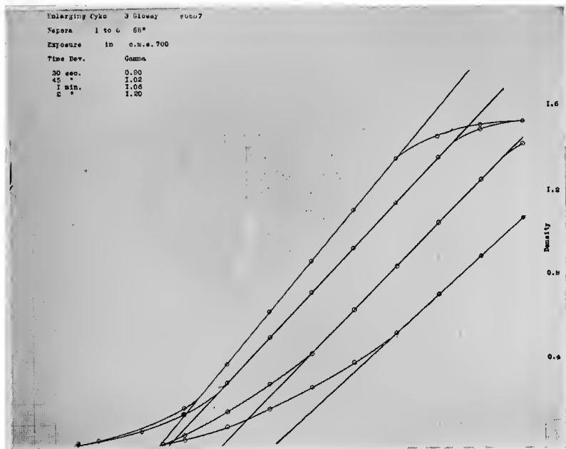
FIG. 111.—Characteristic curves of gas-light paper.
