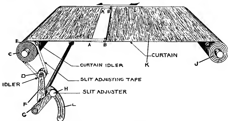
FIG. 28.—Variable aperture curtain developed in U. S. Air Service, and used in American deRam, and "K" type automatic film cameras.
