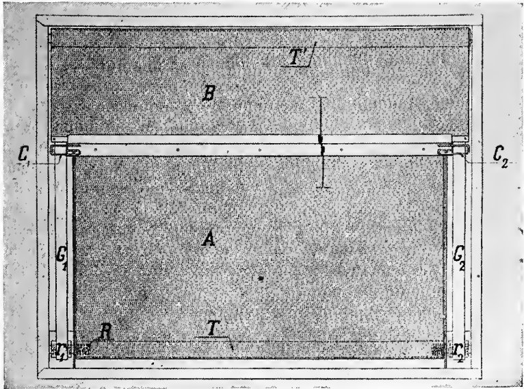
FIG. 29.—Mechanism of Kloplic variable aperture self-capping shutter.
