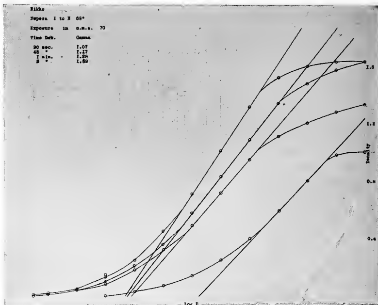
FIG. 110.—Characteristic curves of bromide paper.
