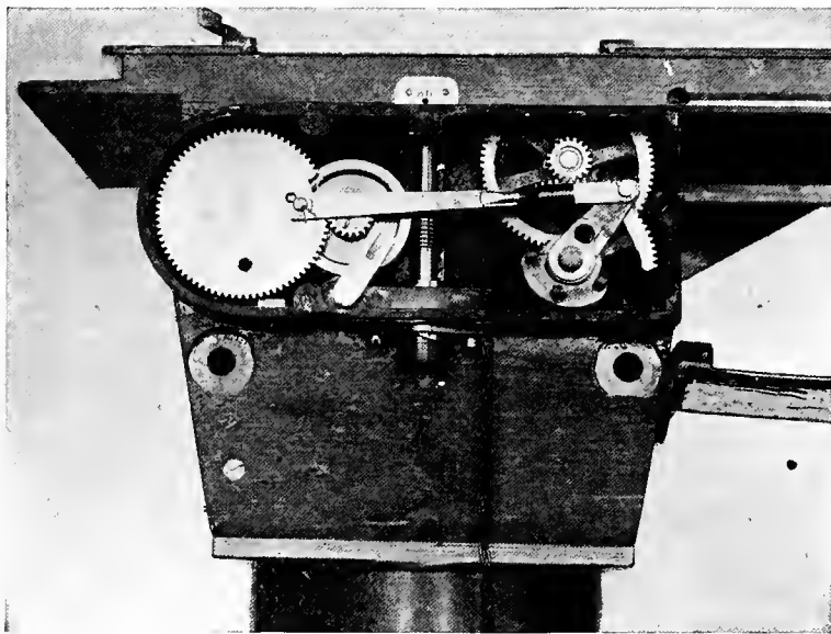
FIG. 51.—Mechanism of "L" camera.
