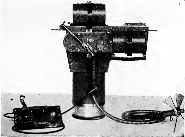
FIG. 50.—American model, English "L" type semi-automatic camera.
