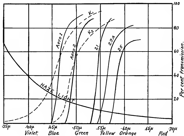
FIG. 106.—Characteristics of various filters.
