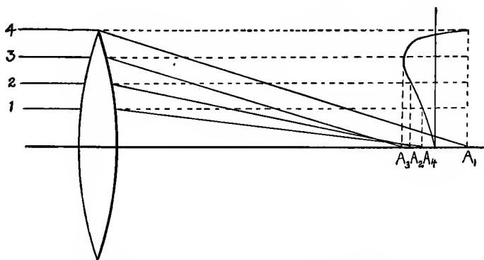
FIG. 12.—Diagrammatic representation of spherical aberration.
