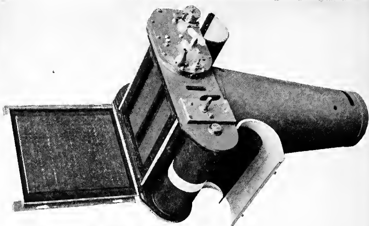
FIG. 65.—Type "K" camera, open, showing suction plate.
