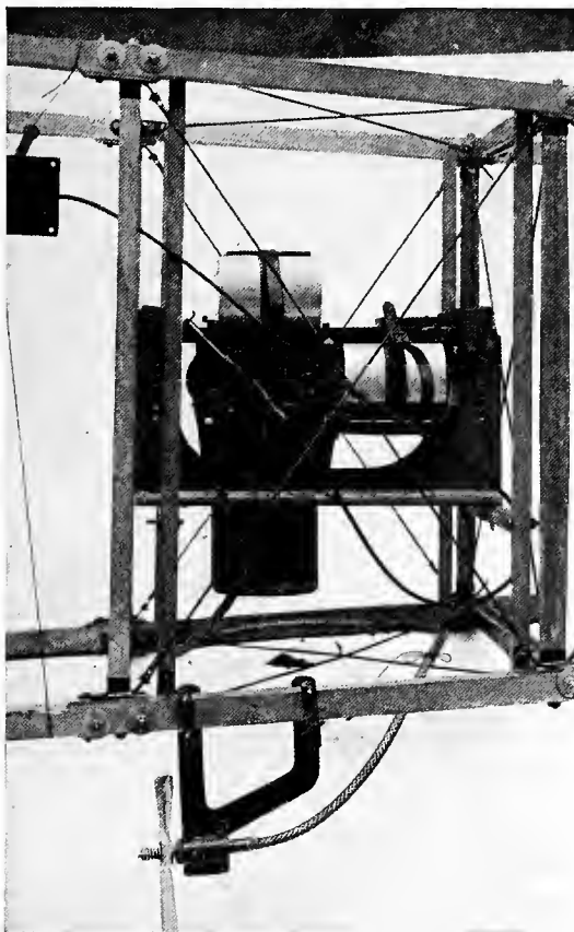
FIG. 88.—“L” camera and cradle mount in skeleton DeHaviland 4 fuselage, side view.
