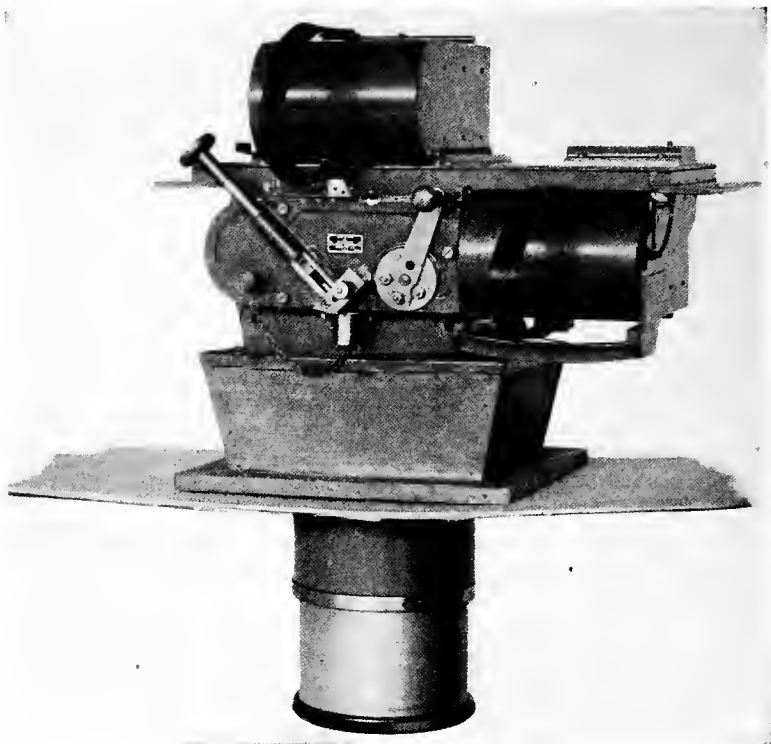
FIG. 82.—"L" camera in floor mounting.
