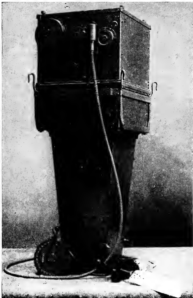
FIG. 54.—French model deRam automatic plate camera.
