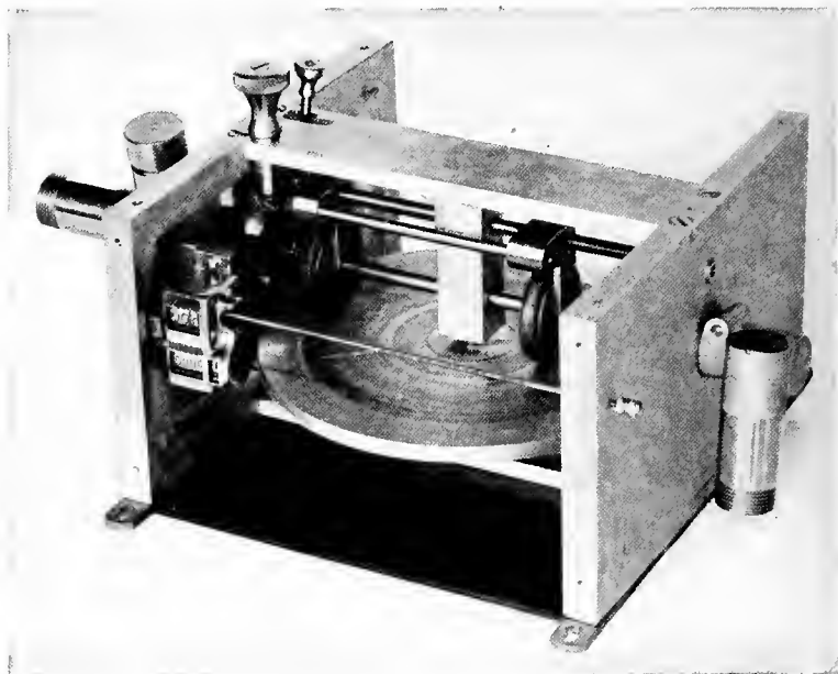
FIG. 68.—Friction disc speed control.
