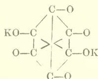
Rhodizonate of potassium or potassium dioxydichinoyl.
