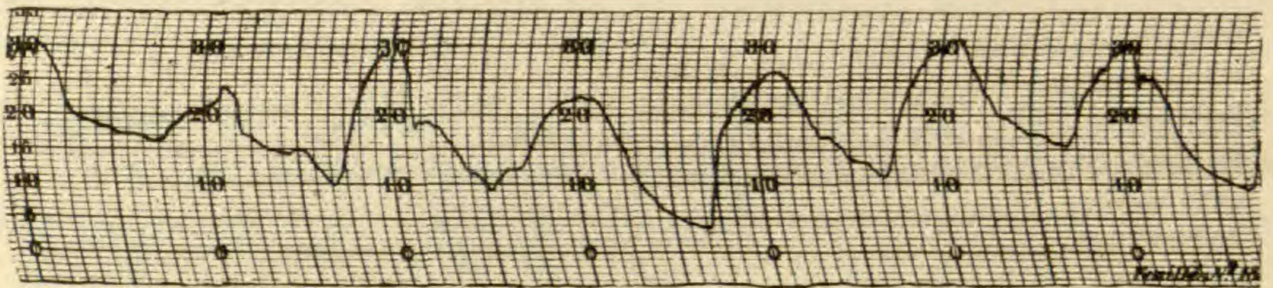
FIG. 3.—Temperature record of the air for the week July 2-9, 1906, taken in the sedge zone at First Sister Lake; the highest was 31^{\circ} C., the lowest 3.5^{\circ} C.; this occurred about 5 A.M., July 6.
