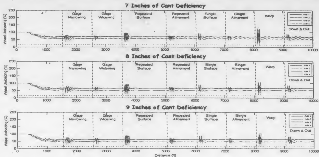
Figure 3. V_{min} , Acela Coach, 160 m.p.h., 31-foot Perturbations
