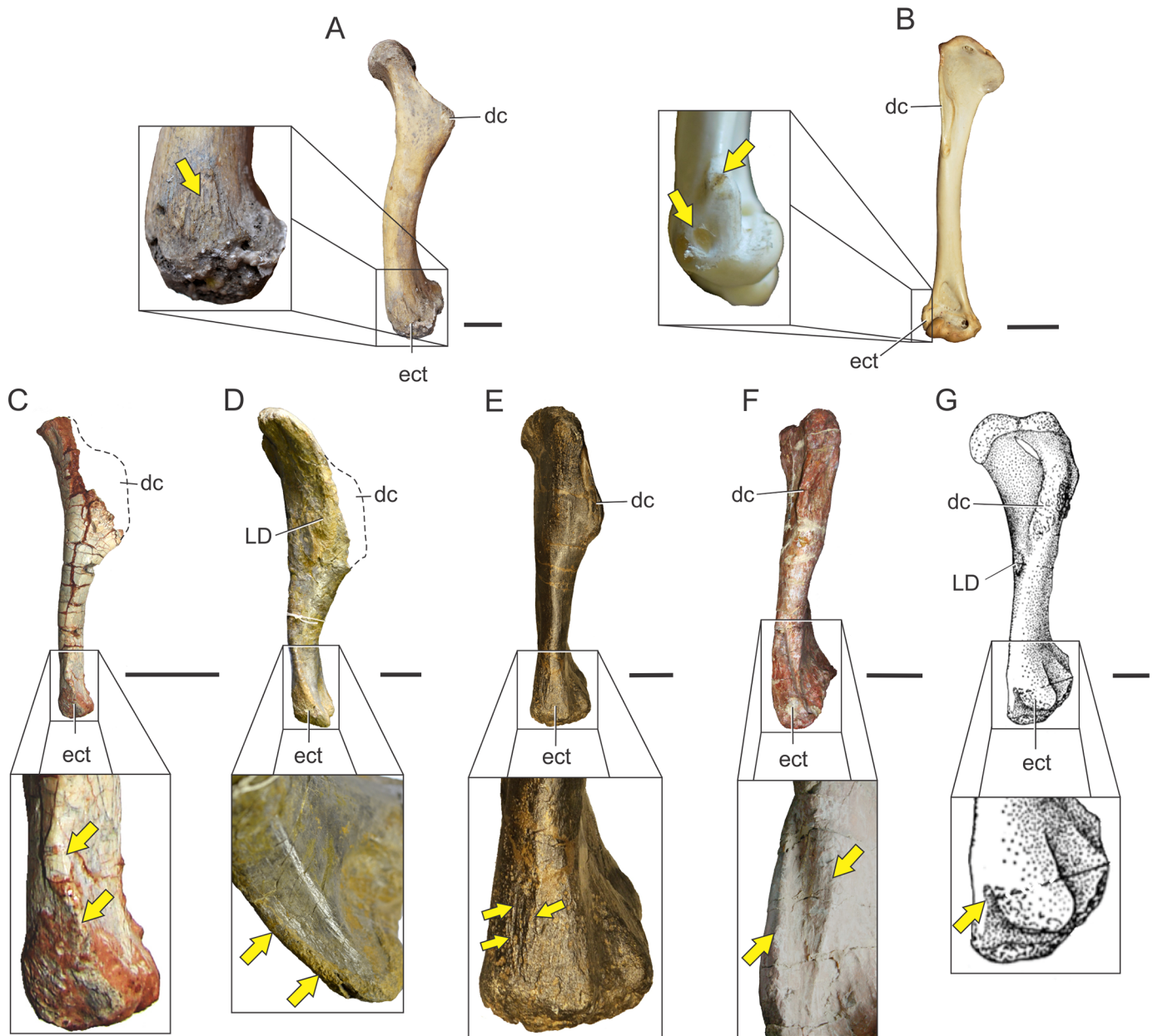
Fig 15. Osteological correlates on the distal humerus in living archosaurs and Sauropodomorpha. Origin site (arrow) of antibrachial muscles on the lateral surface of the ectepicondyle in Crocodylus niloticus (A); Sarcoramphus papa (MLP-O 14362) (B); Saturnalia tupiniquim (MPC 3844-PV)(C); Plateosaurus engelhardti (MB.R. 4404.43 skelett 25)(D); Camarasaurus sp. (AMNH 664)(E); Saltasaurus loricatus (PVL 4017–67)(F); Opisthocoelicaudia skarzynskii (Reprinted from Borsuk-Bialynicka, Fig 7C in [15] under a CC BY license, with permission from Instytut Paleobiologii PAN, original copyright)(G). Abbreviations: ect, ectepicondyle; dc, deltopectoral crest; LD, M. latissimus dorsi insertion site. Scale bar: 3 cm (A)–(D); 10 cm (E)–(G).
