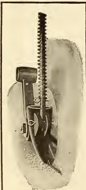
Illustrating one of the revolving discs cutting a narrow gash in the sod and the boot sowing the seed immediately behind the gash which is then closed by the roller following.
