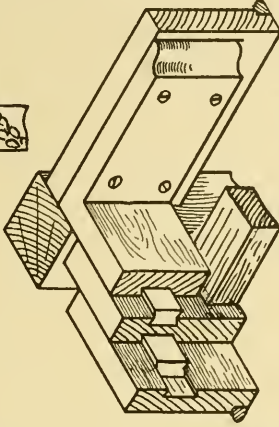
DETAIL OF SLIDES AND FRAMING AT B.
