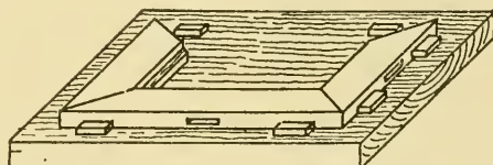
3. Fitting up the Centre Part.
