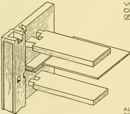
ISOMETRIC VIEW SHOWING CONSTRUCTION AT LEFT HAND CORNER OF FRAME
