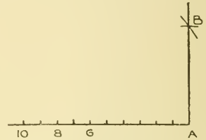
2. Method of Striking a "Square" Line.
