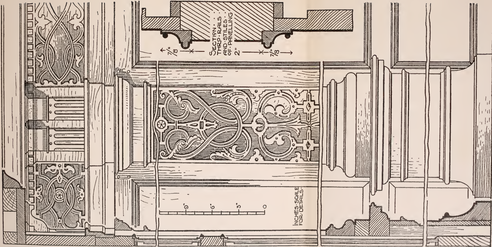
VIEW SHOWING PROPORTION OF PANEL - LING AND ARRANGEMENT OF BRACKET CORNICE IN JACOBEEAN ROOM. V & A. MUSEUM. DATE. CIRCA. 1696 INCHES.
