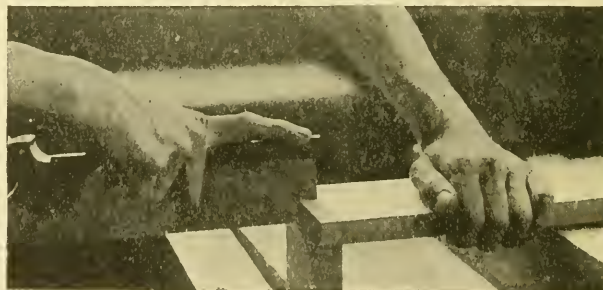
5. Marking Dovetails with Saw.
