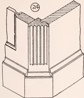
SPLAYED CORNER IN CARCASS WORK . . . .
