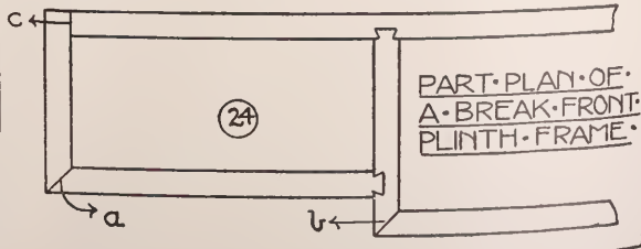
PART PLAN OF A BREAK FRONT PLINTH FRAME...
