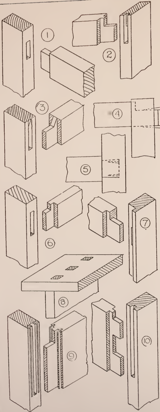
CORNER-TABLE- OF-A-FRAME
