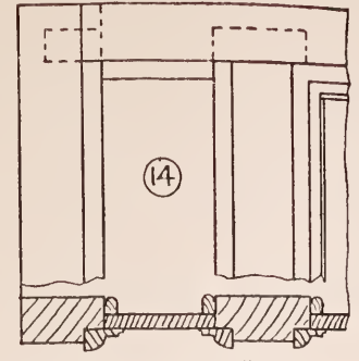
REBATED-FRAMING WITH-PLANTED-MOLDG
