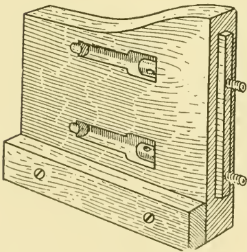
Connection of Rails at Ends.
