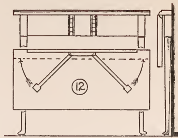
A FOLDING HALL TABLE WITH LEGS ON FLY RAILS...
