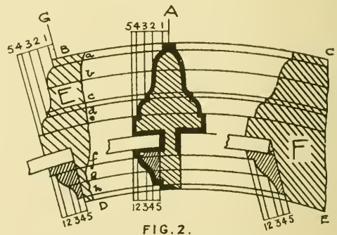
FIG. 2. Showing Method of Intersection for Mouldings on Curved Bars.
