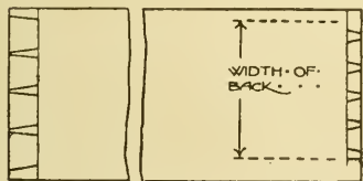
2. Drawer Side Dovetails.
