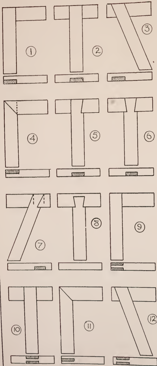
METHOD OF FIXING TILES IN BACK OF WASHSTAND...
