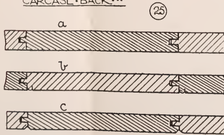
SECTIONS OF MATCHED BACKS . . .
