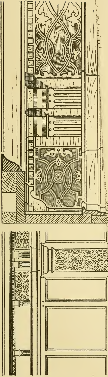
PANELLING AND DETAILS OF JACOBEAN DOORS
