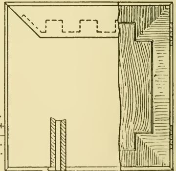
ALTERNATIVE CONSTRUCTION IN DOOR LAMINATING AND CLAMPING
