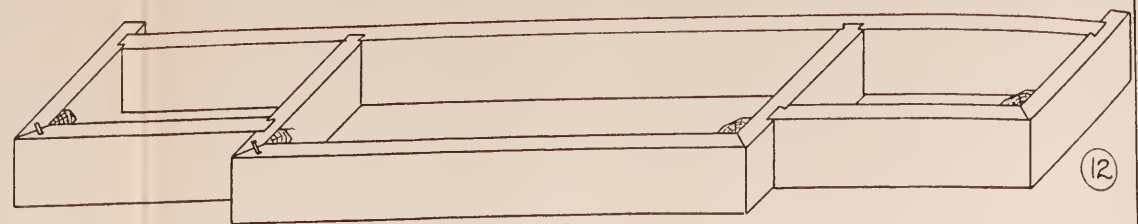
A. PLINTH FRAME SHEWING APPLICATION OF BLOCKED AND TONGUED MITRE JOINTS...
