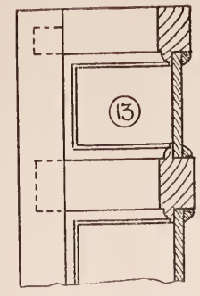
FOX-WEDGED TENONED-DOOR
