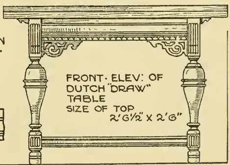
DETAILS ENLARGED
