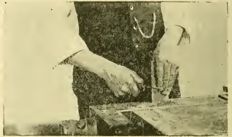
2. Vertical Sharpening of Scraper.
