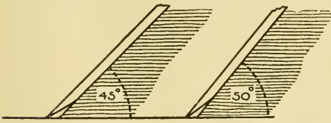
1. Angles of Trying and Smoothing Planes.
