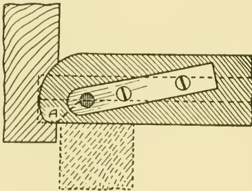
4. Method of Finding Centre and Fixing Centre Hinge.
