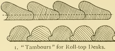
1. "Tambours" for Roll-top Desks.
