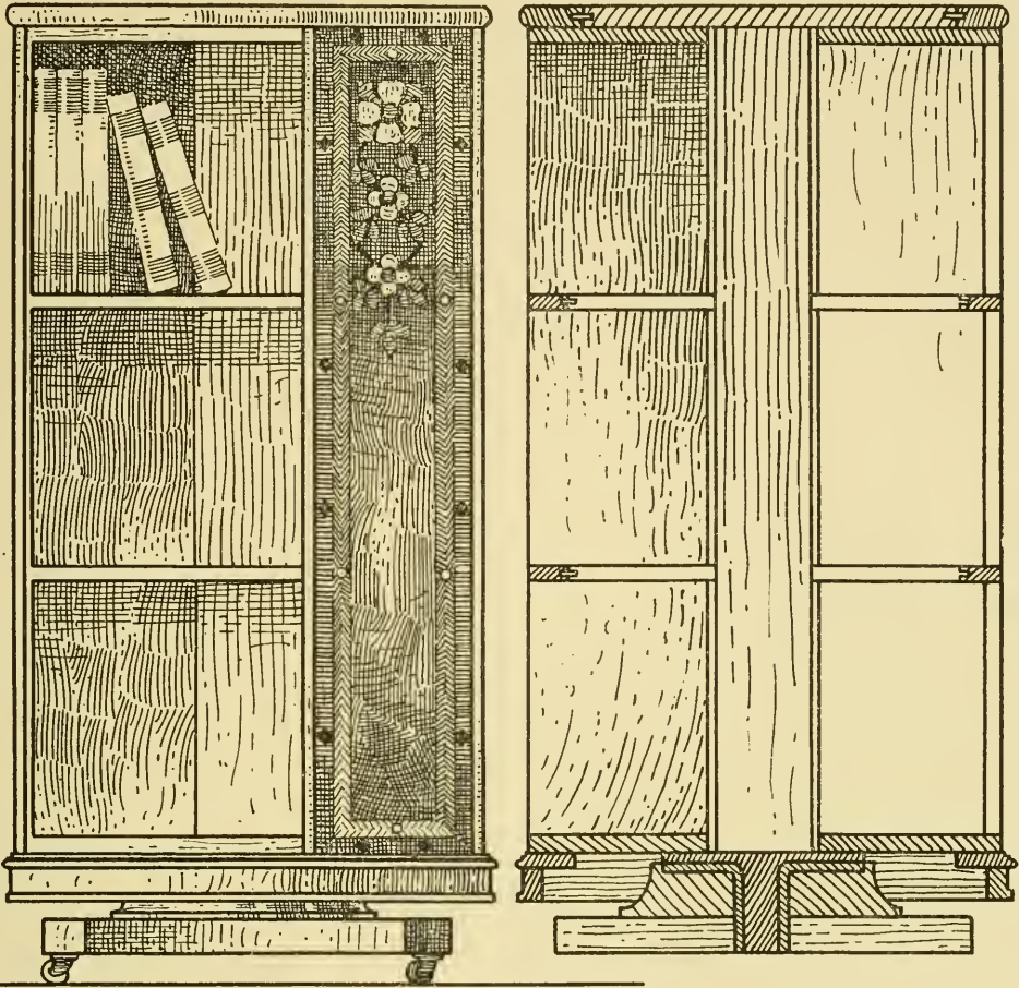
SECTIONAL VIEW ON LINE X-X
