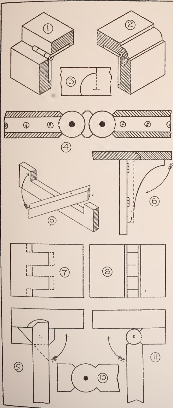
A FOLDING HALL TABLE WITH LEGS ON FLY RAILS...
