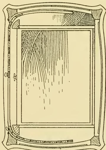
SECTIONAL PLAN • THRO' TAMBOUR •
