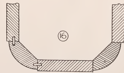
JOINTING IN COMMODES AND PILLARS...
