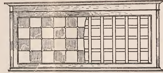
METHOD OF FIXING TILES IN BACK OF WASHSTAND...
