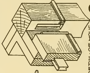
DETAIL OF SLIDES AND FRAMING AT B.
