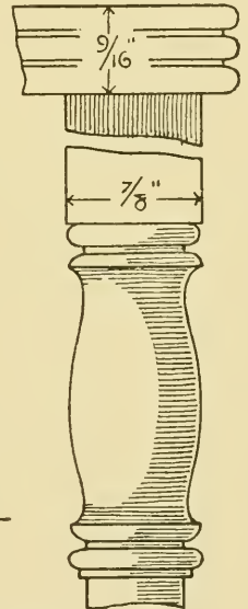
SECTION..
