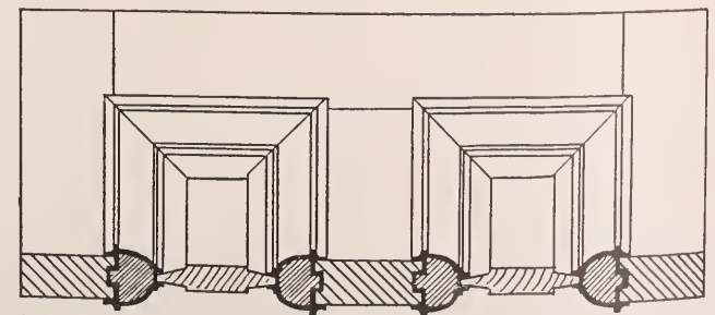
DOOR WITH MOULDINGS MITRED AND TONGUED...
