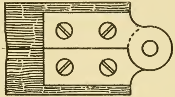
METHOD OF FIXING TOP PIN PLATES EXACT SIZE . .
