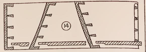
LAPPED AND BEVELLED LAPPED DOVETAILED APPLIED TO DRAWER FRONTS...
