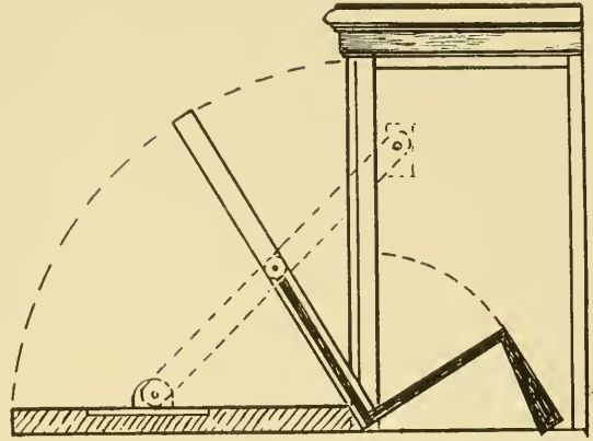
1. Method of Supporting Heavy Flaps.
