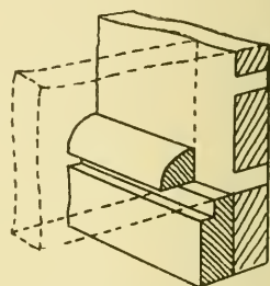
2. Fitting a Drawer Slip.
