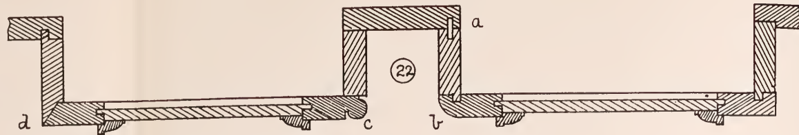
VARIOUS METHODS OF CONNECTING ANGLES OF PANELLING . . . .
