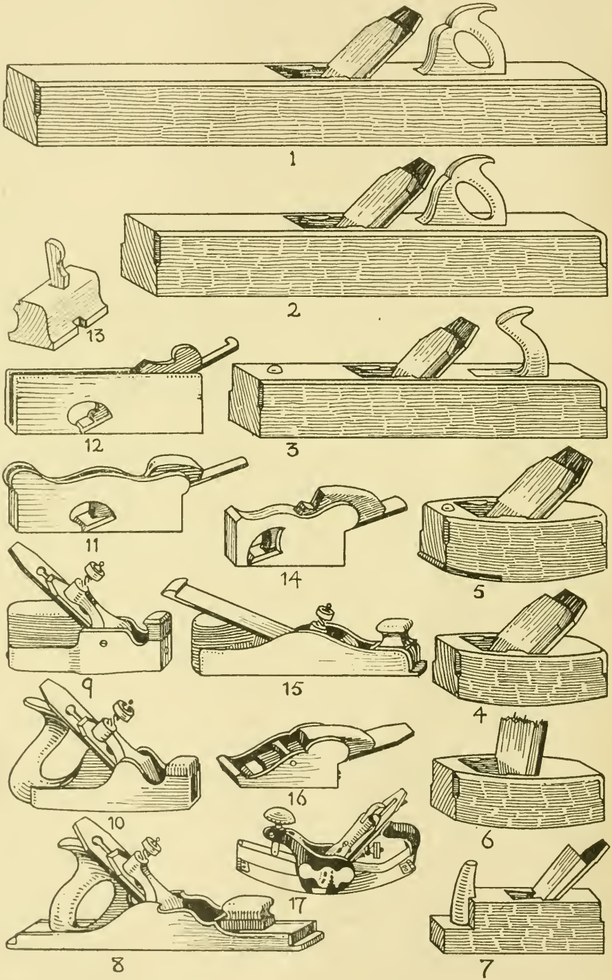
VARIOUS PLANES.
