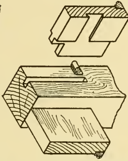
JOINT AT A.
