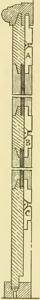
Section of the Mansfield-Robinson Patent Panelling.
