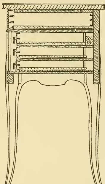
SECTIONAL VIEW —
