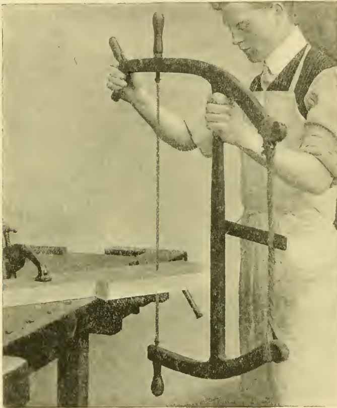
Cutting Sweep on Bench.
