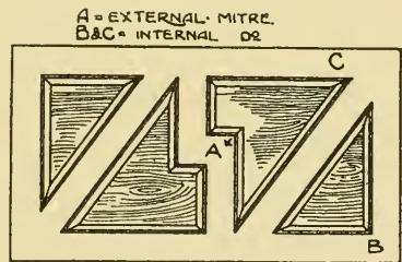
3. Diagram showing Various Mitres.
