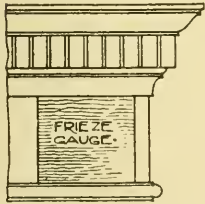
2. Use of Margin Gauge.
