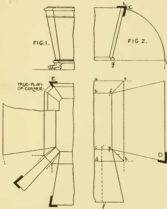
Views showing Method of Projecting Developments.
