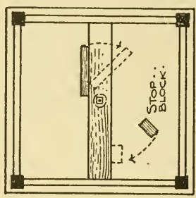
VIEW SHEWING POSITION OF SPRING AND STOP..
