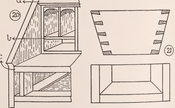
HOUSED DOVETAILED IN CARCASE WORK... ELEVATION AND HALF PLAN OF A HOPPER...
