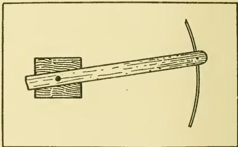
2. Router for Curved Lines.
