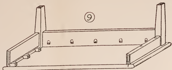
DIAGRAM SHEWING METHODS OF FIXING TABLE TOPS ...
