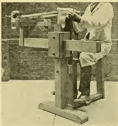
Using a Marquetry Cutter's "Donkey."
