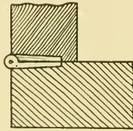
3. Butt Hinge fixed on to Carcase End.
