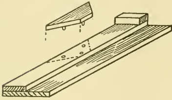
1. A "Mitre" Shooting Board Attachment.
