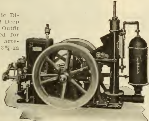
DIRECT CONNECTED DEEP WELL PUMPING ENGINE
