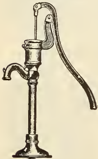
Fig. 41. No. 392. —Lift Pump, for wells up to 25 feet; can be extended to 40 feet; adjustable base and brace; iron Cylinder, 3 inches. Fitted for 1 1/4-inch pipe. Pump extends 4 feet below platform, will fit in a 5-inch cased well. Price, List, $6.75; Retail, $4.50.
