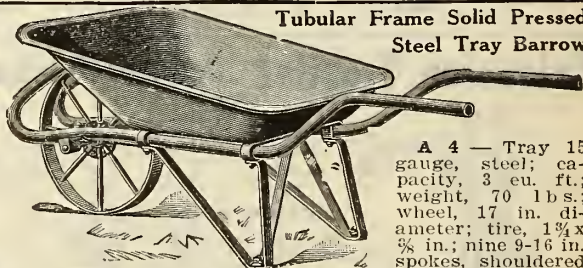
Southern Steel Tray Barrow
