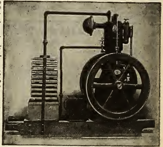
3 H. P. VICTOR ENGINE WITH PAN COOLER.
