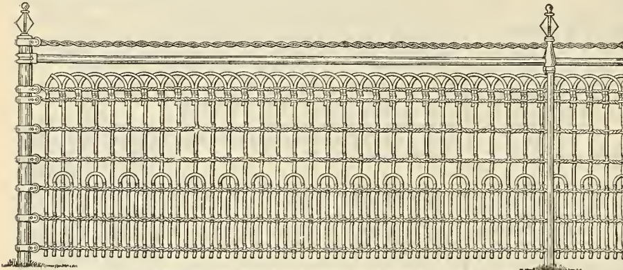
STYLE C FENCE ON STEEL POSTS WITH BRAIDED TOP.
