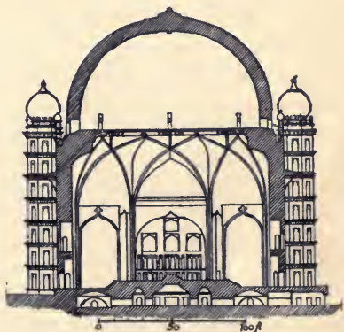
FIG. 85.—TOMB OF MAHMUD, BIJAPUR. SECTION.
