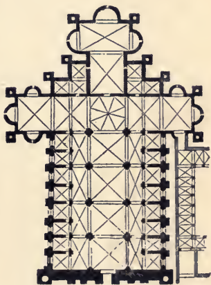
FIG. 153.—PLAN OF CERTOSA AT PAVIA.
