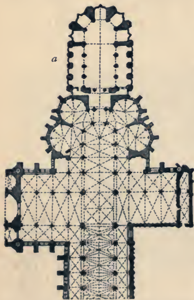
FIG. 137.—EASTERN HALF OF WESTMINSTER ABBEY. PLAN.
