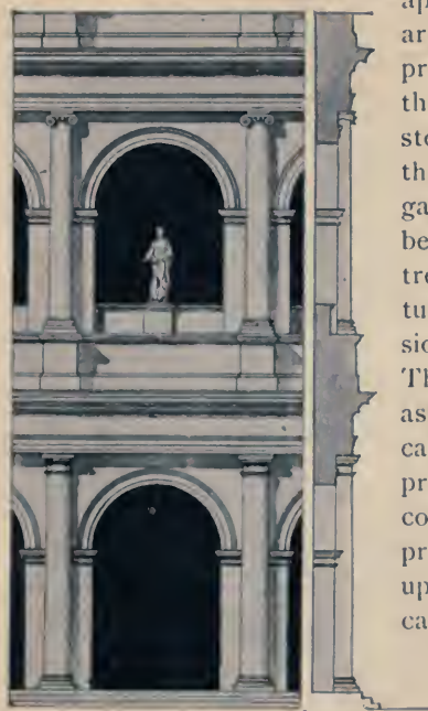
FIG. 45.—ROMAN ARCADE WITH ENGAGED COLUMNS.
