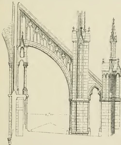
FIG. u.—FLYING BUTTRESS.
