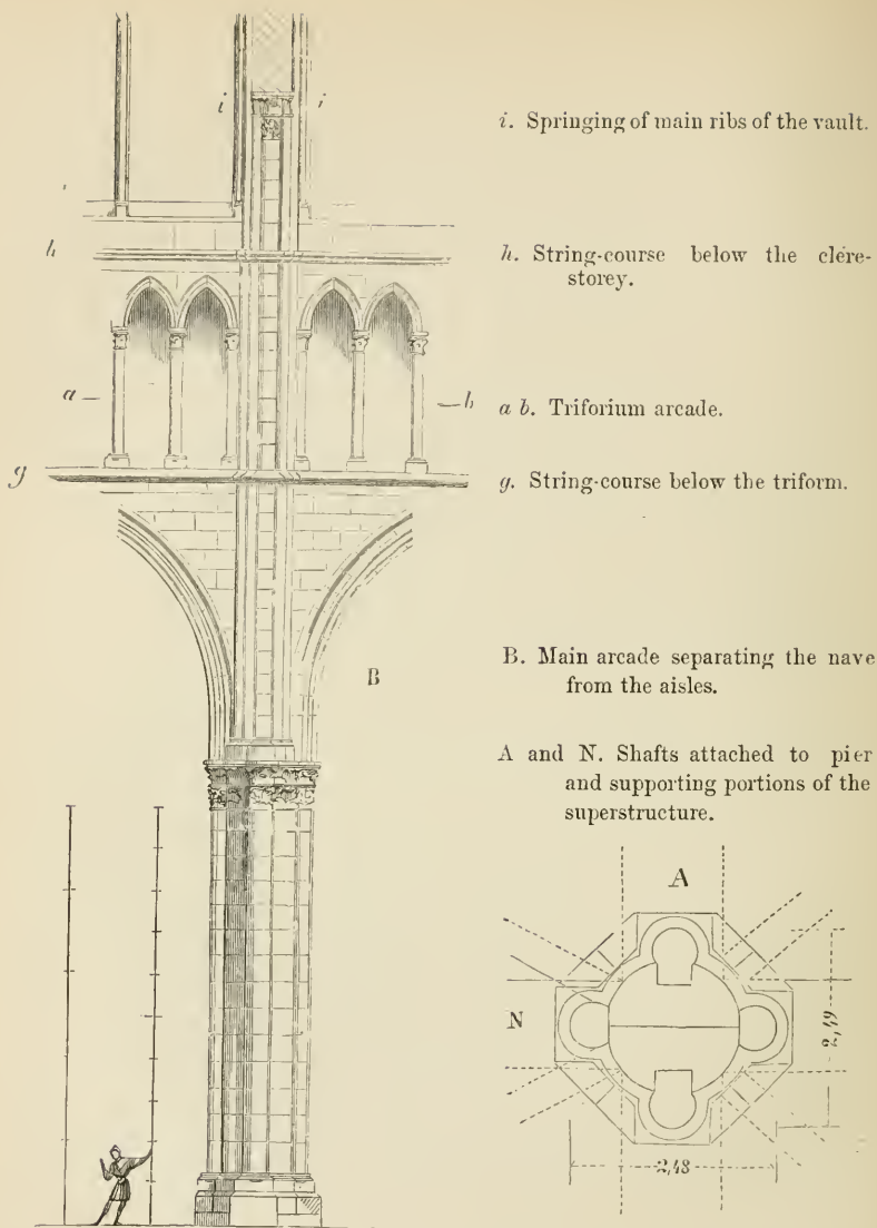
FIG. 36.—PIERS AND SUPERSTRUCTURE, RHEIMS CATHEDRAL. (1211-1240.)
