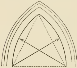
FIG. c.—EQUILATERAL ARCH.
