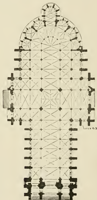
FIG. 34.—PLAN OF AMIENS CATHEDRAL. (1220-1272.)
