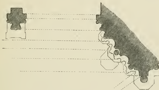
FIG. 2.—PLAN OF A JAMB AND CENTRAL PIER OF A GOTHIC DOORWAY.
