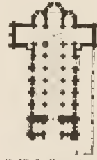
Fig. 115. San Vincente in Avila, erb. c. 1260.
