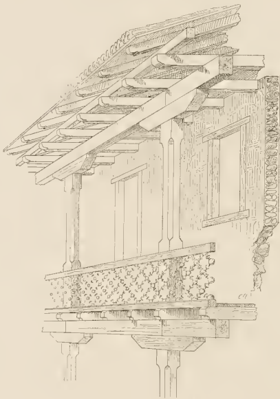
Fig. 53. Gallerie in Holz constr. dirt.
