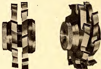
ADJUSTABLE COPE HEADS 8" DIA. #2-200 5" DIA. #2-167
