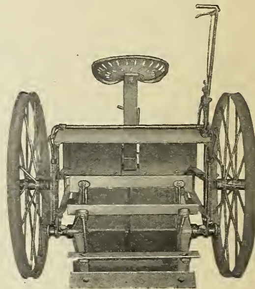
Oliver 9 Blade Stalk Cutter
