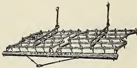
CLOSED END LEVER HARROW
