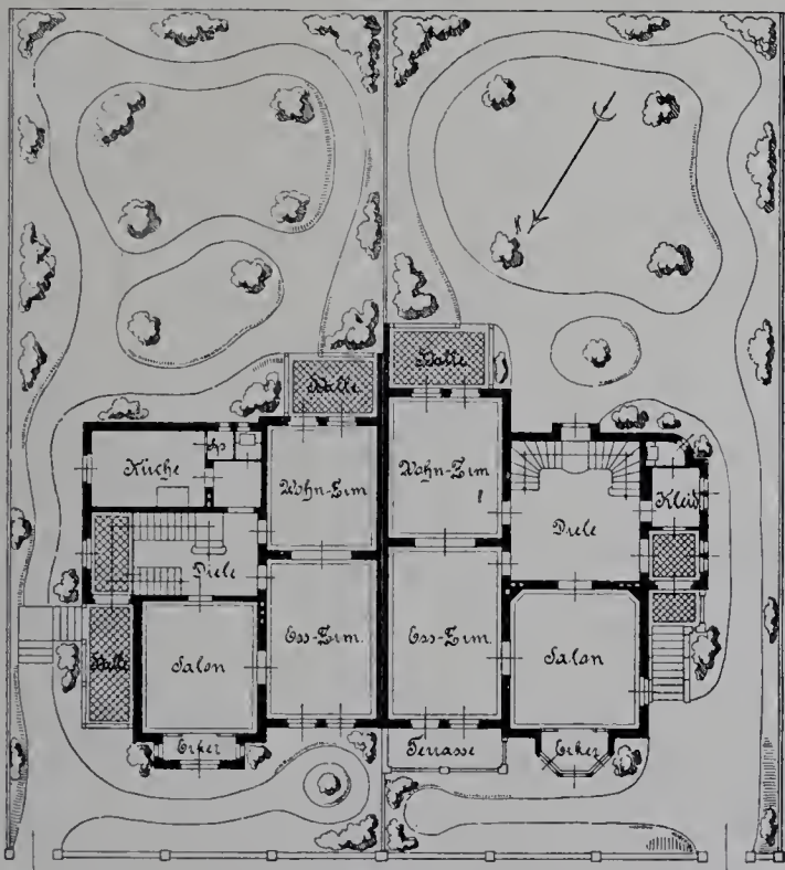
Erdgeschoss.
