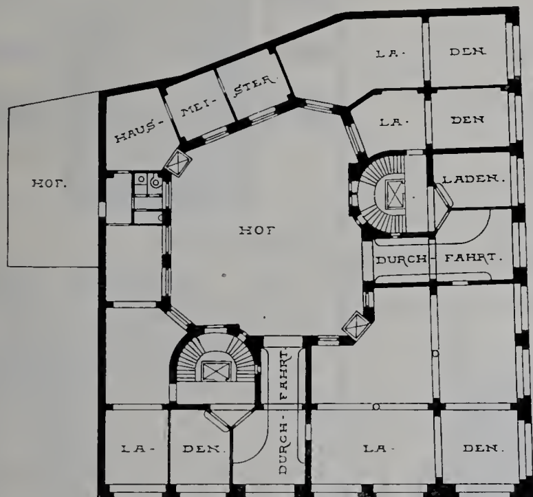
Erdgeschoss.
