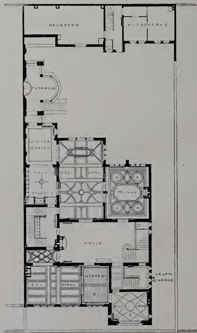
Erdgeschoss.
