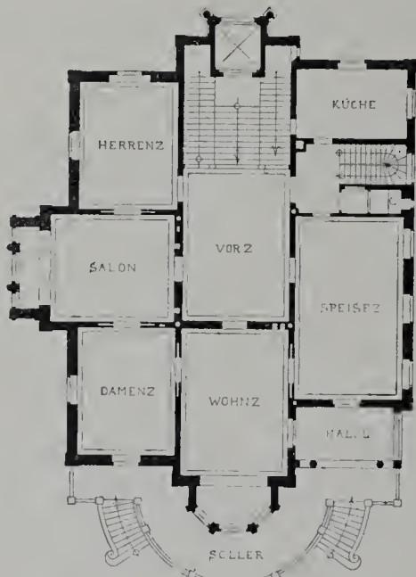
Erdgeschoss.
