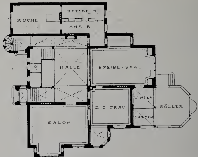
Erdgeschoss.
