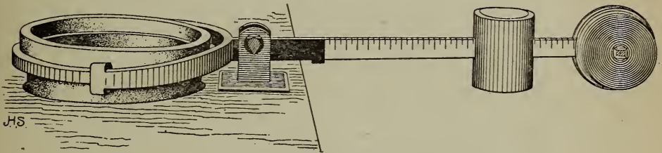
FIG. 1.—Balance for weighing soil pots.
