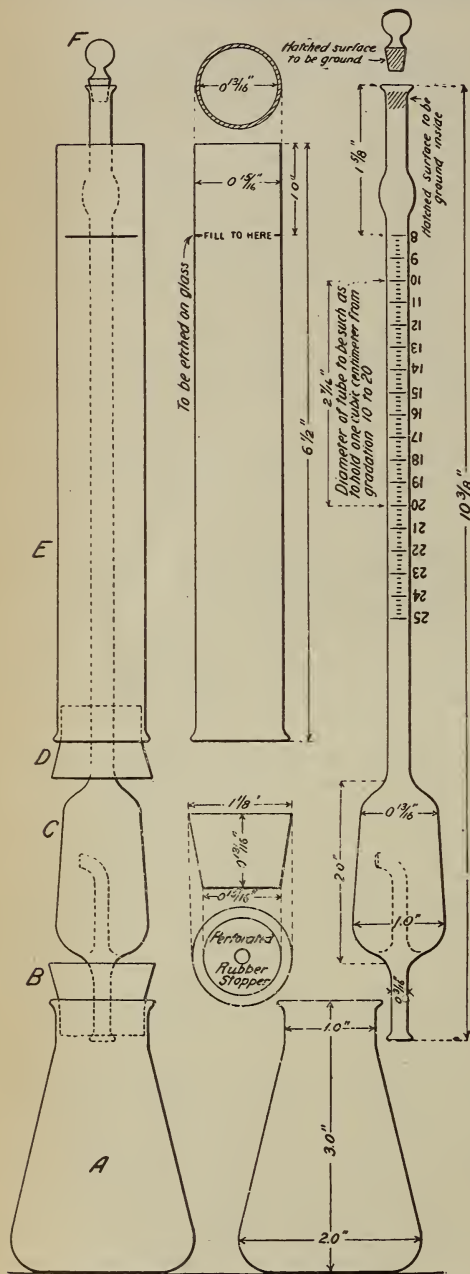
FIG. 1.—Apparatus for moisture determination.
