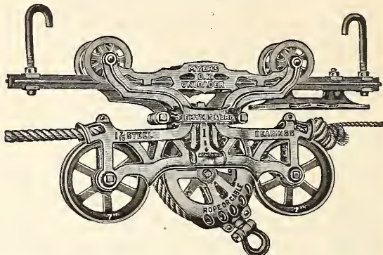
Myers' Double Lock Unloaders.
