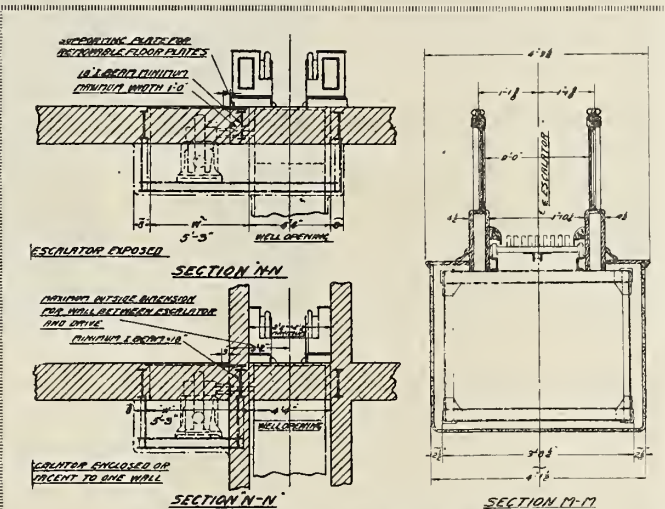
DETAILS OF THE OTIS THEATRE ESCALATOR
