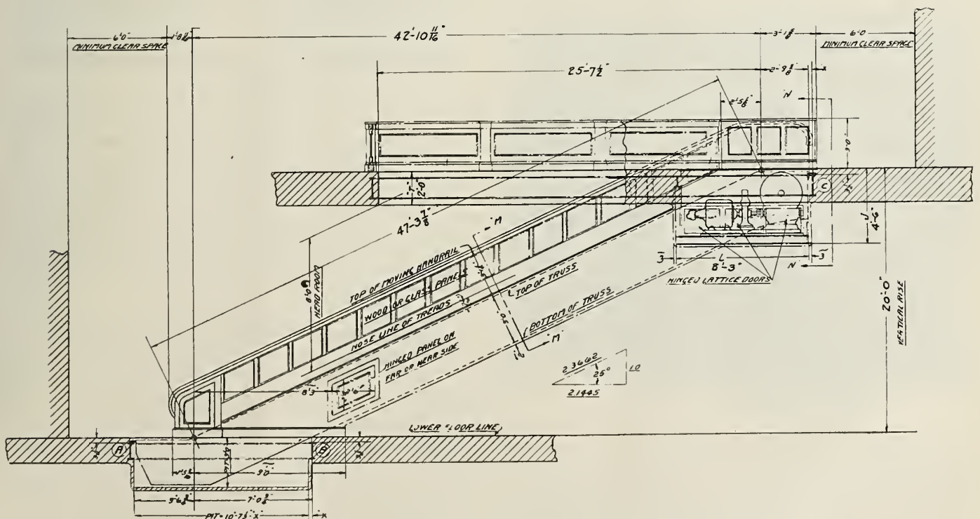
SECTION K-K
