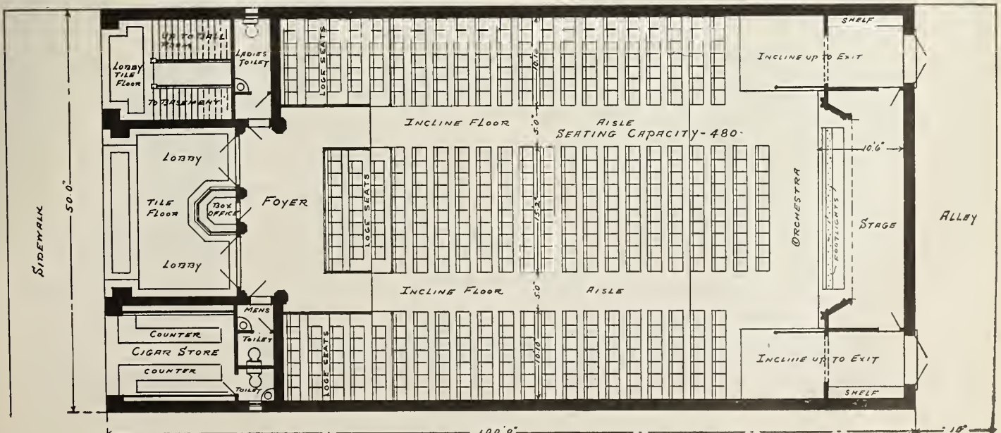
GROUND FLOOR PLAN OF THE GLOBE THEATRE, SAN PEDRO, CAL. (L. B. & A. L. Valk, Los Angeles, Cal., Architects)
