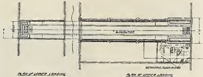
PLAN OF LANDINGS FOR OTIS THEATRE ESCALATORS
