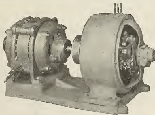
TYPE OF AC TO DC COMPENSARC
