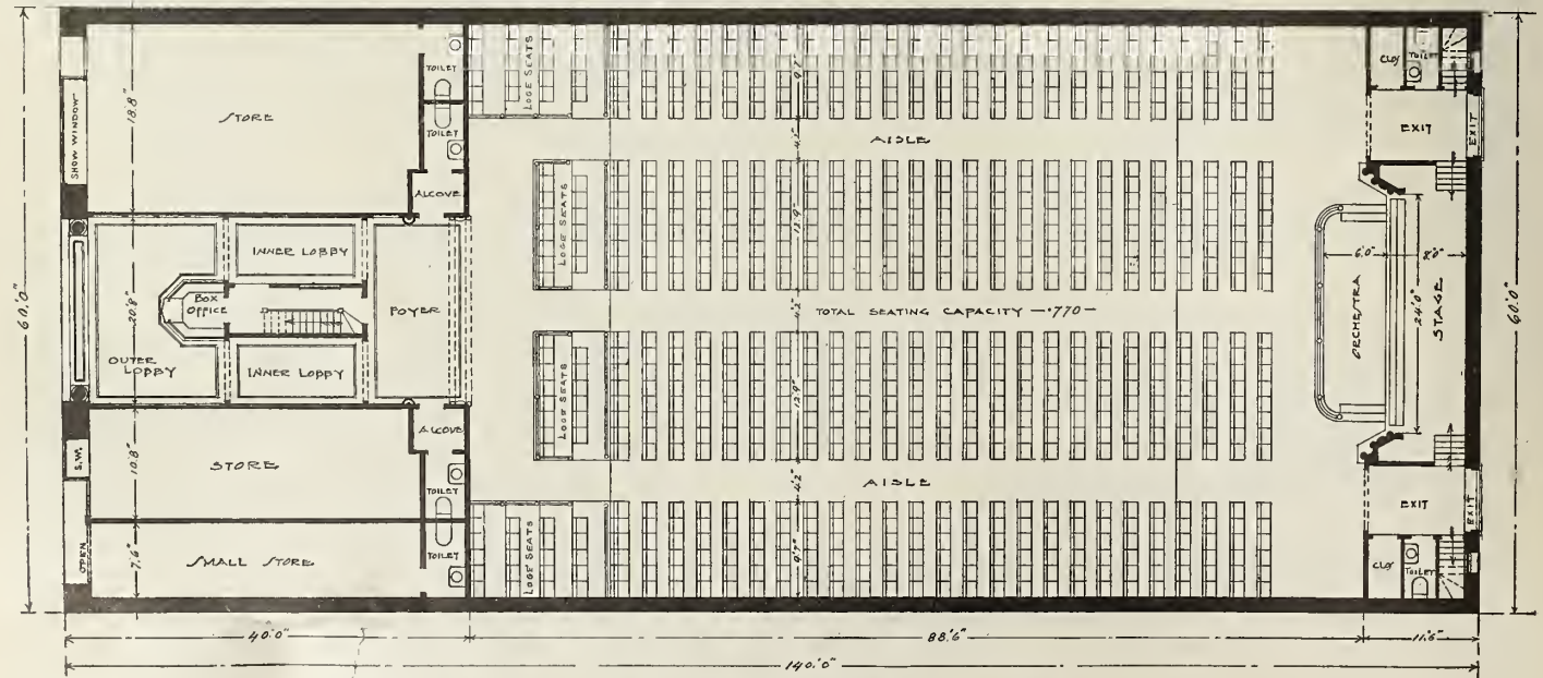
PLAN OF THE MAIN FLOOR, NATIONAL THEATRE, LOS ANGELES, CALIFORNIA.
