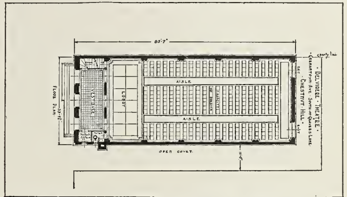
FLOOR PLAN OF THE BELVIDERE THEATRE, CHESTNUT HILL, PHILADELPHIA
