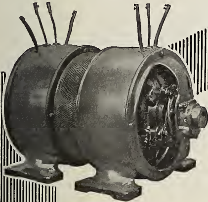
The DC Compensarc lowers the voltage of a direct current supply to that required at the lamp without needless waste.
