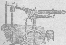
[A simple form of Spectroscope.] p Prism of Flint Glass; a Telescope with Eyepiece; b Collimator through which the Light, which enters at the Slit in the End of the Prism, is sent to form Spectrum; c, passes to the Prism to form Spectrum; d, a Tube with a Micrometer; e Holder for Substrate whose Spectrum is to be examined; f, Flame illuminating Micrometer Scale; g, a Adjusting Screws.
