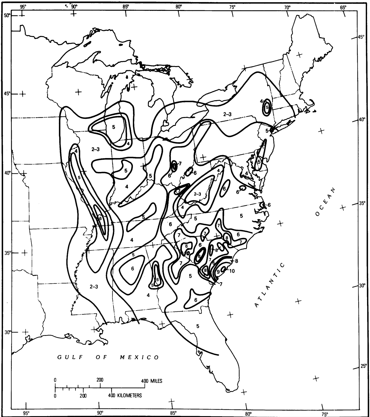
Figure 4. Isoseismal map of the Eastern United States contoured to show the more localized variation in the reported intensities for the 1886 Charleston earthquake. Contoured intensity levels are shown by arabic numerals. (From Bollinger, 1977.)
