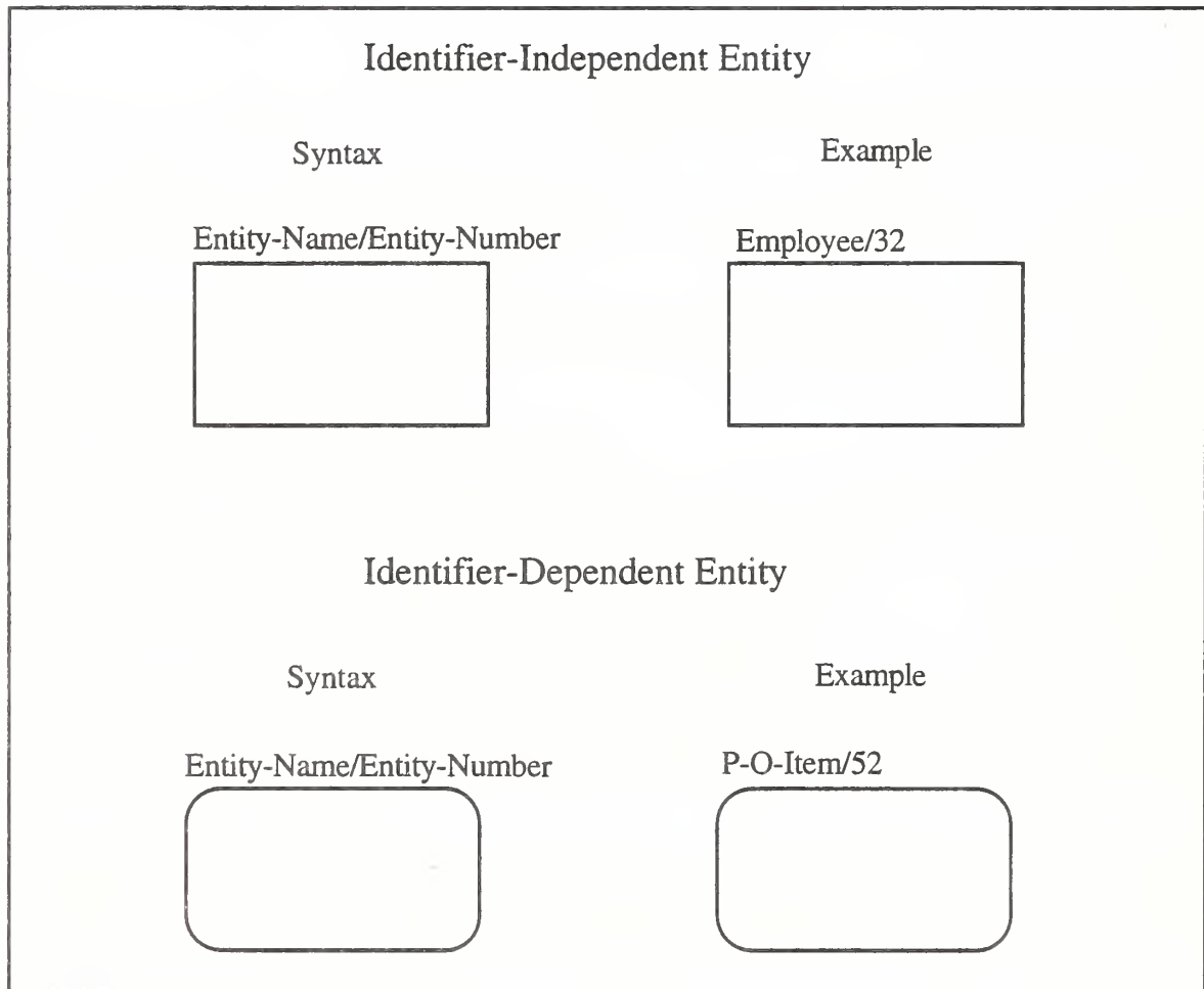
Figure 1. Entity Syntax
